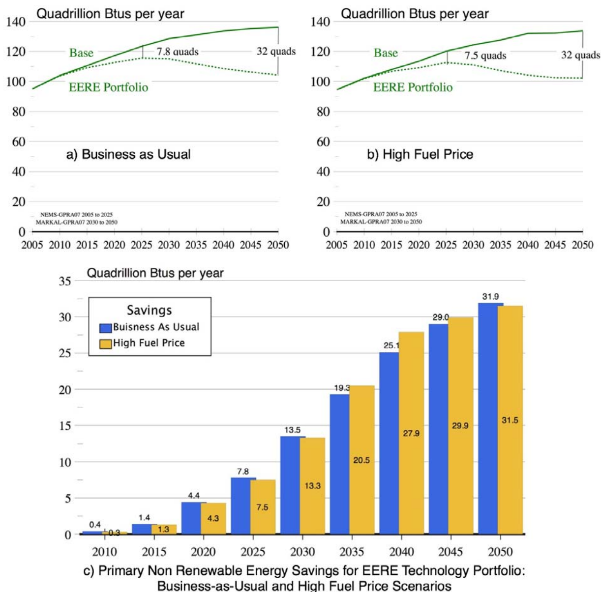
Figure 3. Primary Nonrenewable Energy Use Under Alternative Fuel Price Scenarios
