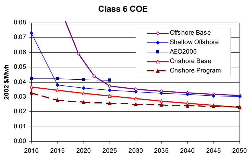
Figure 1. Class 6 Baseline and Program COE Trajectories
