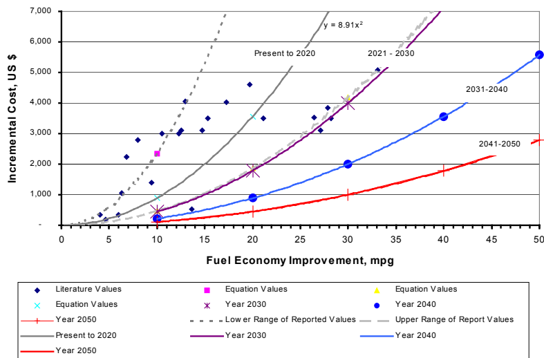
Exhibit 7: Proposed Hybrid-Electric Auto Cost Curves
