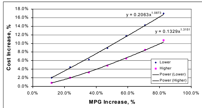
Exhibit 4: Normalized Graphs of NRV Fuel Economy—Cost for Light Trucks
