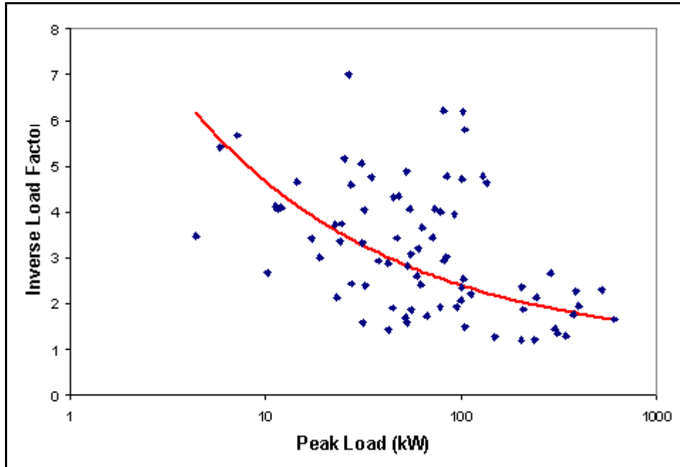
Figure 6.2.2 Scatterplot of Inverse Load Factor versus Peak Load from Hourly ELCAP Data
