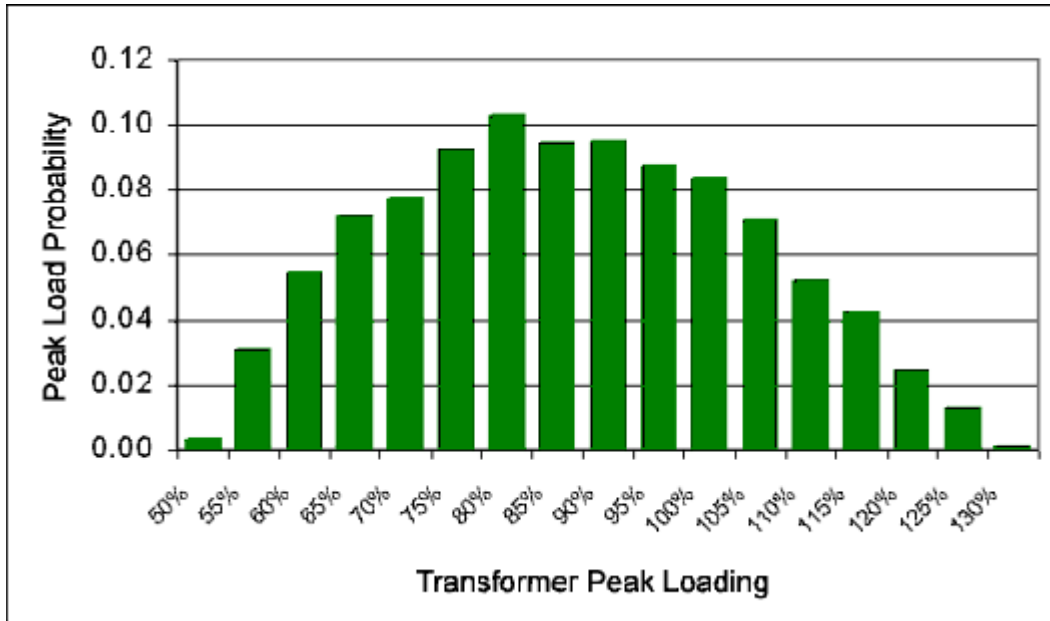
Figure 6.2.1 Histogram of the Peak Loading Distribution Generated in the Hourly Load Analysis
