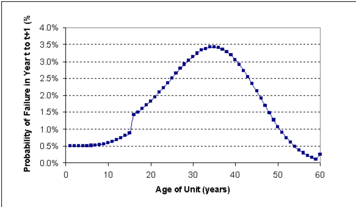
Figure 9.3.2 Fraction of Original Shipment Retiring
