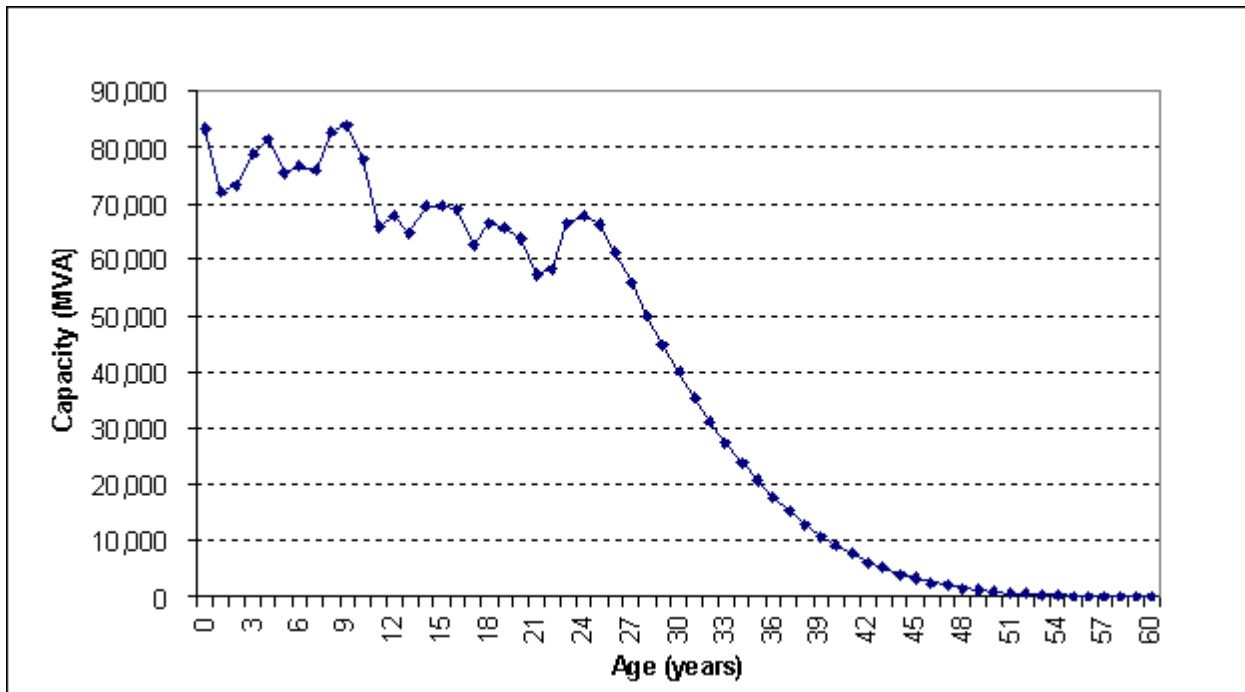
Figure 9.3.1 Age Distribution of Liquid-Immersed In-Service Transformer Stock in 2004
