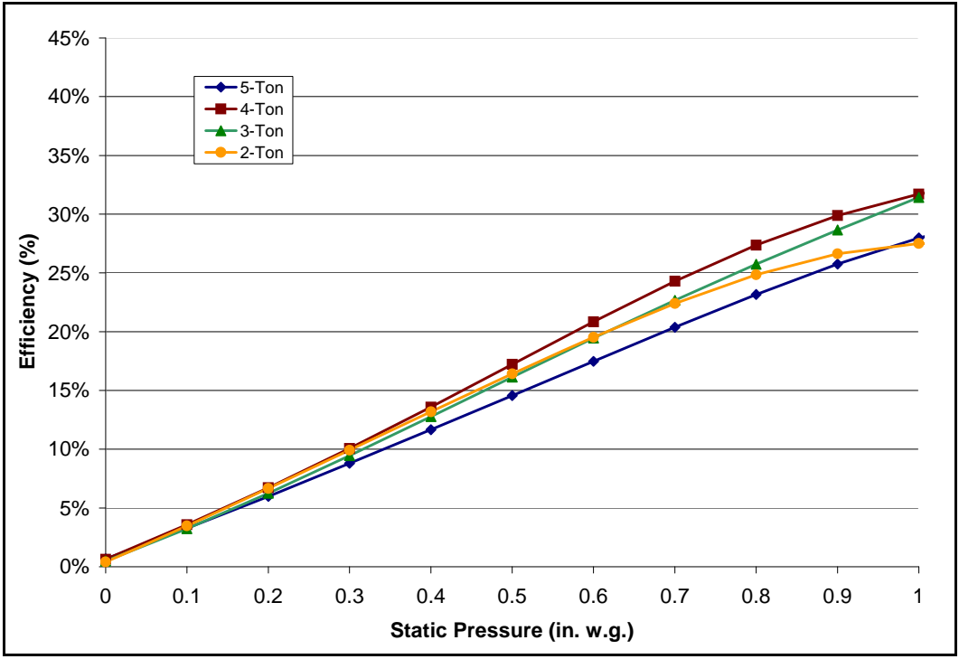
Figure K.3.6 Blower Efficiency vs. Pressure Curves for Condensing Furnace - Single-Stage Control, PSC Motor
