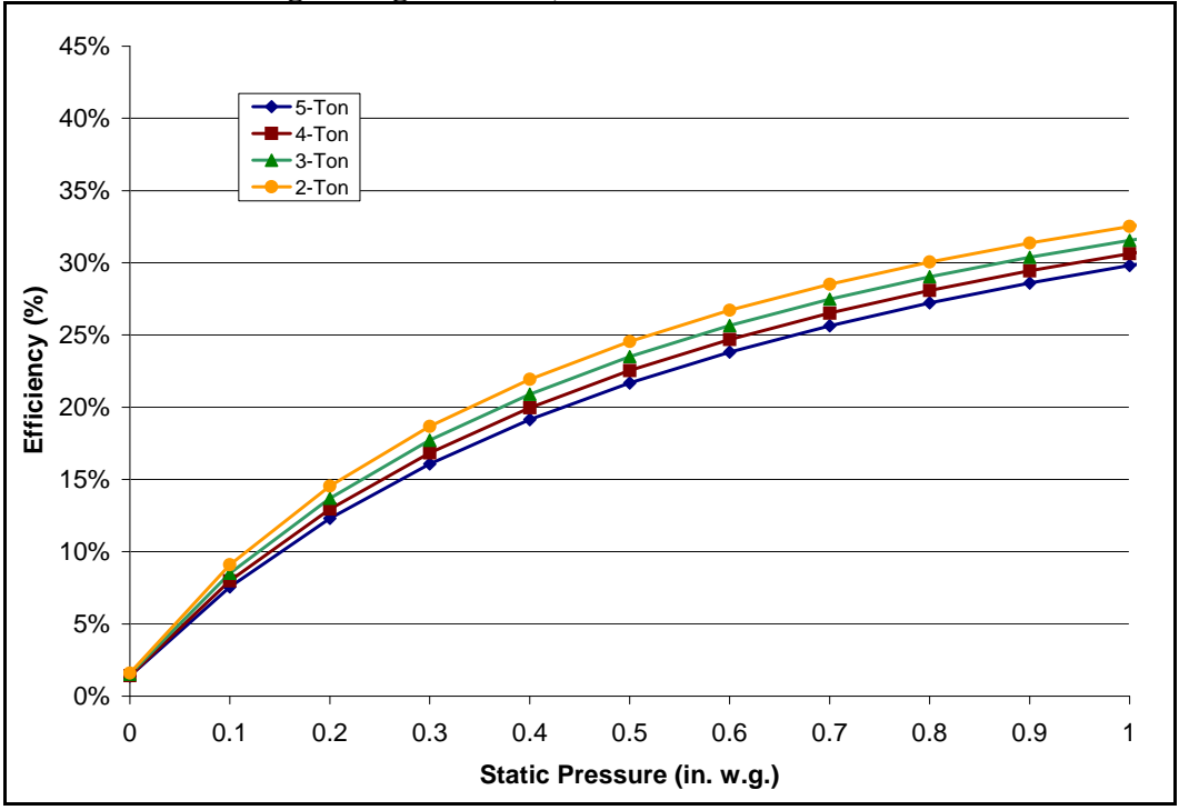
Figure K.3.7 Blower Efficiency vs. Pressure Curves for Non-Condensing Furnace - Two-Stage Virtual Control, ECM Motor, High Fire
