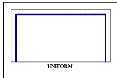
Figure 8A.5.3 Uniform Probability Distribution
