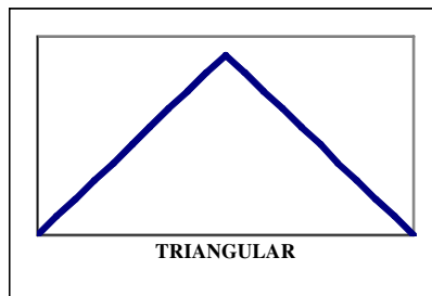
Figure 8A.5.2 Triangular Probability Distribution
