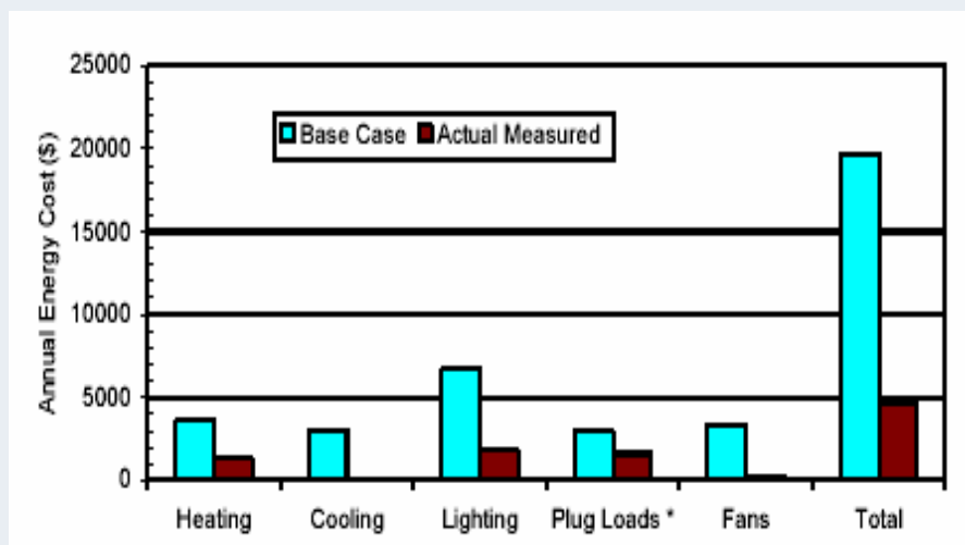
Measured Energy Cost Performance of the Visitors Center (Torcellini et al. 2002)
