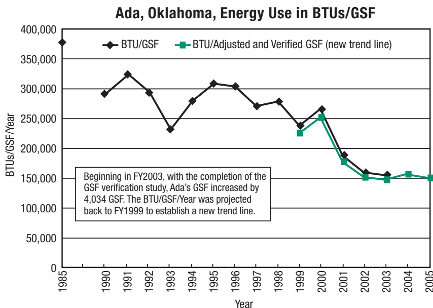
Figure 3. Energy consumption history for the EPA Ada Lab.
