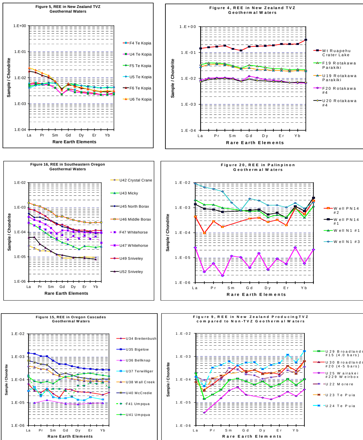
Figure 1. Representative Data Shown in Chondrite Normalized Form
