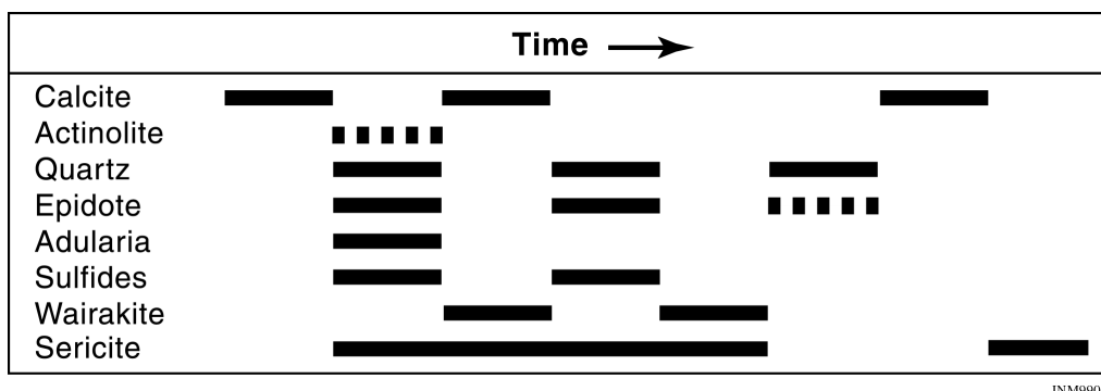
Figure 1. Generalized paragenesis of veins studied in Awibengkok 1-2. Dashed lines indicate that the mineral is present in trace amounts.
