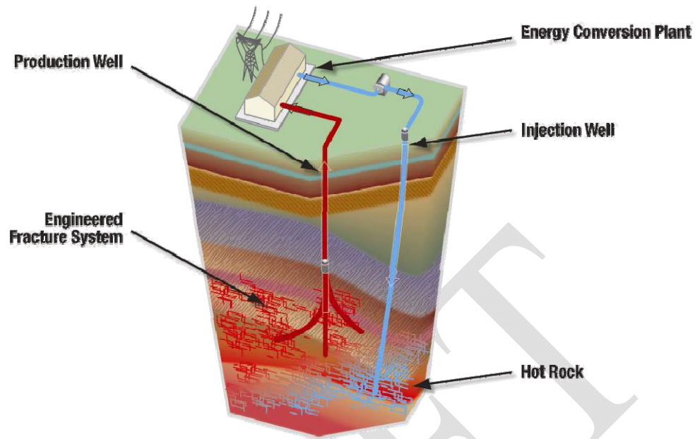
Figure 2. EGS Cutaway Diagram
