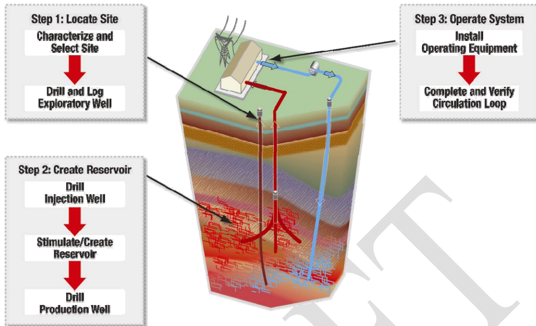
Figure 3. EGS Development Sequence
