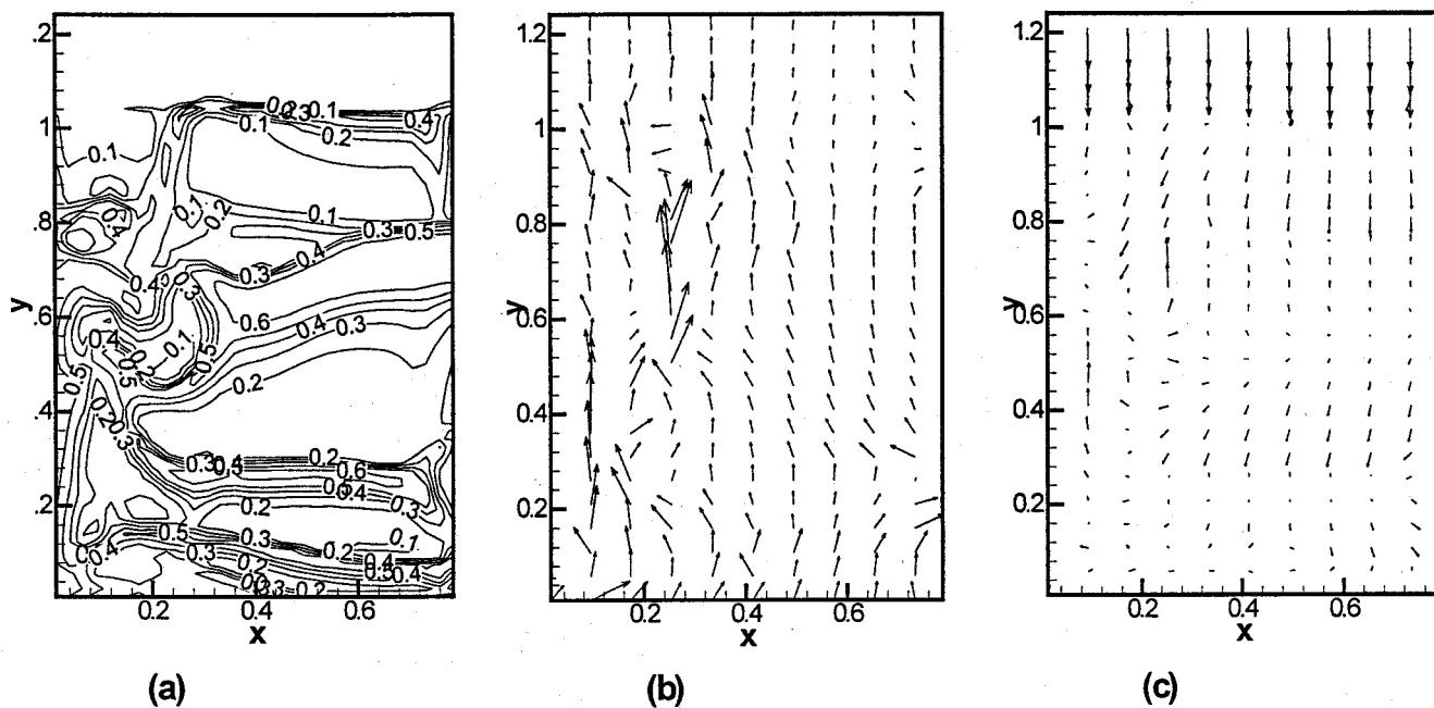
Figure 3: Contours of the solids volume fraction (a), velocity vectors of the gas phase (b) and of the solids phase (c) at 1.2 s. after startup.
