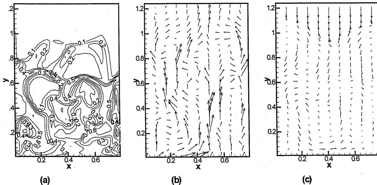
Figure 4: Contours of the solids volume fraction (a), velocity vectors of the gas phase (b) and of the solid phase (c) at 1.8 s. after startup.
