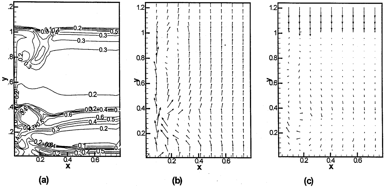
Figure 2: Contours of the solids volume fraction (a), velocity vectors of the gas phase (b) and of the solid phase (c) at 0.8 s. after startup.
