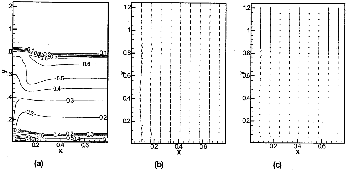
Figure 1: Contours of the solids volume fraction (a), velocity vectors of the gas phase (b) and of the solid phase (c) at 0.4 s. after startup.
