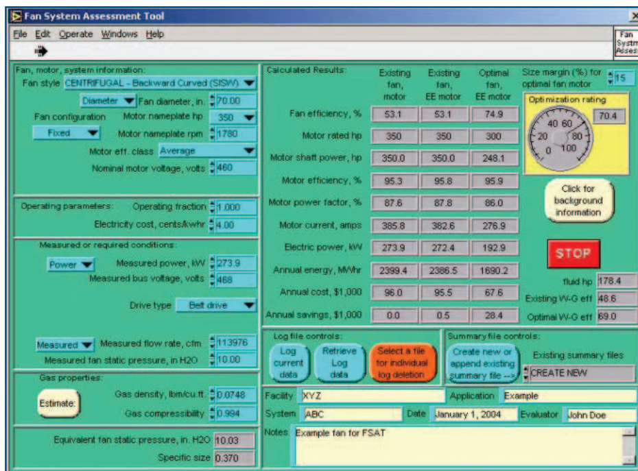
Figure 1: FSAT image showing the tool's main data input screen.
