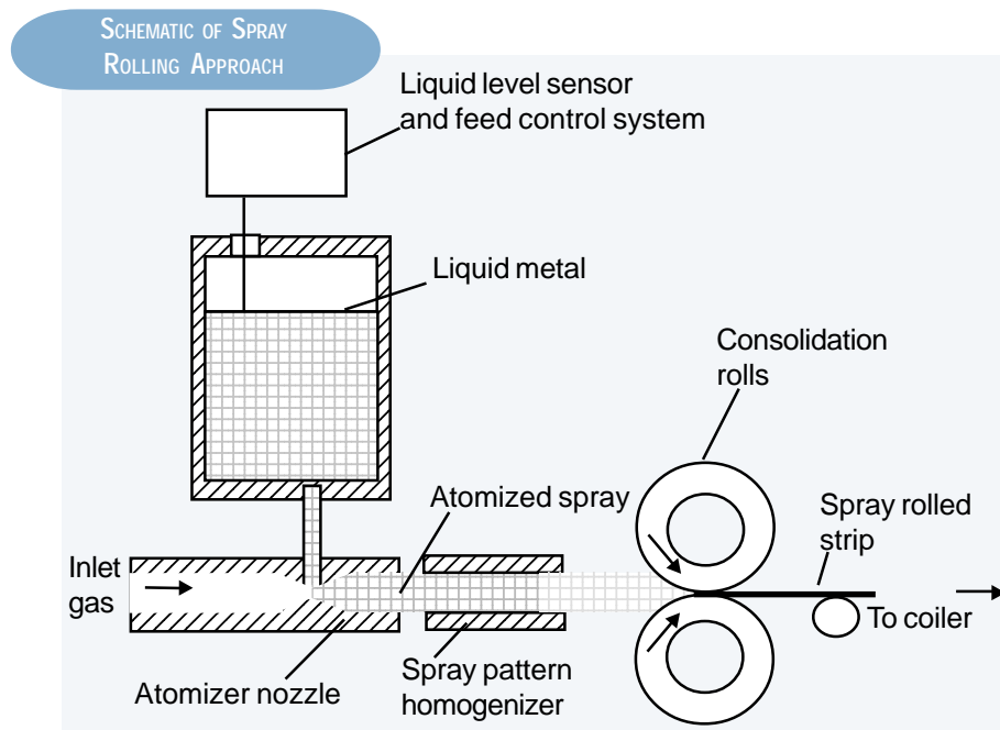
Schematic of the spray rolling approach for manufacturing ferrous and non-ferrous alloy shapes.
