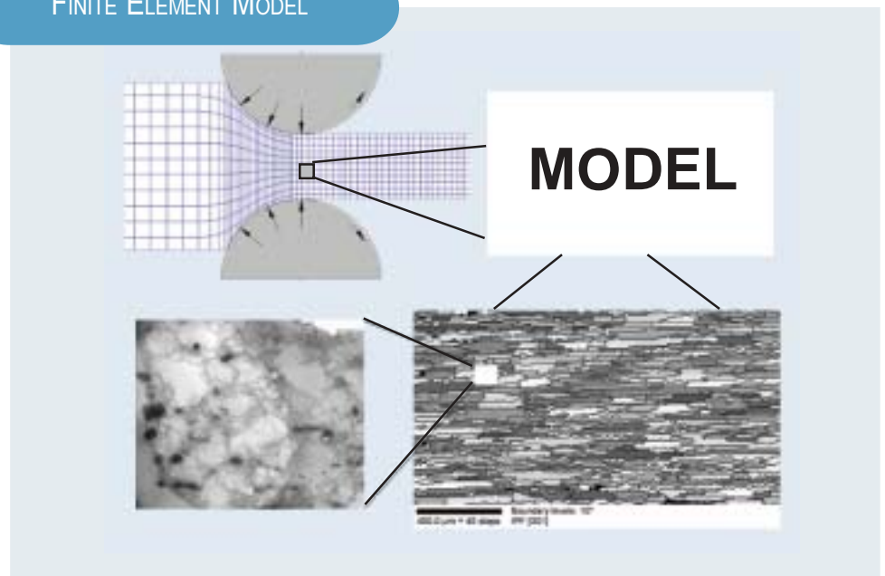
Finite element-based model for thermomechanical deformation and microstructure formation.
