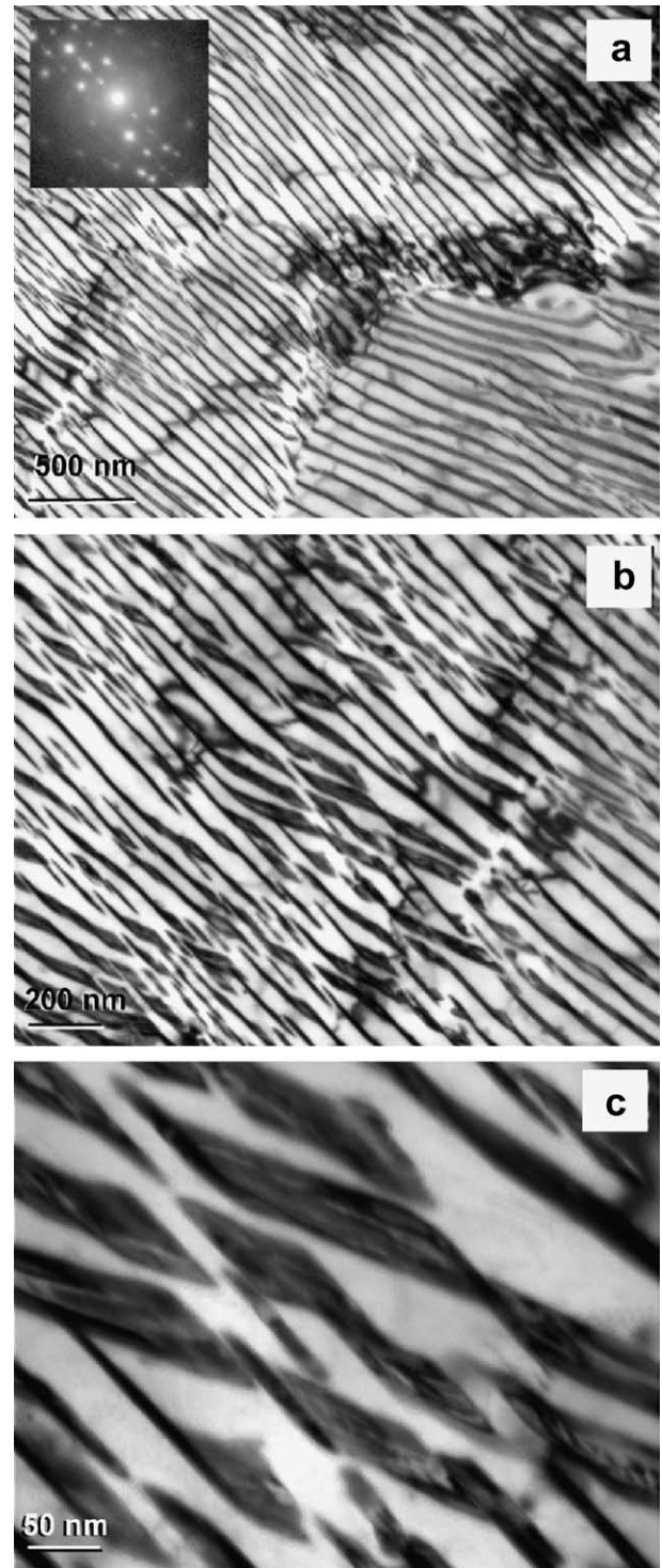
Fig. 3. Transmission electron microscopy images of samples subjected to 30 T magnetic field: (a) Low-magnification picture showing pearlite colonies with inset diffraction pattern obtained from the same area. High magnification micrographs show (b) the cementite lamellae and (c) fine substructure and morphology of carbides.
