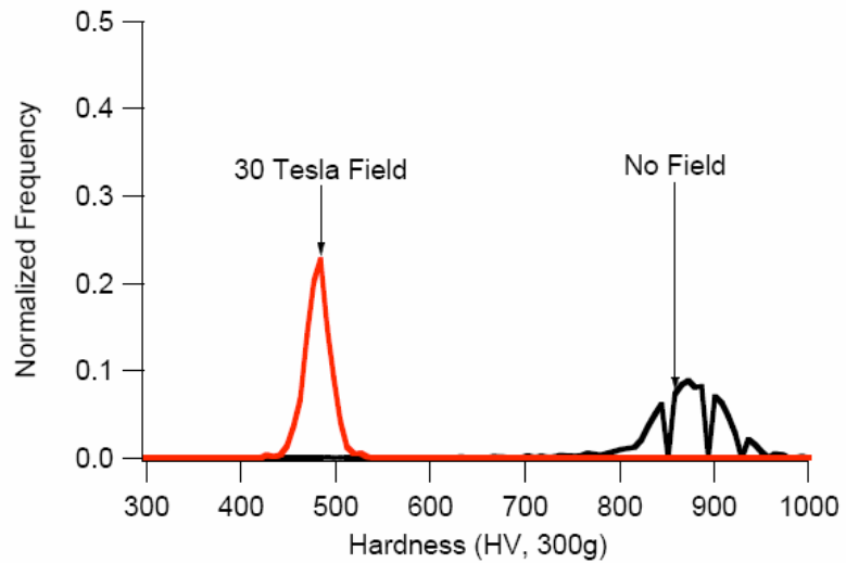
Fig. 4.23. Supporting hardness distribution data for the slow-cooled (1°C/s) high-strength bainitic steel for both the “no-field” and 30-T field magnetic processing conditions.
