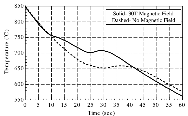
Fig. 2. Cooling curves for cooling at 10 °C/s. Specimen held at 850 °C for 5 min prior to cooling.
