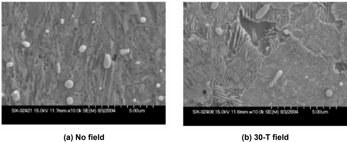
Fig. 4.10. Microstructure of a 52100 alloy subjected to continuous cooling at a rate that would result in martensite formation, with and without application of a magnetic field. Sample (a) shows martensite and remnant carbide; the application of a magnetic field during cooling resulted in the complete transformation to carbide plus pearlite in sample (b).
