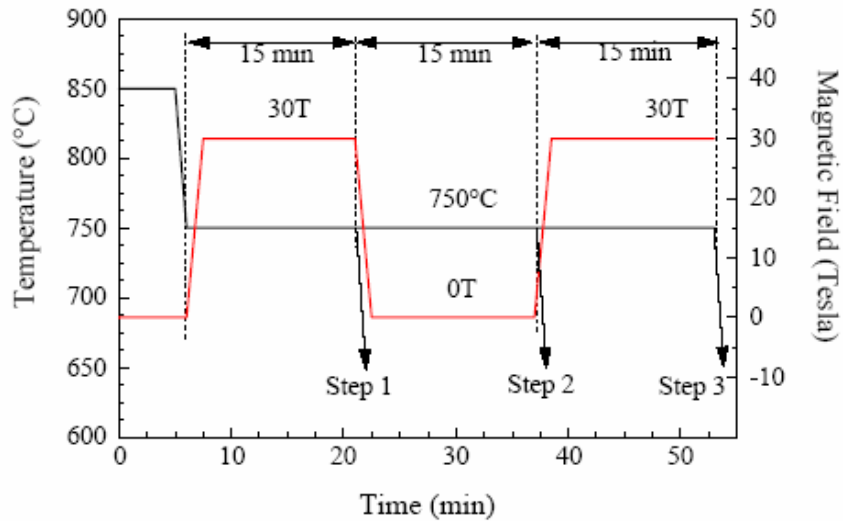
Fig. 4.19. Schematic of an isothermal magnetic field cycling process showing the magnetic field cycling (0 T → 30 T → 0 T) to achieve austenite decomposition and reversal back to the parent austenite, followed by a second decomposition cycle.
