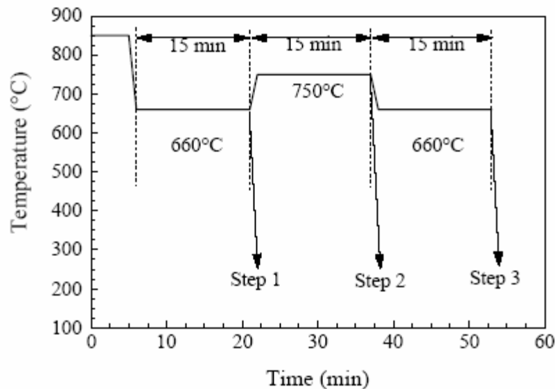
Fig. 4.18. Schematic of a thermal cycling heat treatment cycle about the eutectoid ( A_1 ) temperature range ( \sim 710\text{--}725^\circ\text{C} ) to achieve austenite phase transformation decomposition and reversal back to the parent austenite, followed by a second decomposition cycle.
