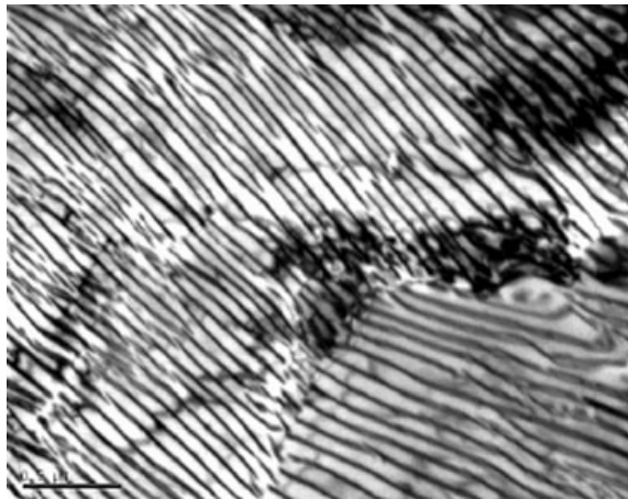
Fig. 4.22. Microstructures of the high-strength bainitic steel specimens formed at a cooling rate of 1°C/s: (a) optical micrograph of the “no-field” experiment showing the fully martensitic microstructure; (b) optical micrograph of the 30-T experiment showing a microstructure typical of cellular decomposition and no martensite; (c) bright field transmission electron micrograph of the 30-T specimen resolving the very fine pearlite microstructure.
