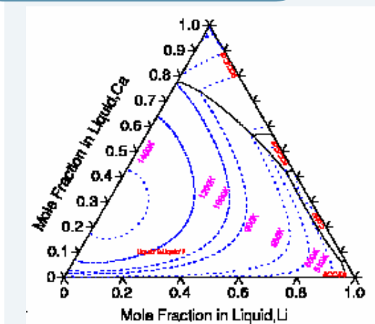
Liquidus projection of the Ca-Li-NA Ternary System.
