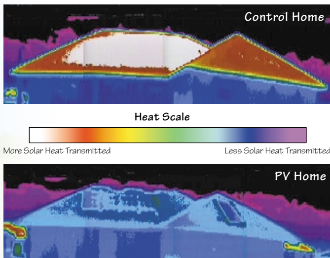
Thermographic images of the roofs in both homes. Note the lower roof and attic heat gain into the PV home, thus reducing the demand for cooling.
