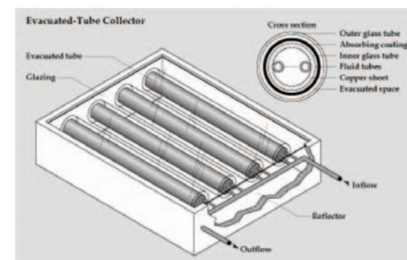
Figure 2. Flooded evacuated tube collector
