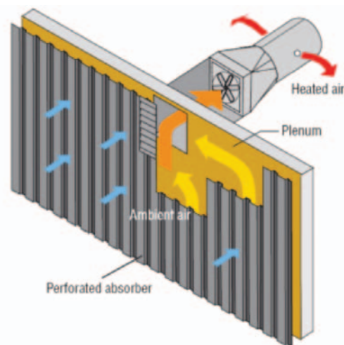
Figure 3. Transpired air collector
