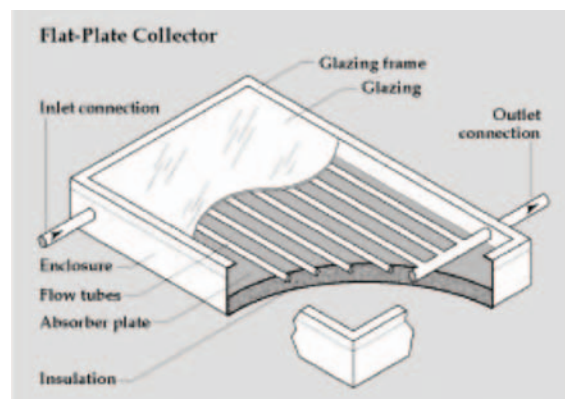
Figure 1. Flat-plate collector
