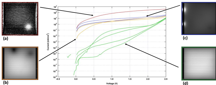
Figure 4. Initial bare cell dark IV trace curves are plotted on log scale for various cells that reside in highlighted regions of Figure 3. Each unfiltered EL image is representative of a typical cell in each region. Colors correspond accord-
