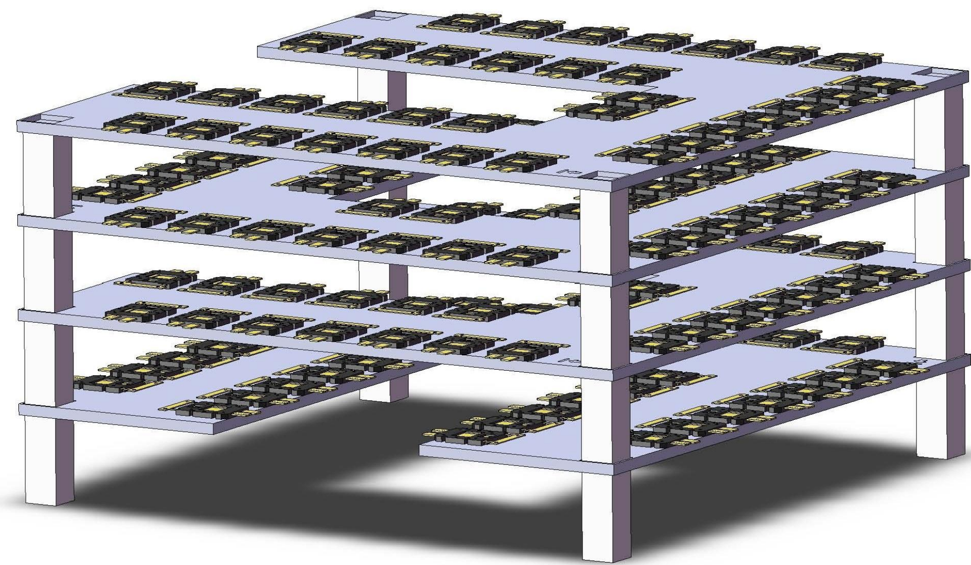
Forward Bias Test Fixture
