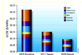
Fig. 3.1.8-5 Component contributions to LCOE for c-Si residential reference system - shown for 2005 benchmark and 2011/2020 targets.
