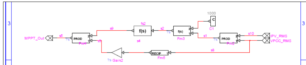
Inverter Development Model: Max Power Point Tracking algorithm implemented in Matlab.
