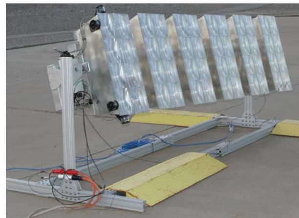
Concentrating PV Test Setup with Soliant
