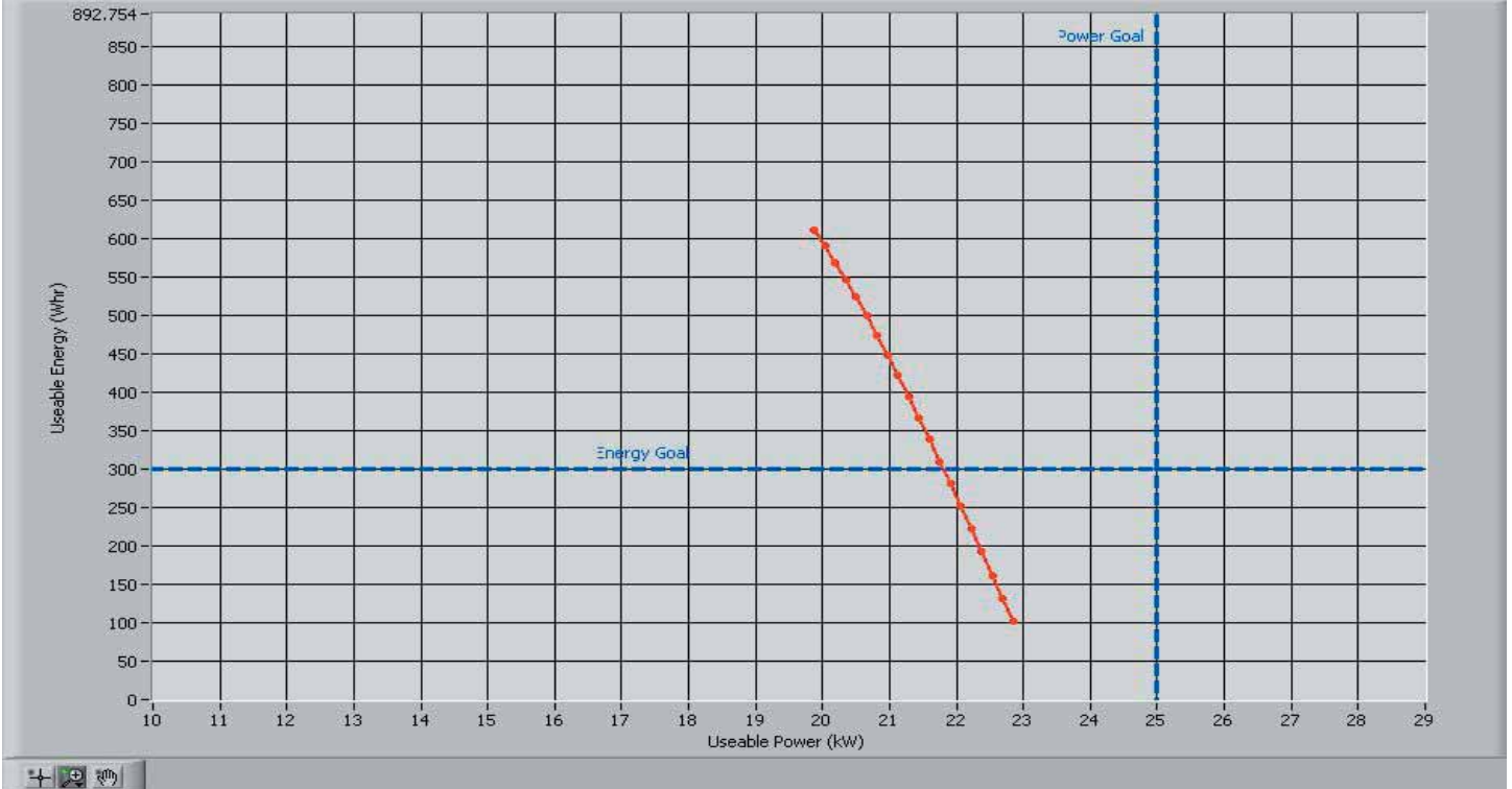
Figure 7 Useable Energy
