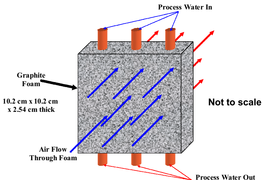
Figure 2. Schematic representation of heat exchanger with cooling air forced through pores of foam. Overall heat transfer coefficient measured at 11,000 W/m 2 ·K.
