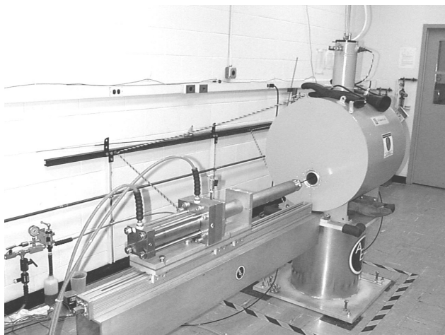
Figure 1. The Axial-Die Press Facility. Press tube is remotely moved along a track into the horizontal bore of the 9-T superconducting solenoid.
