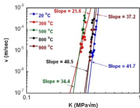
Figure 7. The effect of temperature on the slow crack growth behavior of porous cordierite in a lab environment.
