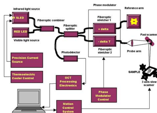
Figure 15. Block diagram of ANL's OCT system.
