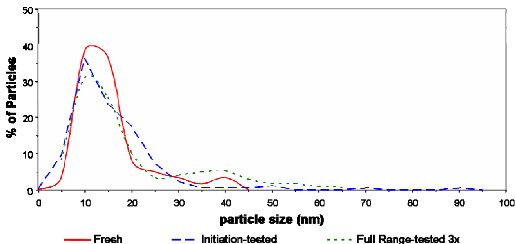
Figure 5: Particle size distribution comparison of 12 nm 2%Pt/ \gamma -alumina catalyst as determined from the STEM imaging of multiple areas, for fresh sample and those exposed to various CO oxidations conditions. Sizes have been sorted into ranges for this graph and all begin and end at zero.
