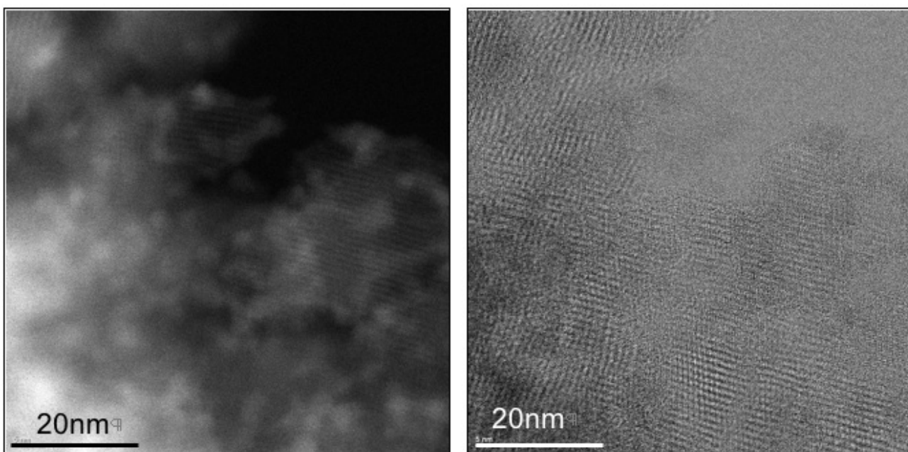
Figure 7. 700°C degreened powder sample, in HA-ADF and BF imaging. The Fe species in this area is remarkably similar to the original Fresh sample, with patches 2-4 nm in size as the predominant structure seen.
