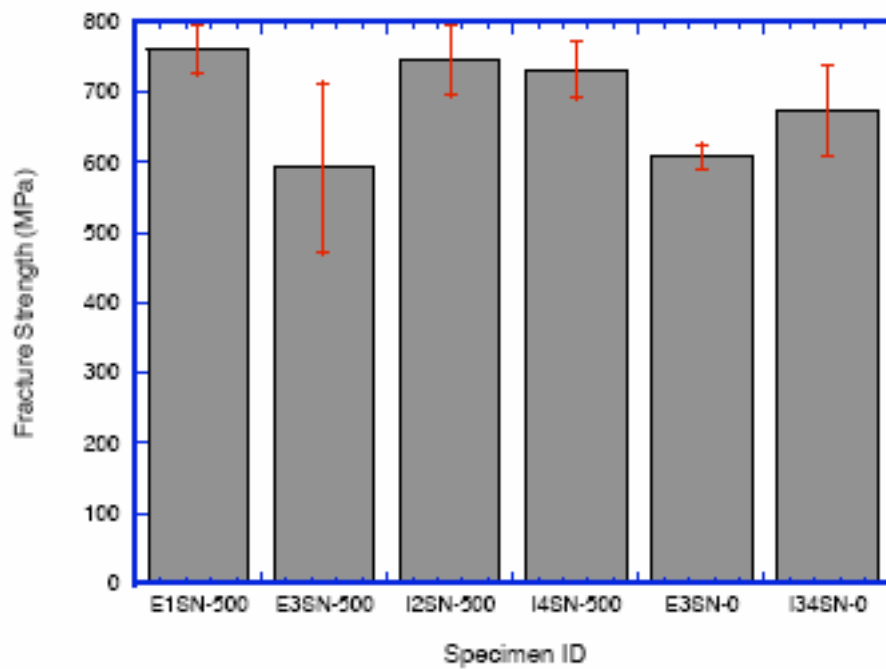
Figure 7. Fracture strength of half-cylindrical \text{Si}_3\text{N}_4 valve stems.
