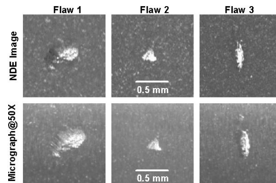
Figure 9. Detailed laser-scatter NDE images and photomicrographs of 3 flaws marked in Fig. 8.
