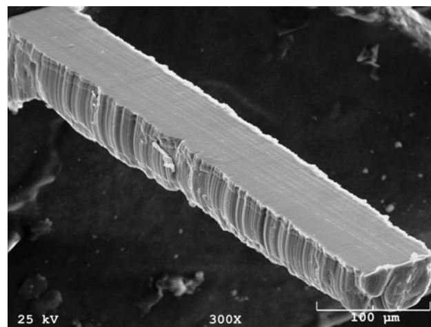
Fig. 4 SEM picture of a needle particle with aspect ratio \sim 7 . The geometry and size are controlled by the MAM conditions. The smooth surface is the
