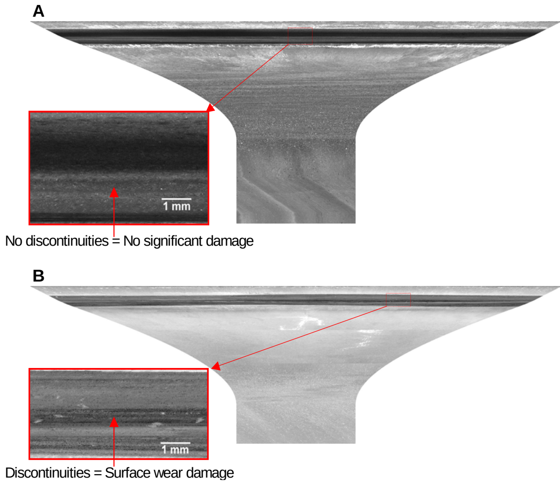
Figure 5. Laser-based NDE scans after 100 hours of engine exposure time of (A) \text{Si}_3\text{N}_4 -32 and (B) \text{TiAl} -5, indicating that the \text{Si}_3\text{N}_4 valve has not sustained major wear damage, but the \text{TiAl} valve is showing signs of significant valve/seat wear.
