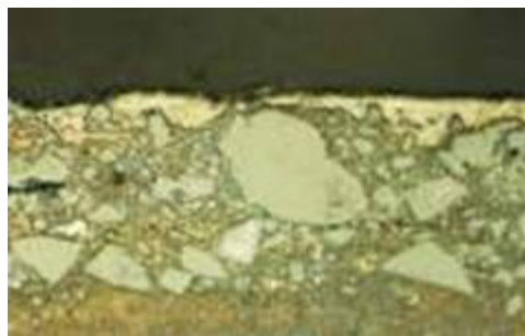
Figure 1 - 1a - Friction stir processing can close porosity in castings, producing better fatigue performance. The micrographs illustrate a cast aluminum MMC in the as-cast condition on the bottom, and as-friction stir processed (top) 1b - Ceramic particulate can also be stirred into the surface to produce functionally graded surfaces and near surface MMCs.
