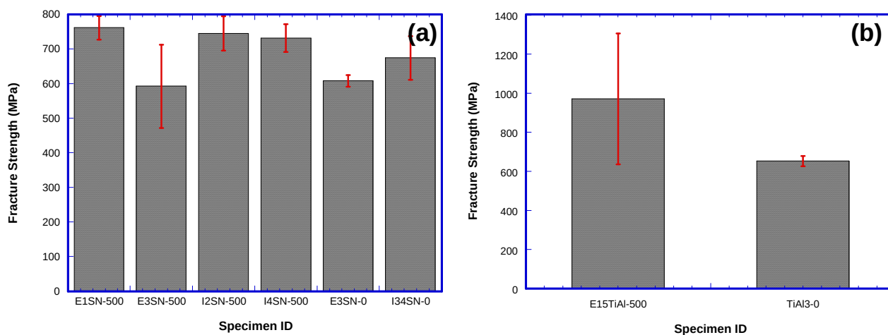
Figure 3. Fracture strength of half-cylindrical valves before and after engine test of (a) SN235P silicon nitride and (b) TiAl alloys.
