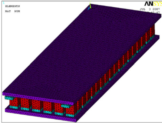
Figure 4. The mesh distribution contained 142899 elements and 240989 nodes.
