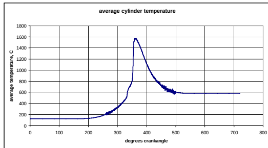
Figure 1. In-cylinder temperature conditions during HCCI combustion.
