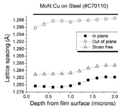
Figure 8. Lattice parameters of MoN 222 reflections for various stress-states as a function of film depth in MoNCu film deposited on steel.
