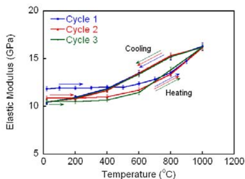
Figure 3. The temperature dependence of the elastic modulus of porous cordierite. The test specimen was subjected to three thermal loading cycles with a maximum temperature of 1000°C.
