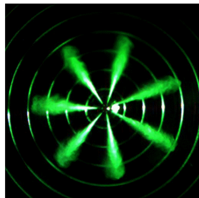
Fig. 4. Laser image of fuel spray from 50 \mu\text{m} orifice.
