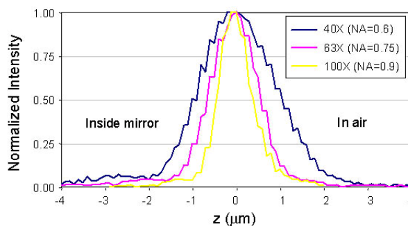
Figure 10. Axial intensity profiles obtained from mirror scan images using various objectives.
