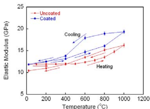
Figure 4. The effect of catalytic washcoating on the temperature dependence of the elastic modulus of porous cordierite.
