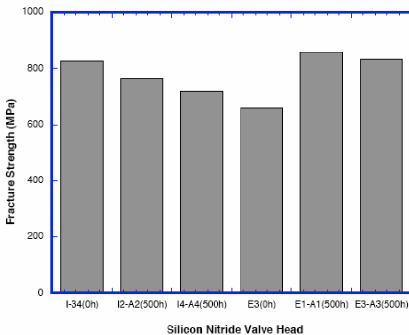
Figure 8. Fracture strength of \text{Si}_3\text{N}_4 valve heads.
