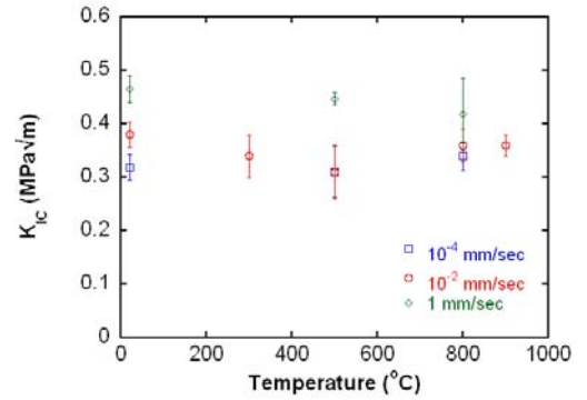
Figure 6. Fracture toughness variation of porous cordierite up to 900 °C at three different crosshead displacement rates. Every data point represents an average of five tests under that condition.
