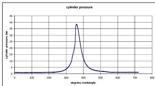
Figure 2. In-cylinder pressure conditions during HCCI combustion.
