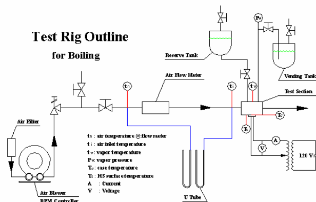
Figure 1. Test rig outline for boiling experiments
