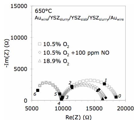
Figure 3. Nyquist plot of Au/YSZ/Au cell at 650°C in 10.5% O 2 , 10.5% O 2 + 100 ppm NO, and 18.9% O 2 .
