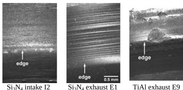
Figure 6. Photomicrographs of impact surfaces of \text{Si}_3\text{N}_4 and TiAl valves after 500-h engine test.
