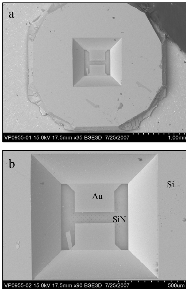
Fig. 6. a) Scanning micrograph of the back side of the Protochips heater element. b) Ceramic film (SiN) and Au electrodes shown at higher magnification.
