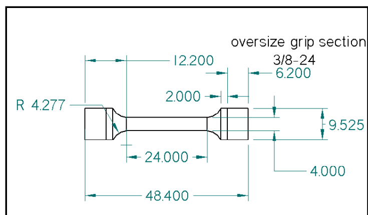
Figure 2. Schematic of cylindrical buttonhead tensile creep specimen of TiAl alloys.
