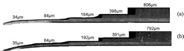
Figure 16. Micrographs and average thickness at edges of (a) NT551 (b) SN235P step wedges.
