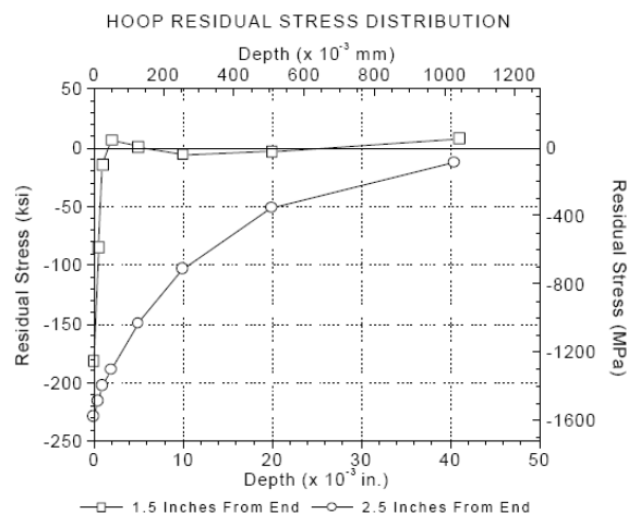
Figure 2. Stress depth profile in M50 test specimen with LSP surface treatment.
