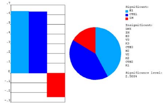
Figure 10. Sensitivity plot for the maximum principal stress in the alumina plates.
