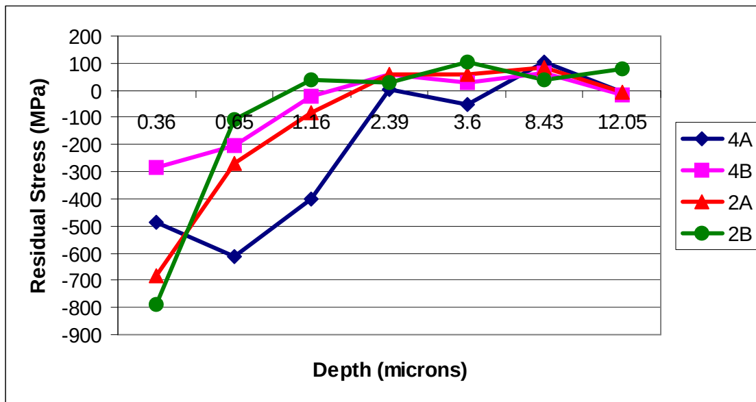
Figure 14. Relative GIXD residual stress results as a function of sample depth for machined SN235P \text{Si}_3\text{N}_4 test rods.
