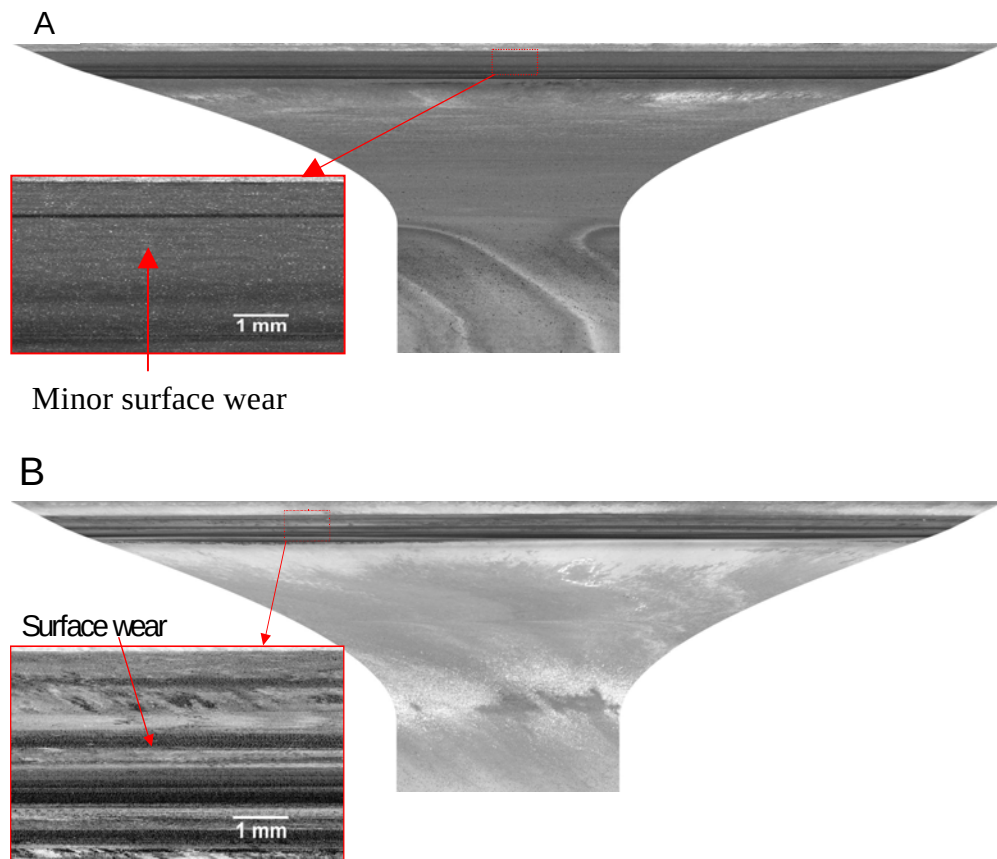
Figure 6. Laser-based NDE scans after 500 hours of engine exposure time of (A) \text{Si}_3\text{N}_4\text{E-32} and (B) \text{TiAl-5}
