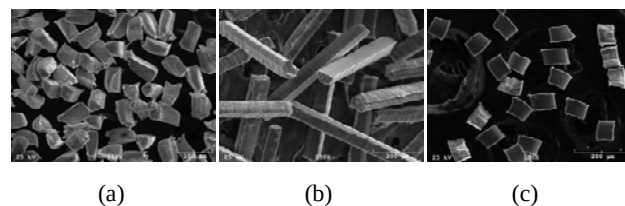
Fig. 3 Scanning electron micrographs of Al 6061-T6 particulate showing (a) equiaxed, (b) needle, and (c) platelet shapes.
