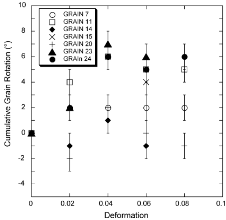
Figure 1. Cumulative grain rotation of seven surface grains as a function of strain in \text{SrTiO}_3 deformed at 1280^\circ\text{C} and 5 \times 10^{-6}/\text{s} .
