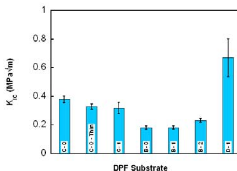
Figure 8. The average room temperature fracture toughness of the DPF substrates analyzed. The mullite substrate (D-1) has a higher fracture toughness compared to the cordierite based substrates. Five tests were carried for C-0, C-0-thin, C-1, B-0 and B-1 substrates whereas; three tests were conducted for B-2 and D-1 substrates. The error-bars represent the standard deviation of the values.
