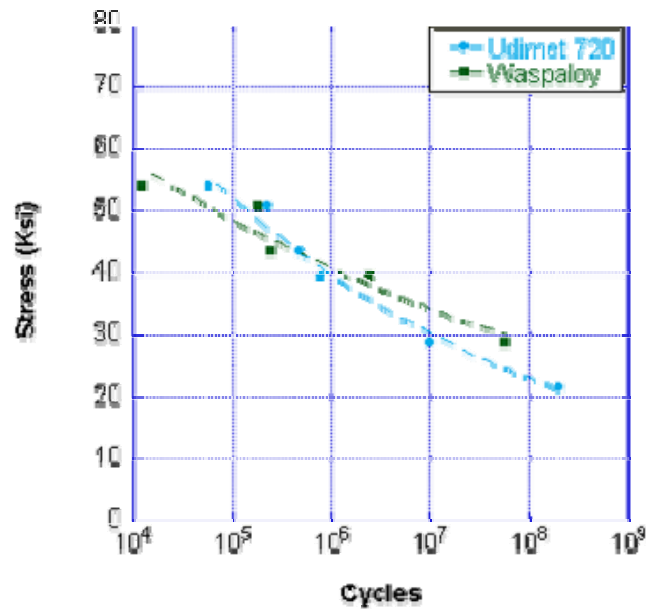
Fig. 2. Fatigue properties of Udimet 720 and Waspaloy
