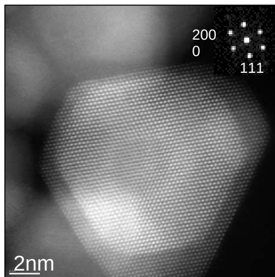
Fig. 4. Higher magnification image of a single Au-Pd nanoparticle, showing the Pd-rich core, Au-rich inner shell, and Pd-rich outer shell (see text for details).
