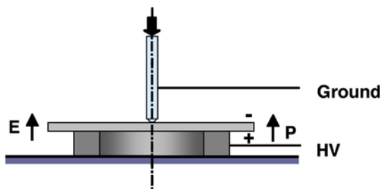
Figure 3. Cross-section of ball-on-ring test configuration for the condition when an electric field was applied across the PZT specimen with its positive poled side positioned to be loaded in tension during flexure. Four combinations were examined: positive poled side in tension or compression with or without an applied concurrent electric field.
