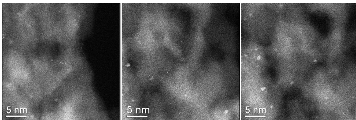
Fig. 1. a) Pt/alumina as-oxidized. Pt species dispersed almost entirely as single atoms and some dimers. b) Same area after 350°C reduction treatment for 15min. Some single atoms remain, but more small clusters of 3-4 atoms are seen. c) Same area after 350°C reduction treatment for 15min. Fewer single atoms and slight aggregation into bigger clusters.
