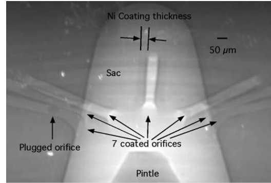
Figure 2: Phase contrast X-ray images of commercial nozzle plated with EN
