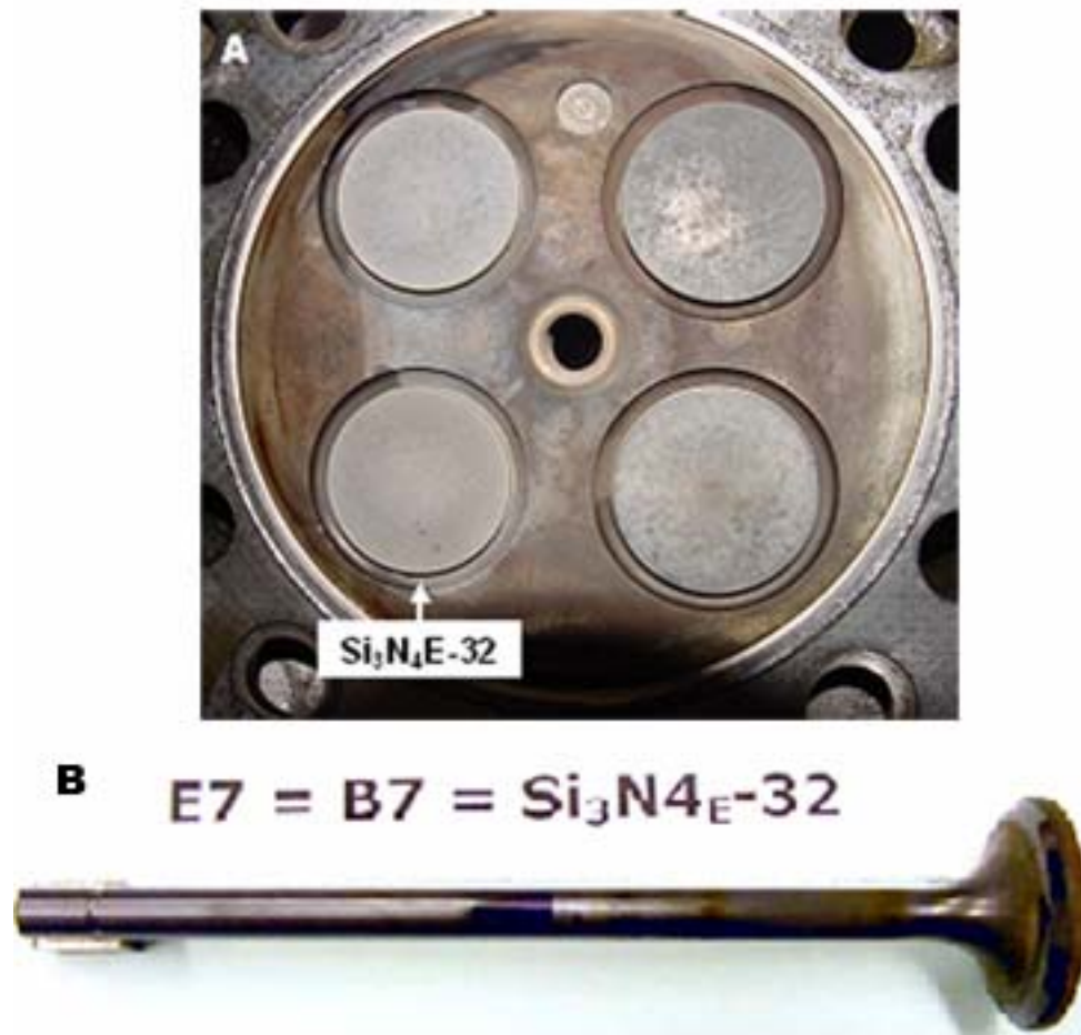
Figure 1. (A) Cylinder 2 immediately after the completion of the first 100-hour break-in phase. (B) Valve Si 3 N 4 E-32, a representative Si 3 N 4 exhaust valve after 500 hours.
