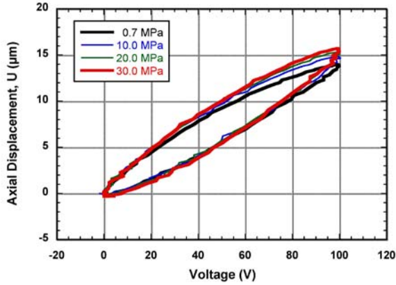
Figure 8. Axial displacement in a PMLA as a function of applied voltage.
