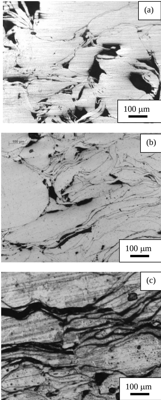
Fig. 5 Optical micrographs Al-6061-T6 chip powder produced by milling and mixed with liquid epoxy: M-bond epoxy ( \eta \sim 1 mPa-s) pressed at 500 MPa (a)
