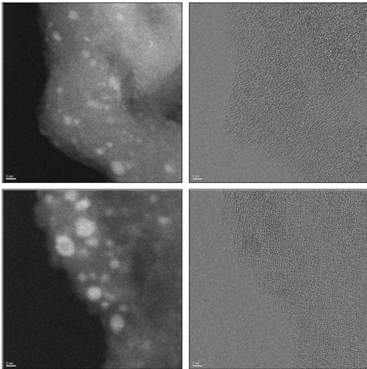
Figure 5. a,c, left) HA-ADF images of two different areas of the ion-milled Fresh powder sample, showing patches of Fe in bright contrast; b,d, right) corresponding BF images showing faint contrast from the heavy metal patches.
