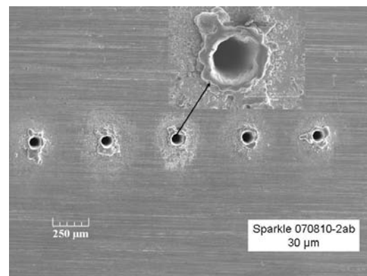
Figure 6: Scanning electron image of the entrance surface of percussion drilled orifices.
