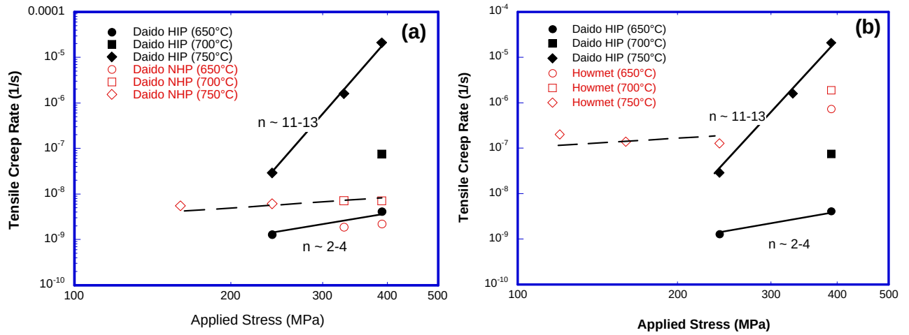
Figure 8. Tensile creep rates versus applied stress curves of Diado TiAl alloy (a) and Howmet TiAl alloy (b).
