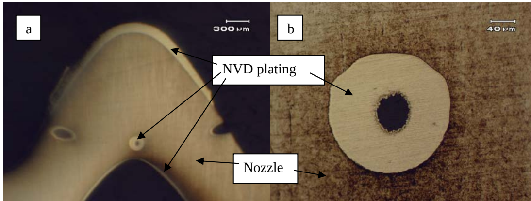
Figure 5: Low (a) and high (b) magnification optical images of a cross-sectioned, polished, and etched (Nital) six-orifice nozzle after NVD.
