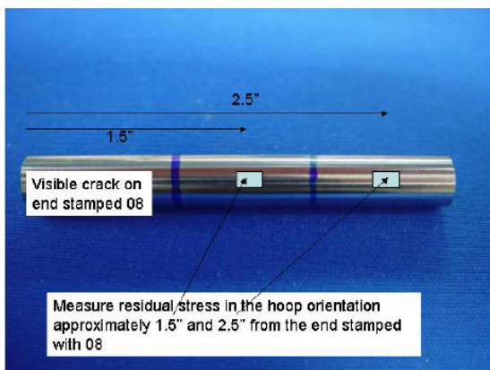
Figure 1. Photograph of test specimen stress measurement locations.
