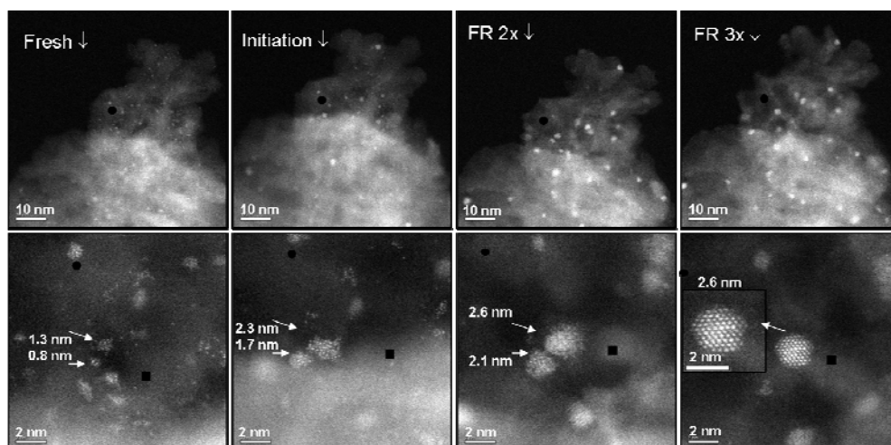
Figure 3: ACEM HAADF-STEM images of the exact same sample area of fresh 2%Pt/ \gamma -Al 2 O 3 , after CO oxidation initiation, after 2-, and 3-cycles of quantitative CO-conversion (left to right, respectively). The second row shows the area at higher magnification for each stage, respectively. Circles and squares are located at the same place on each image to allow monitoring of Pt growth at each stage of testing.
