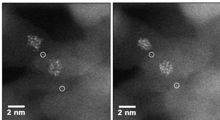
Fig. 2. Frames from a “movie” of the 700°C/15min reduction treatment (starting from a fresh as-oxidized Pt/alumina sample). Rafts of 20-30 atoms were seen, which tended to rearrange slightly under beam exposure, while single atoms (circled) are pinned to the alumina.
