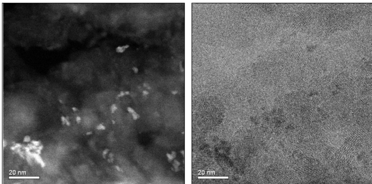
Figure 8. 700°C degreened powder sample, in HA-ADF and BF imaging. The Fe morphology in this area shows strong contrast in both images, suggesting the Fe species has formed more discrete particles of several atomic layers.
