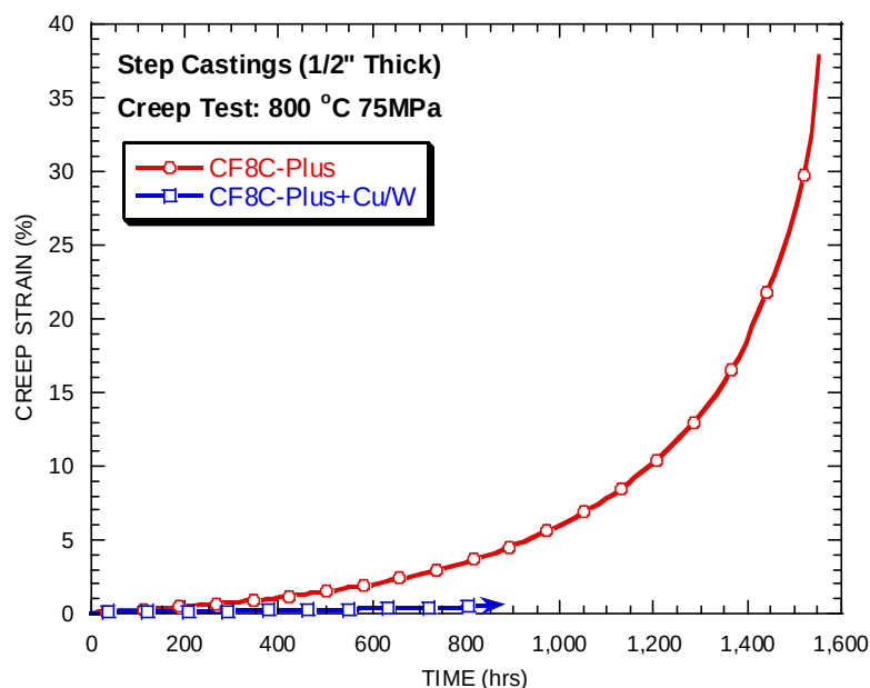
Figure 4. Plots of creep-strain vs time for new thin-section step-cast heats of CF8C-Plus and the new CF8C-Plus Cu/W, all tested in air at 800°C and 75 MPa. Clearly the CF8C-Plus Cu/W has much more creep-resistance, with an extended secondary creep-regime and a very low steady-state creep rate, which is very important for applications like turbocharger housings
