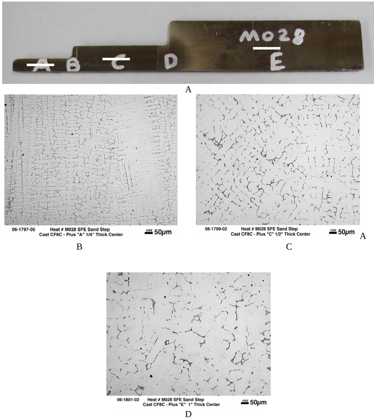
Figure 2 – A) Macro-photo of CF8C-Plus stainless steels step casting, with 1.0, 0.5 and 0.25 inch step thicknesses, and etched metallographic cross-sections showing the as-cast dendritic structure of the B) 0.25 inch thick section (marked A), C) the 0.5 inch thick section (marked C), and D) the 1.0 inch thick section (marked E) in the photo above.
