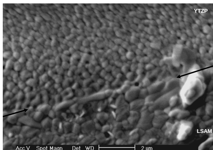
Figure 7. High-resolution SEM of the joining plane in YTZP/LSAM/YTZP joined at 1250°C.
