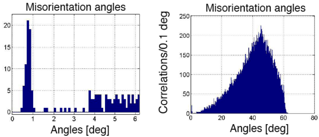
Fig.3. Misorientation angles after straining from 0.05% to 0.45%. Sixty-four grains have been correlated and tracked.
