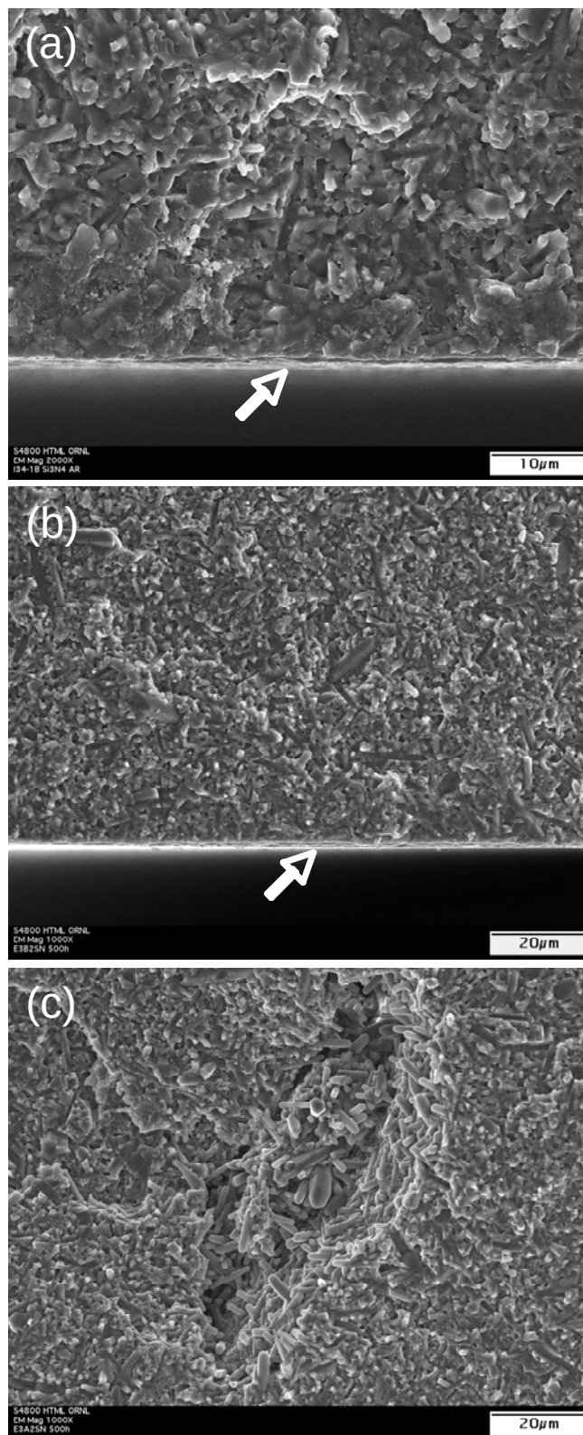
Figure 5. Scanning electron microscopy fracture surface features of silicon nitride valve stem before (a) and after engine test (b and c).
