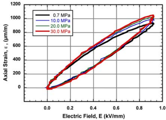
Figure 9. Calculated axial strain in a PMLA as a function of calculated electric field.
