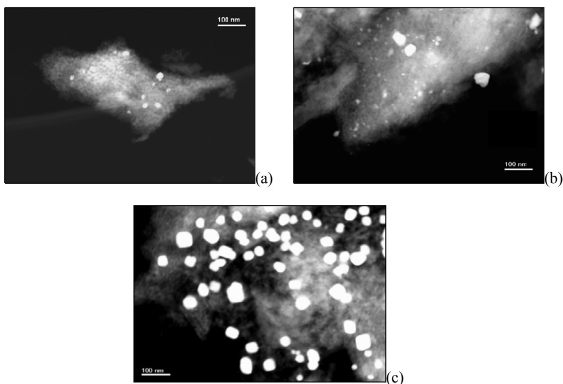
Figure 4: STEM images of fresh 12 nm 2%Pt/ \gamma -alumina (a), after CO oxidation initiation (b) and after 3 cycles of quantitative CO oxidation (c).
