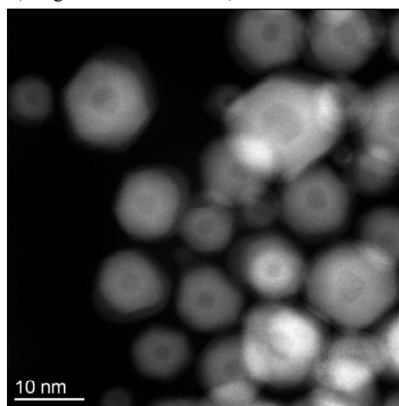
Fig. 3. As-synthesized Au-Pd particles showing core/inner/outer shell structure.
