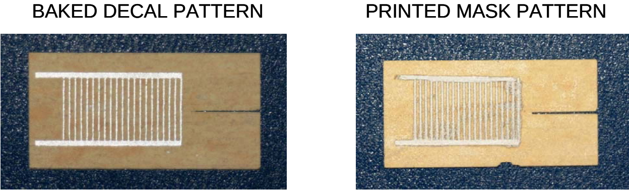
Figure 14. Images of two different kinds of crack-gages bonded to double-torsion specimens of porous cordierite. (a) Decal pattern baked on DT specimen and (b) Printed mask of cermet paste baked on ceramic substrate.
