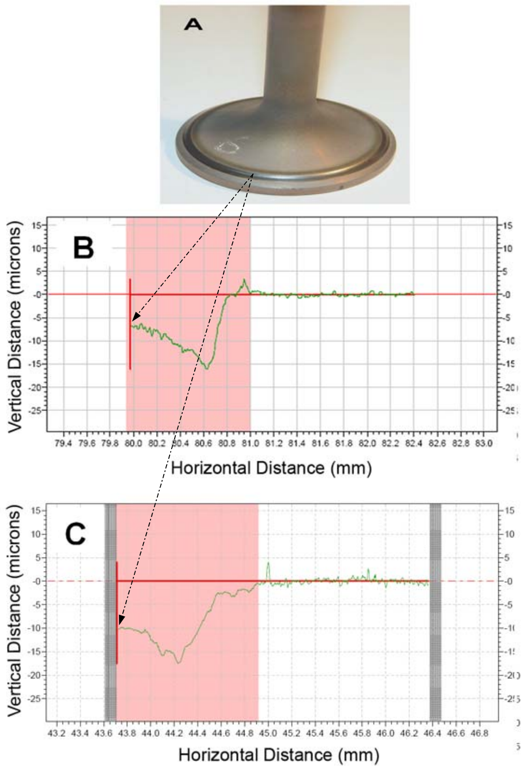
Figure 4. (A) Seat area where profilometry was taken from (B) 100- and (C) 500-hour TiAl wear patterns.
