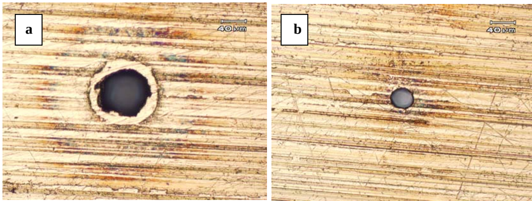
Figure 7: Optical images of the entrance (a) and exit (b) surfaces of percussion drilled orifices.
