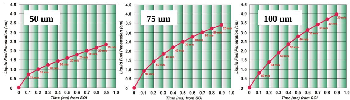
Figure 4: Fuel penetration as a function of time from start of injection (SOI) for 50, 75, and 100 \mu\text{m} nozzles. 7
