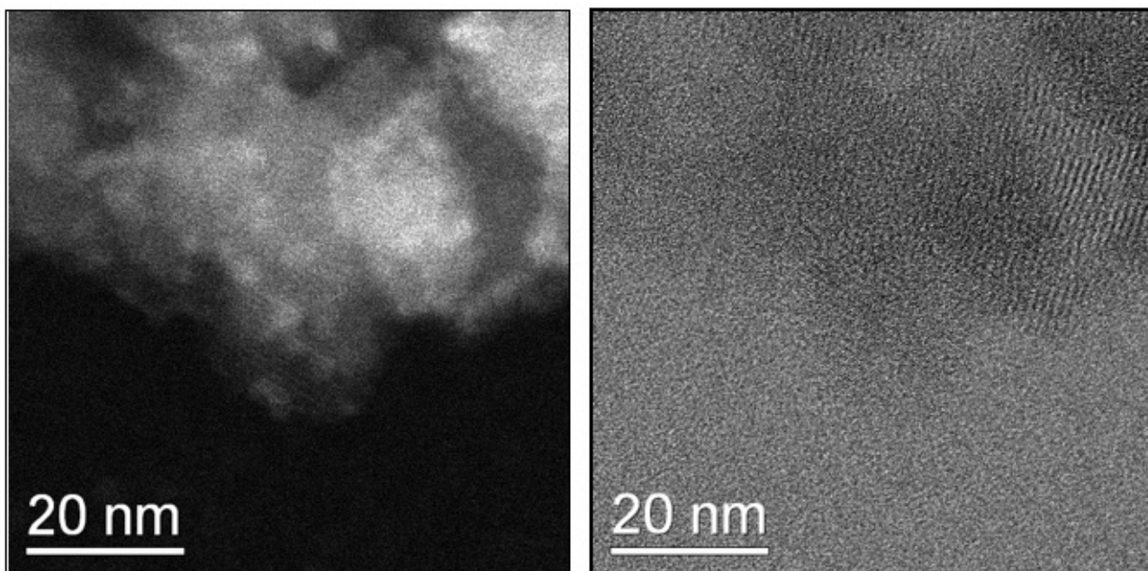
Figure 2. HA-ADF/BF pair of micrographs of fresh Fe/zeolite powder. The bright areas in the HA-ADF image are the Fe-rich phase.
