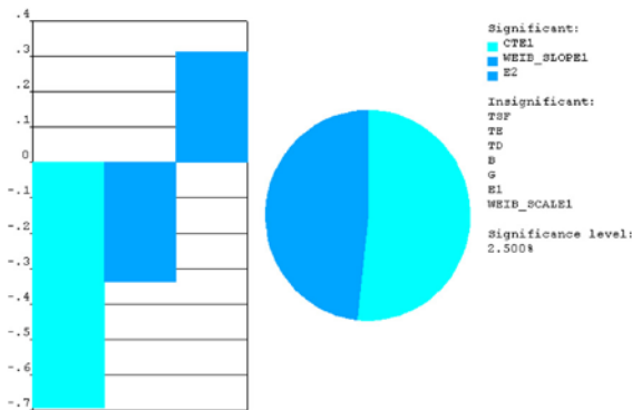
Figure 9. CTE mismatch, Weibull modulus, and electrode elastic modulus had the largest effect on ceramic probability of failure.
