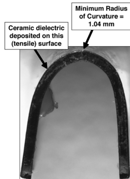
Figure 5. Mechanically evaluated ceramic dielectric - nickel substrate system.
