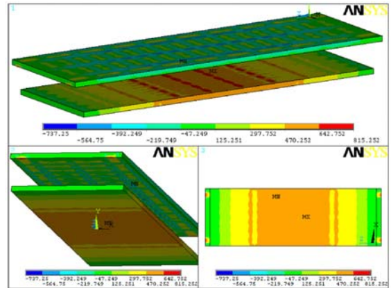
Figure 7. First principal stresses in the alumina plates due to the thermal loading.
