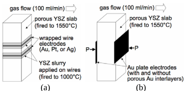
Figure 2. Schematic of (a) wire setup to investigate composition (Au, Pt, and Ag) and (b) plate setup to investigate microstructure (dense and porous Au)
