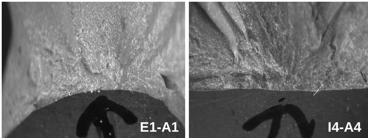
Figure 7. Fractography photo of tested SN235P exhaust (a) and intake (b) valve head.
