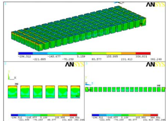
Figure 8. First principal stresses in the TE legs due to the thermal loading.
