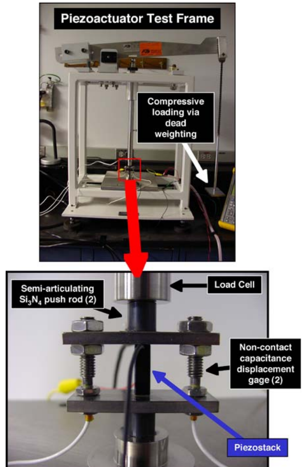
Figure 7. Test setup that enables PMLA fatigue characterization.
