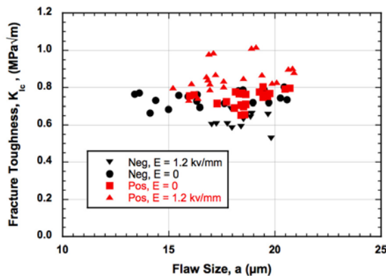
Figure 6. Fracture toughness as a function of poled direction and electric field.
