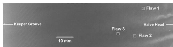
Figure 8. Laser-scatter scan image of stem surface of \text{Si}_3\text{N}_4 intake valve Cyl6-I#22.
