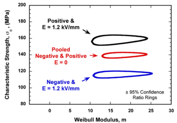
Figure 4. Confidence ratio rings of characteristic strength and Weibull modulus of the four test conditions. Specimens had nominal dimensions of 10 x 10 x 0.273 mm, and the diameters of the loading ball and support ring were 2.0 and 7.4 mm, respectively.
