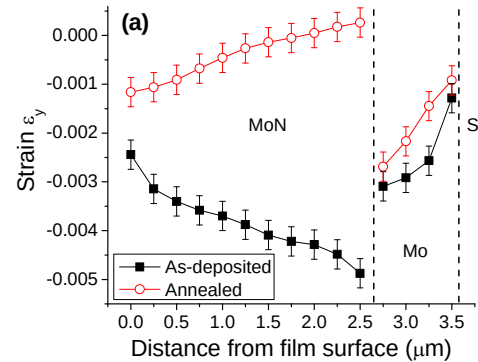
Figure 4: Depth-resolved residual strain for as-deposited and annealed MoN/Mo bilayer films as determined from cross-section technique.
