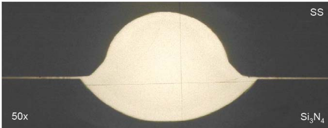
Figure 12. Keeper groove from a production stainless steel (SS) and \text{Si}_3\text{N}_4 valve.
