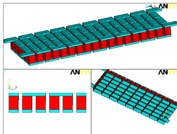
Figure 2. Views of the TE module with the insulator plates removed to show the arrangement of the steel and TE legs.
