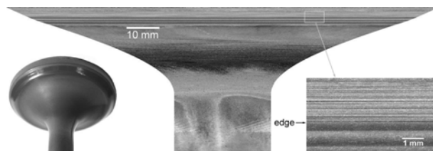
Figure 4. Laser-scatter scan image of \text{Si}_3\text{N}_4 exhaust valve E1 after 500-h engine test.
