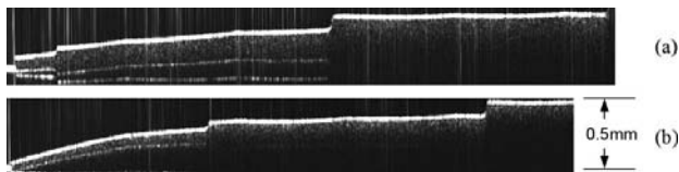
Figure 17. Scanned cross-sectional OCT images for (a) NT551 and (b) SN235P step wedges.
