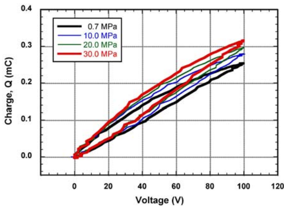
Figure 10. Charge in a PMLA as a function of applied voltage.
