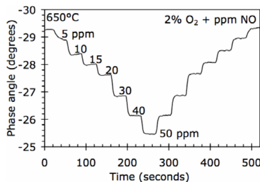
Figure 4. Impedancemetric sensing behavior of Au-wire wrapped porous YSZ slab using the phase angle response at 10 Hz as the sensing signal.
