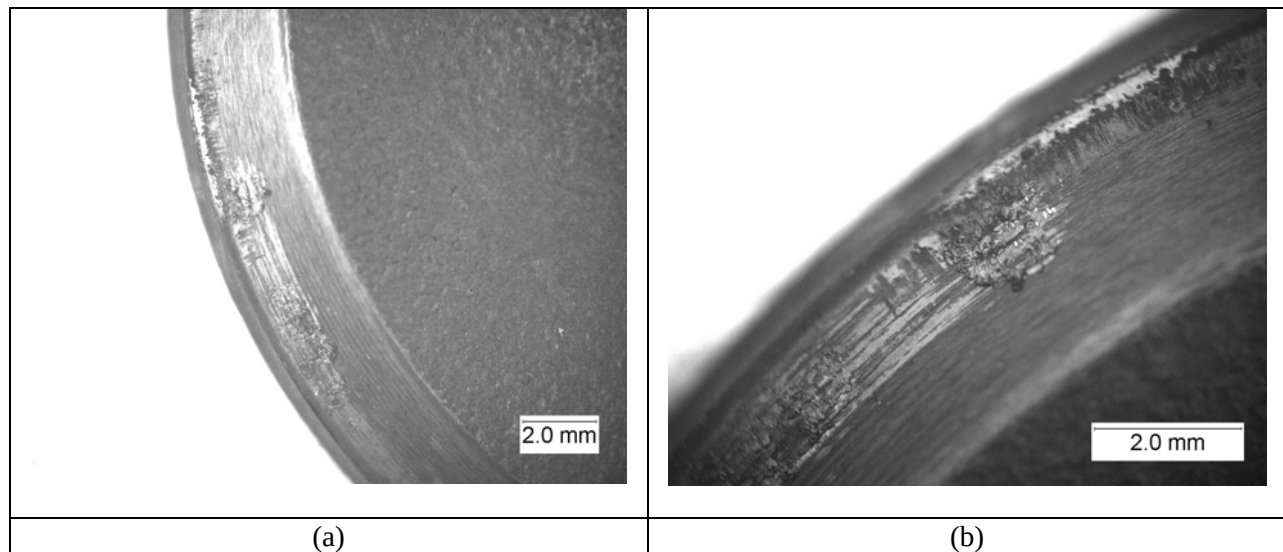
Figure 2. Close-up views of a commercial diesel exhaust valve subjected to 20,000 impacts at 800°C in the HTRI. Significant micro-welding, plastic deformation, and material transfer are indicated.
