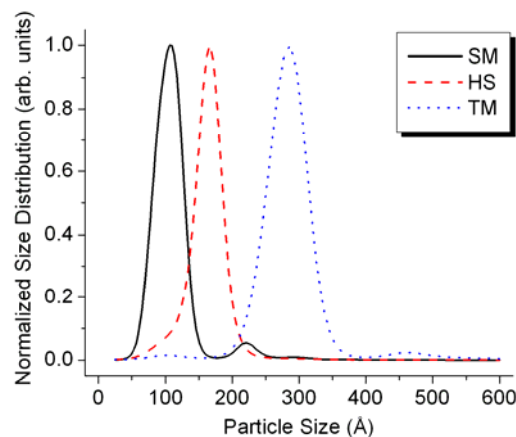
Fig. 5. Particle size distribution of three silica nanofluid samples
