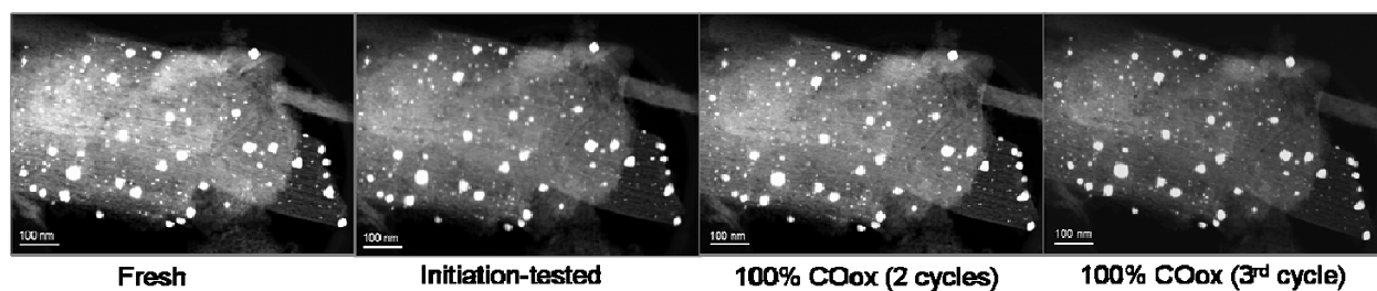
Figure 7: HAADF-STEM images of the exact same sample area throughout the ex-situ CO oxidation study on Fresh 12 nm 2%Pt/ \gamma -Al 2 O 3 . Images after CO oxidation initiation-testing, 2 cycles of quantitative oxidation and a 3 rd cycle of quantitative oxidation are shown.
