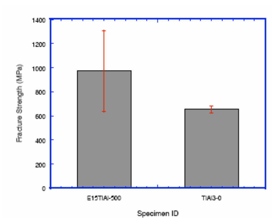
Figure 9. Fracture strength of half-cylindrical TiAl valve stems.
