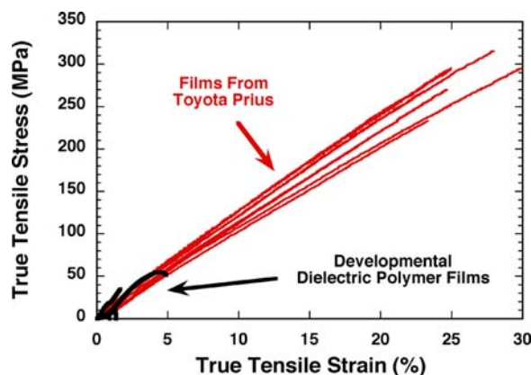
Figure 2. Comparison of tensile strain-to-failures of PPOD dielectric film and the film from capacitor from a Toyota Prius hybrid.
