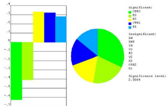
Figure 11. Sensitivity plot for the maximum principal stress in the TE legs.
