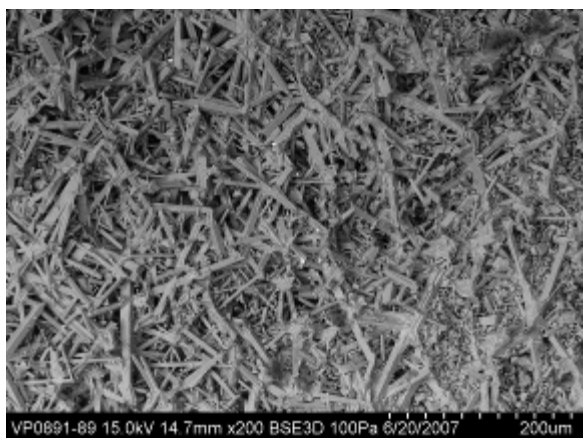
Figure 9. SEM image of the interlocking microstructure, of the mullite (D-1) DPF substrate, that is responsible for its increased fracture toughness.
