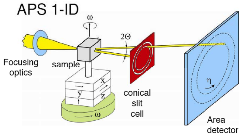
Figure 2. Experimental setup for measuring grain rotation as a function of strain.
