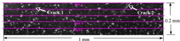
Figure 11. Plane confocal-scan image of a NT551 silicon nitride specimen with two C cracks.
