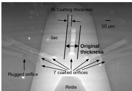
Fig. 3. Phase contrast X-ray image of commercial nozzle plated with electroless nickel
