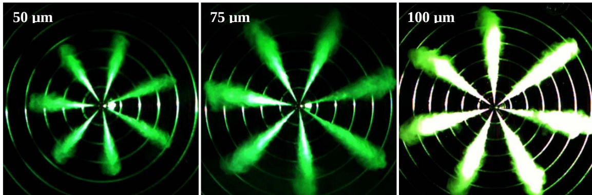
Figure 3: Laser images of fuel sprays from 50, 75, and 100 \mu\text{m} orifices. 7
