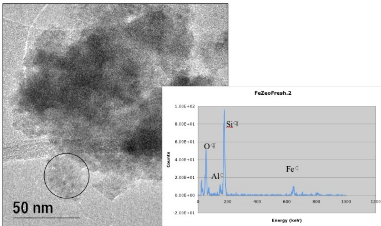
Figure 4. BF image of Zeolite aggregate in the HF-2000 TEM. Circled area shows dark patches equivalent to the bright patches seen in the ACEM HA-ADF images. The presence of Fe in this thin flake of material is confirmed by the EDS spectrum inset; the O, Al and Si peaks originate from the aluminosilicate zeolite structure.
