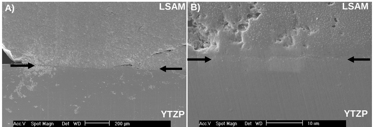
Figure 6. Joining plane of \text{La}_{0.77}\text{Sr}_{0.20}\text{Al}_{0.9}\text{Mn}_{0.1}\text{O}_3 joined to YTZP at 1350°C. Arrows denote the joining plane. A) Wide view of joint. B) The same joint viewed at higher magnification exhibits that a joint was created even though the material is not fully dense.
