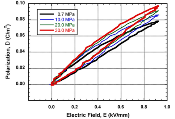
Figure 11. Calculated polarization in a PMLA as a function of calculated electric field.
