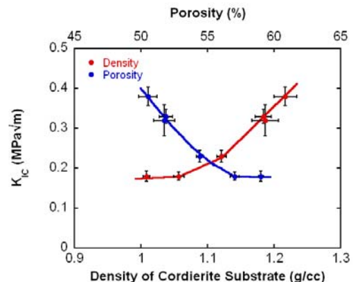
Figure 10. The variation in the fracture toughness of the cordierite substrates as a function of density and porosity of the substrate.
