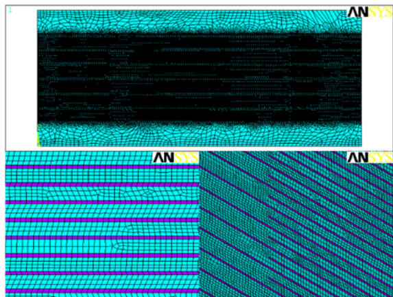
Figure 6. The MLCC 2-D mesh contained ~96,000 elements and ~290,000 nodes.
