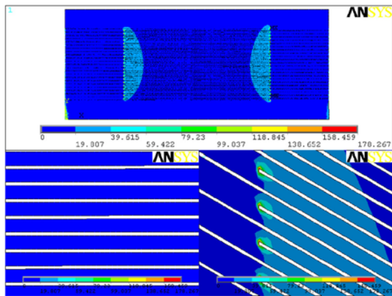
Figure 7. First principal (residual) stress distribution in the dielectric ceramic.
