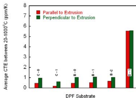
Figure 12. The coefficient of thermal expansion (CTE) of the DPF substrates analyzed. The CTE values reported are the between 20 and 1000°C and in directions that are parallel and perpendicular to the extrusion direction. One measurement each in the parallel and perpendicular direction.
