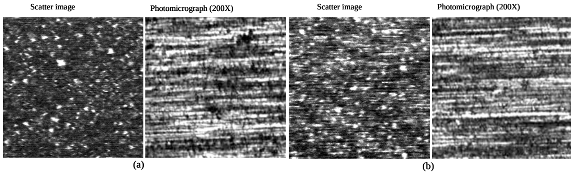
Figure 13. (A) Finished and (B) rough machined \text{Si}_3\text{N}_4 specimens.
