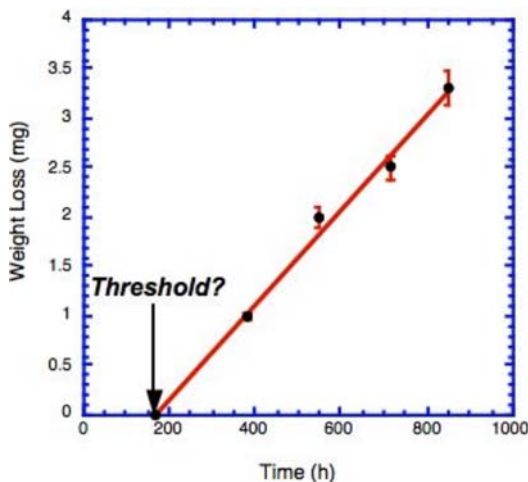
Fig. 1. Weight loss vs. time for an impact angle of 30°, velocity of 7.7 m/s using a 0.1 vol % CuO nanoparticles in ethylene glycol
