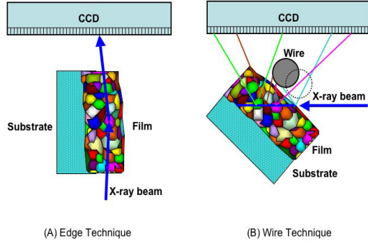
Figure 3. Experimental set-up used for stress evaluations: (A) Edge and (B) Wire techniques.
