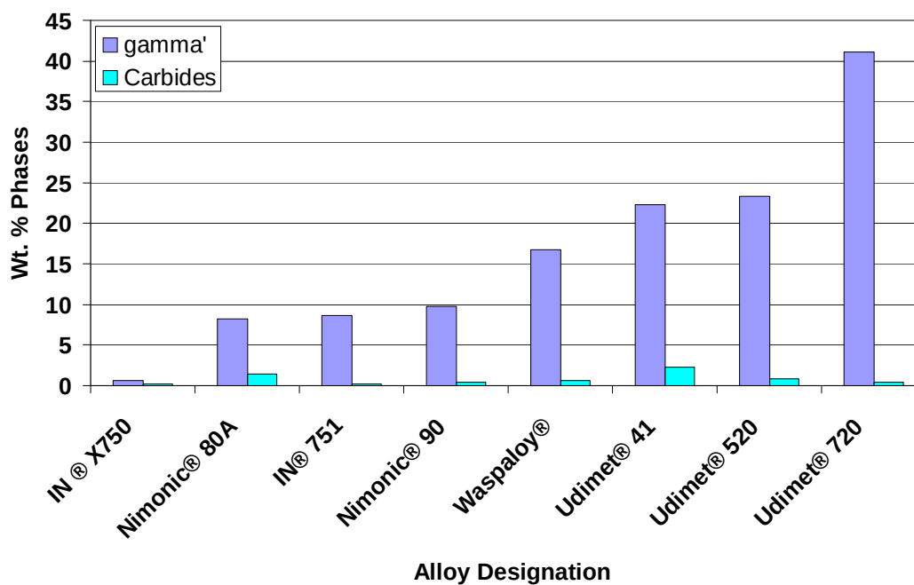
Figure 2. Variation in wt. % of \gamma' and carbides at 870°C in the various alloys used in the study.
