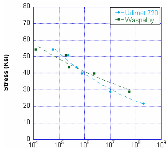
Figure 3. Typical Stress vs. Number of Cycles to Failure (S-N) curve for Udimet 720 and Waspaloy at 870°C.
