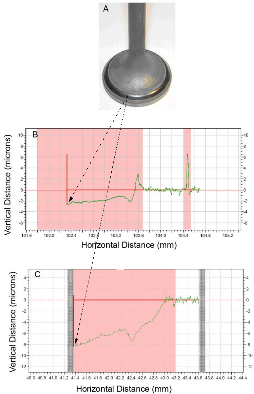
Figure 2. (A) Seat area where profilometry was taken from (B) 100- and (C) 500-hour \text{Si}_3\text{N}_4 wear patterns.
