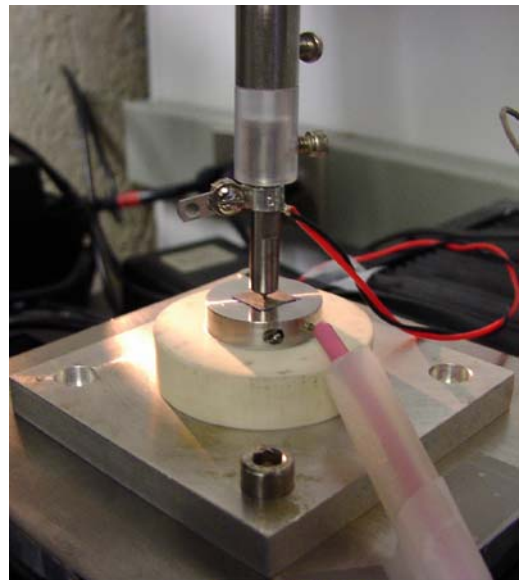
Figure 2. Setup of the ball-on-ring biaxial flexure strength test with capability to apply concurrent electric field.
