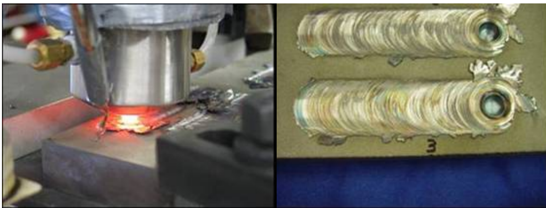
Figure 6. FSP test in progress (left) and initial results showing that ceramic coatings can be stirred into the substrate (right).
