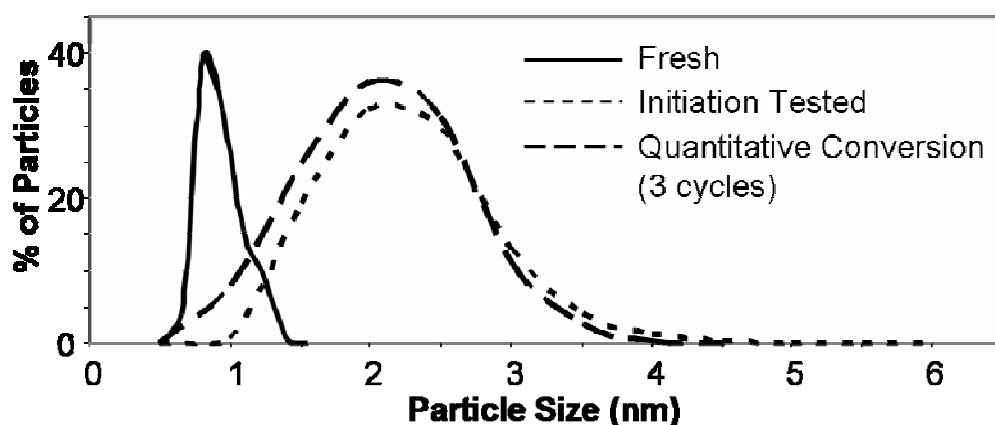
Figure 9: Particle size distribution of 1 nm 2%Pt/ \theta -alumina catalyst as determined from STEM imaging of multiple areas for fresh samples and those exposed to various CO oxidations conditions. Sizes have been sorted into ranges for this graph and all begin and end at zero.
