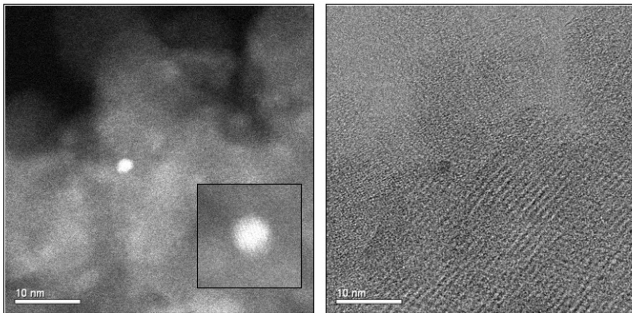
Figure 3. HA-ADF/BF pair of micrographs of showing presence of discrete crystallite. The inset in 3a shows the crystallite lattice, illustrating that it is a 2-3 nm diameter single crystal. The BF image clearly shows channels in the zeolite structure.
