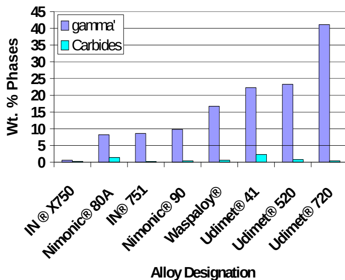
Fig. 1. Calculated amounts of strengthening phases in selected alloys
