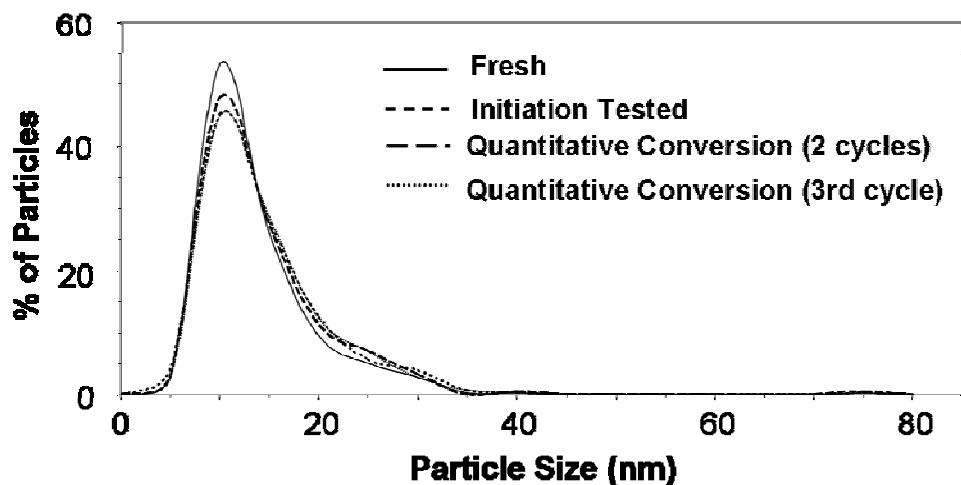
Figure 6: Pt particle size distribution for 12 nm 2%Pt/ \gamma -Al 2 O 3 fresh catalyst and after CO oxidation on the ex-situ reactor, as determined from HAADF-STEM micrographs. Sizes have been sorted into ranges for this graph and all begin and end at zero.
