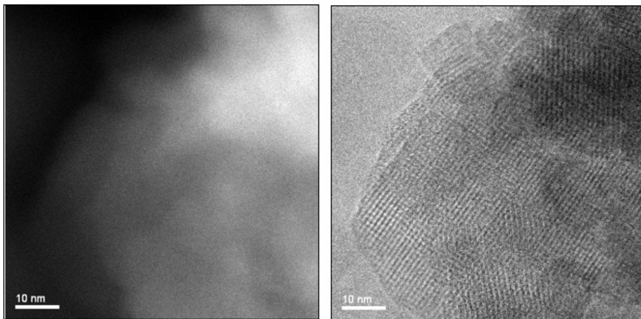
Figure 1. a) HA-ADF image of H-beta-zeolite blank material, showing uniform contrast with no evidence of heavy element scattering; b) Corresponding BF image showing crystal lattice that indicates the high resolution of the incident probe.
