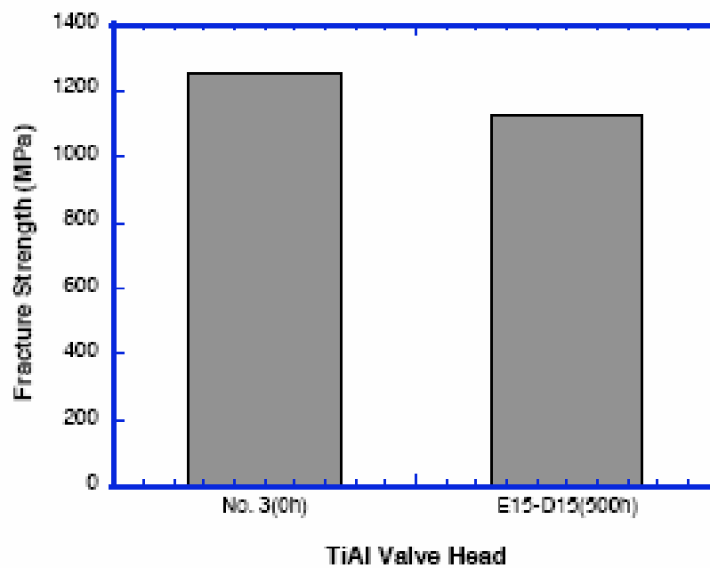
Figure 10. Fracture strength of TiAl valve heads.
