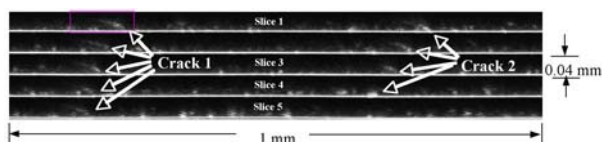
Figure 12. Five cross-sectional confocal-scan images along slice lines 1-5 as indicated in Fig. 11.
