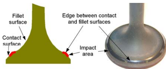
Figure 2. Location of impact area on valve surface.
