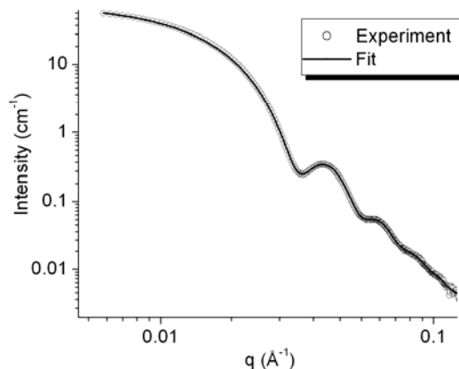
Fig. 4. SAXS data of a 0.02 vol% SiO 2 nanofluid and a fit using the maximum entropy method assuming spherical particles with an average diameter of 17 nm.
