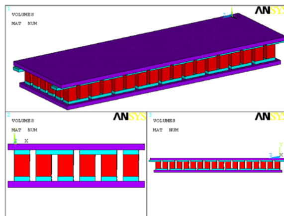
Figure 1. Various views of the TE module with colors corresponding to material sequence. Purple is the alumina, turquoise is the steel, red is the TE legs.
