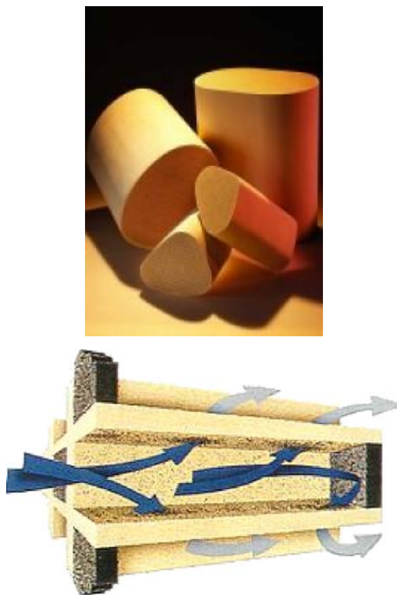
Figure 1. Corning's cordierite-based DPFs.
