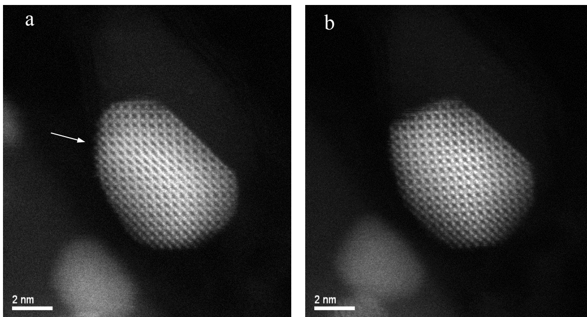
Fig. 9. HA-ADF images of Pt on alumina, at a nominal 1000°C, taken at an original magnification of 10Mx. These images show two “frames” from a 20-image “movie” that followed the changes in particle morphology with time. The particle structure is clearly ordered, indicating a compound has formed, likely a Pt-oxide composition, under these treatment conditions. Note changes in facets, and the details of exposed atomic columns on the surface, such as at the arrows in a).
