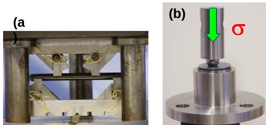
Figure 1. Photo of four-point bending fixture used for testing the half-cylindrical valve stems (a) and custom-designed fixture for the valve head testing.
