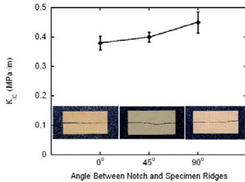
Figure 5. Fracture toughness of porous cordierite at room temperature as a function of orientation.
