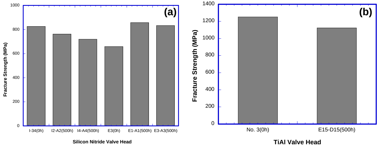
Figure 6. Comparison of fracture strength of valve head before and after engine test. (a) SN235P silicon nitride valves and (b) TiAl valves.
