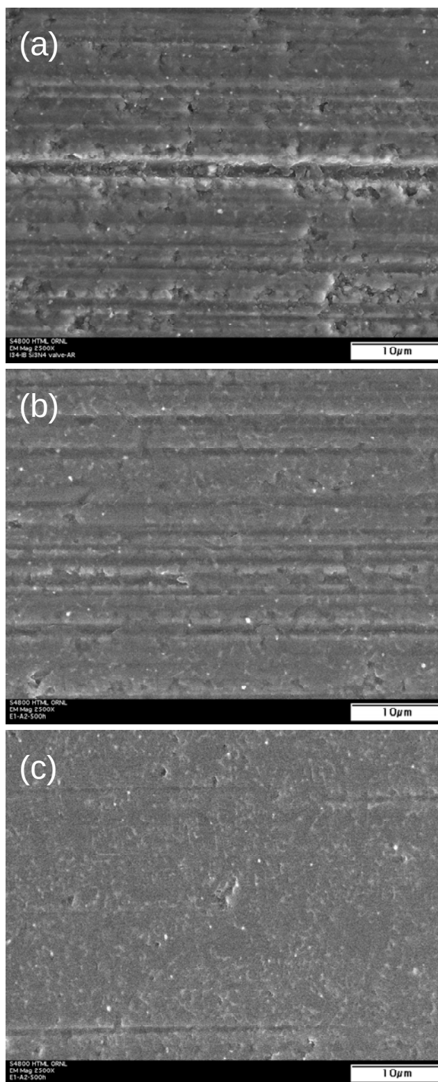
Figure 4. Scanning electron microscopy surface features of silicon nitride valve stem region before (a) and after engine test (b and c).
