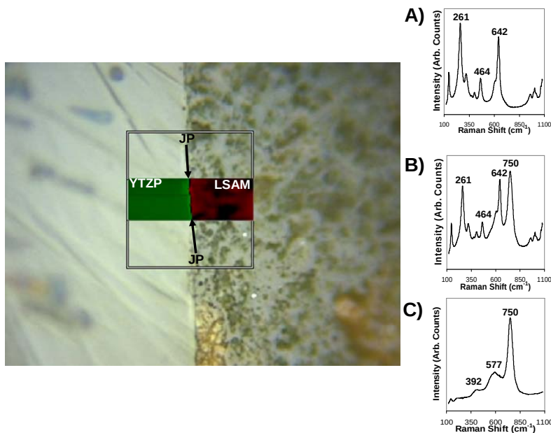
Figure 9. Raman map of interface in sample joined at 1250°C. The joining plane is the narrow region denoted as JP that lies between the bulk of YTZP and LSAM. A) Representative spectrum of the YTZP region marked in green. B) Representative spectrum of the joining plane denoted by arrows. C) Representative spectrum of the LSAM region marked in red.
