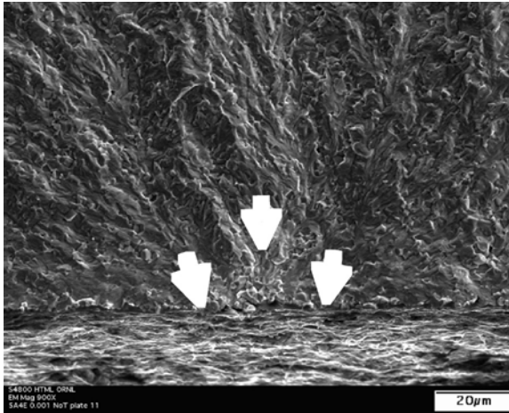
Figure 5. Example of a strength-limiting flaw.
