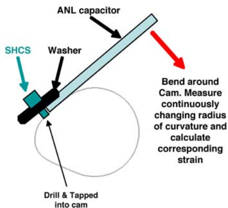
Figure 3. Schematic of the bend test used to estimate strain-to-failure of the ceramic dielectric.
