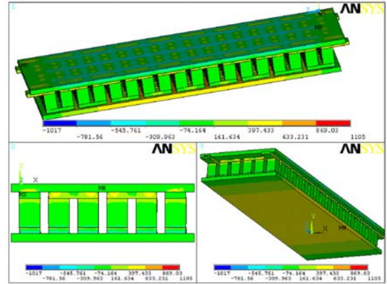
Figure 6. First principal stresses in the TE device due to the thermal loading.
