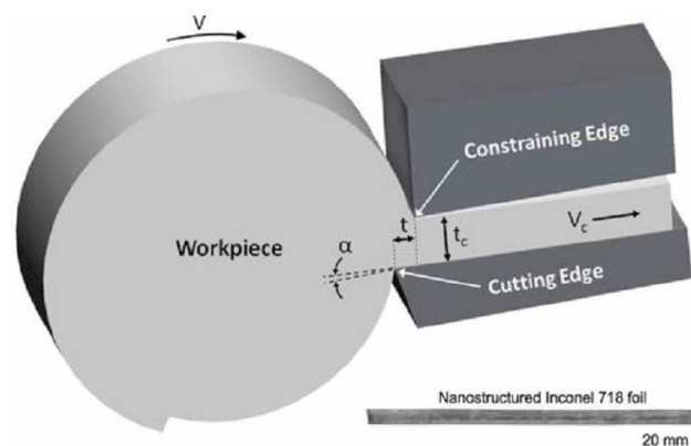
Fig. 1 Schematic of large-strain extrusion machining (LSEM). Inset at bottom right shows a typical Inconel 718 sheet strip created using this process.
