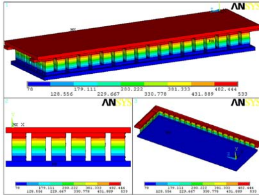
Figure 5. Temperature distribution in °C.
