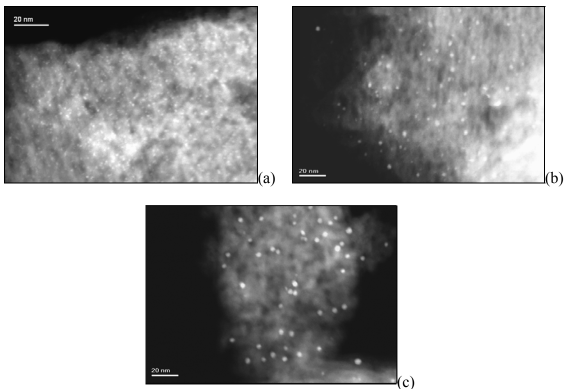
Figure 1: STEM images of fresh 1nm 2%Pt/ \gamma -alumina (a), after CO oxidation initiation (b) and after 3 cycles of quantitative CO oxidation
