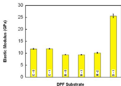
Figure 11. The room temperature elastic modulus of the DPF substrates analyzed. Isotropic elasticity was assumed. The error bars represent the RMS error of the fit for one measurement.
