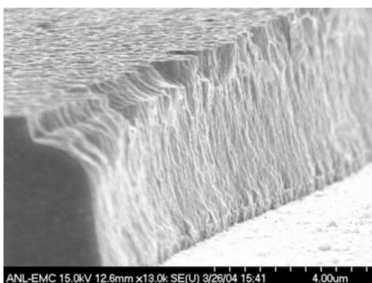
Figure 2: Cross-sectional SEM of a MoNCu/Mo film deposited on steel substrate.
