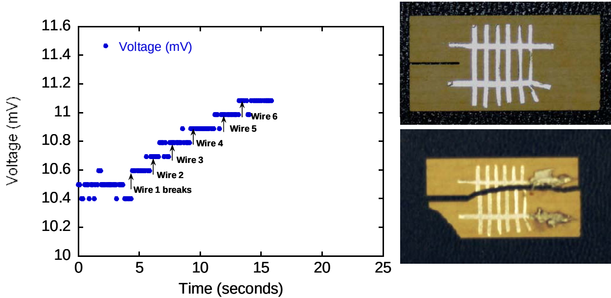
Figure 15. Implementation of developed crack-gages in voltage divider circuits to detect crack growth in porous cordierite substrates.
