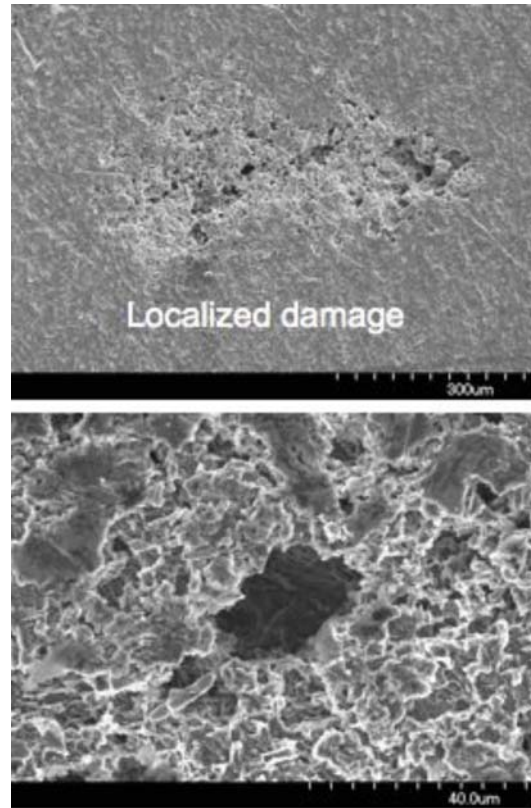
Fig. 2. Scanning electron microscopy of the damage resulting from impacts of 0.1 vol % CuO nanoparticles impacting at 7.7 m/s and 30°
