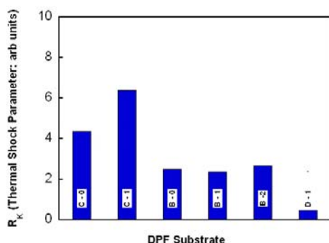
Figure 13. Comparison of the R_K , thermal shock parameter for the DPF substrates. The values are based on the average CTE (average of parallel and perpendicular values), room temperature modulus and average fracture toughness values.
