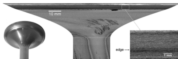
Figure 3. Laser-scatter scan image of \text{Si}_3\text{N}_4 intake valve I2 after 500-h engine test.
