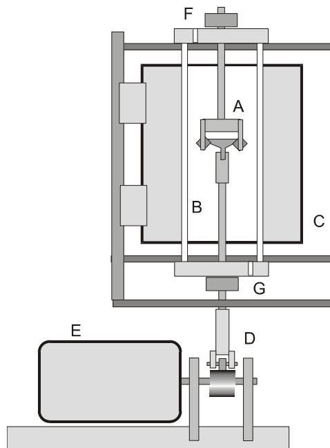
Figure 1. Schematic representation showing the major parts of the HTRI.
