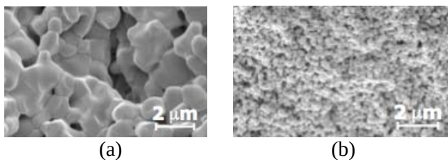
Figure 1. SEM pictures of (a) rectangular porous YSZ slab and (b) fired YSZ slurry on top of wires.
