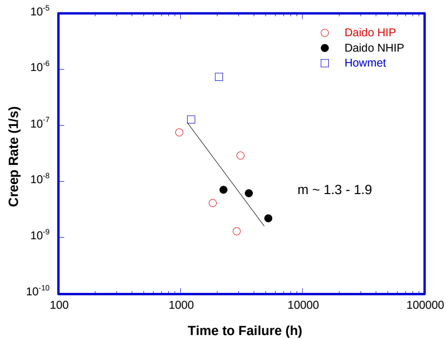
Figure 9. Monkman-Grant creep rate versus lifetime curve of all of the TiAl alloys evaluated.
