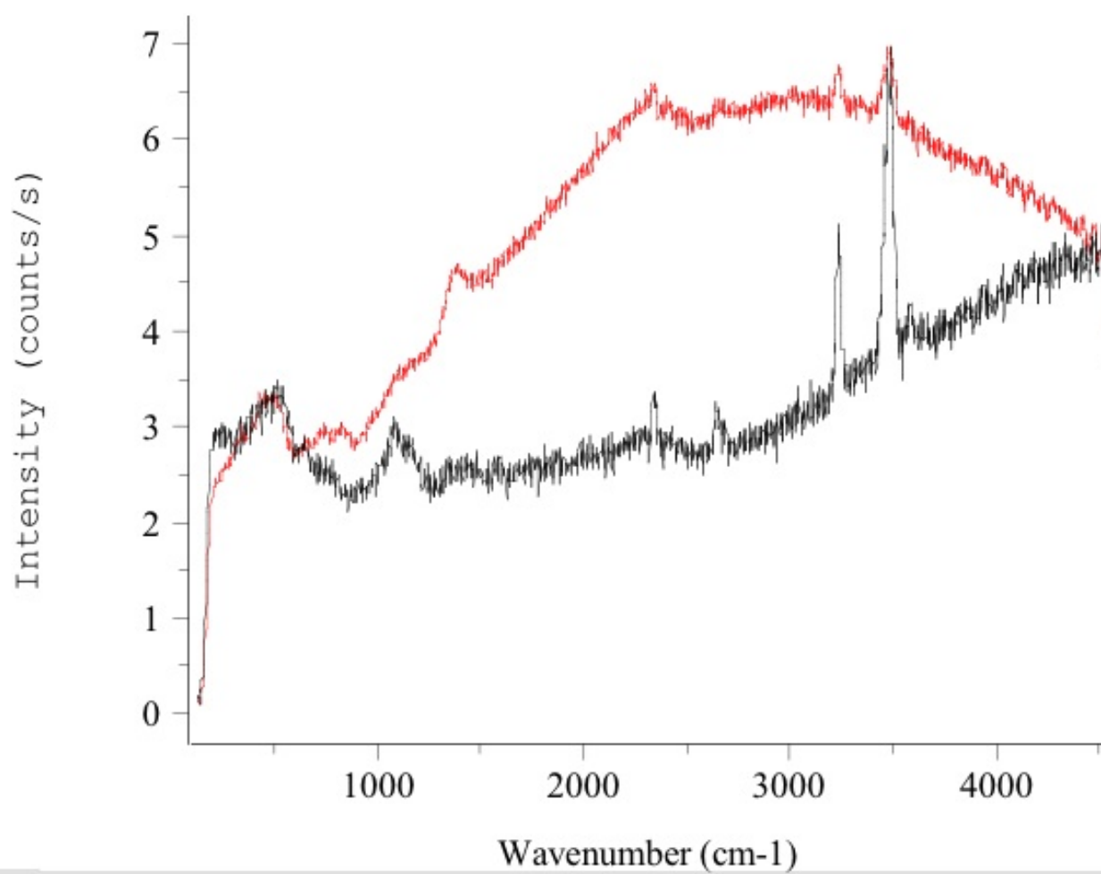
Figure 10. Raman spectra from the zeolite sample degreened at 500°C (black) and 1100°C (red).
