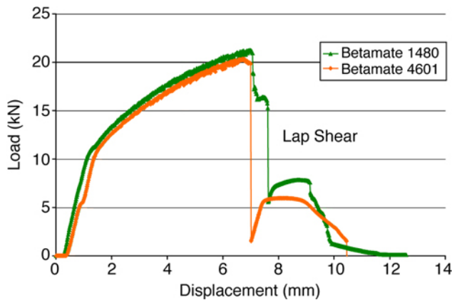
Figure 9. Bond strength test results for Dow Betamate 4601 and Betamate 1480 joining 2 mm AA5182-O to 1.6 mm DP600.
