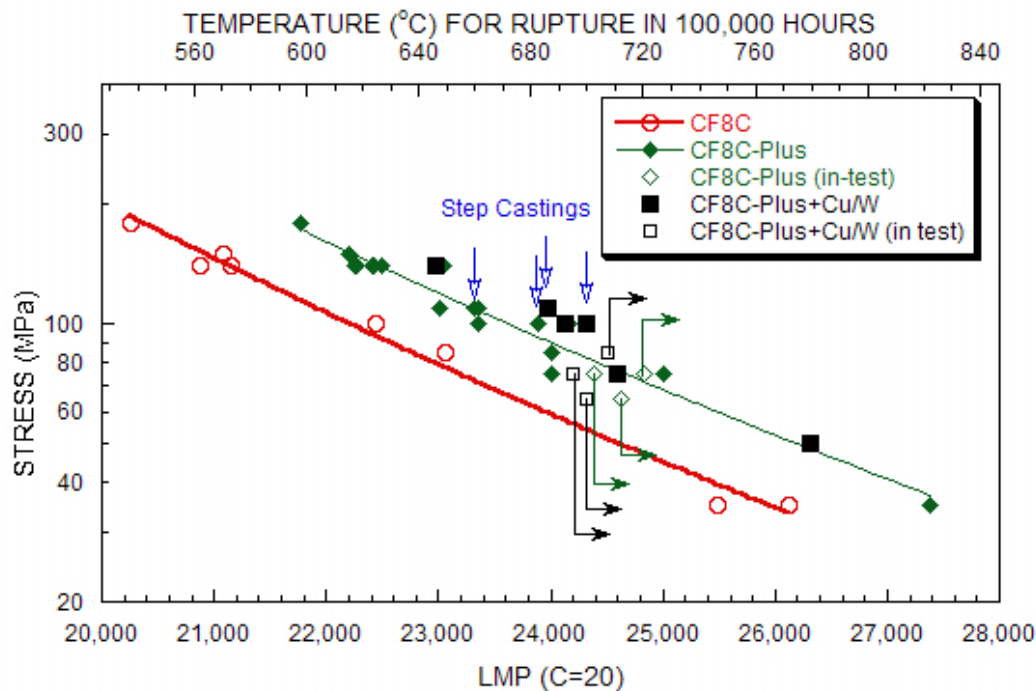
Figure 3. Creep-rupture stress plotted vs LMP for various ORNL creep-rupture tests at 500–850°C in air of various commercial heats of standard CF8C, CF8C-Plus and CF8C-Plus Cu/W stainless steels. New creep data on thin sections of CF8C-Plus and CF8C-Plus Cu/W show similar or better creep-strength compared to previous data on much thicker cast sections.
