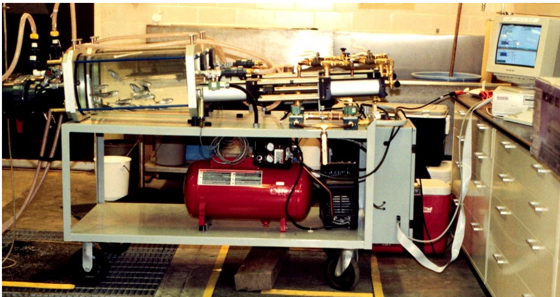
Figure 3.2. Turbine Passage System with Rainbow Trout in Hyperbaric Chambers
