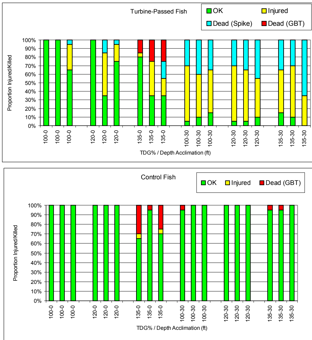
Figure 4.10. Comparison of the Injury and Mortality Rates for Bluegills Based on TDG Level, Acclimation Depth, and Pressure Spike from Turbine Passage
