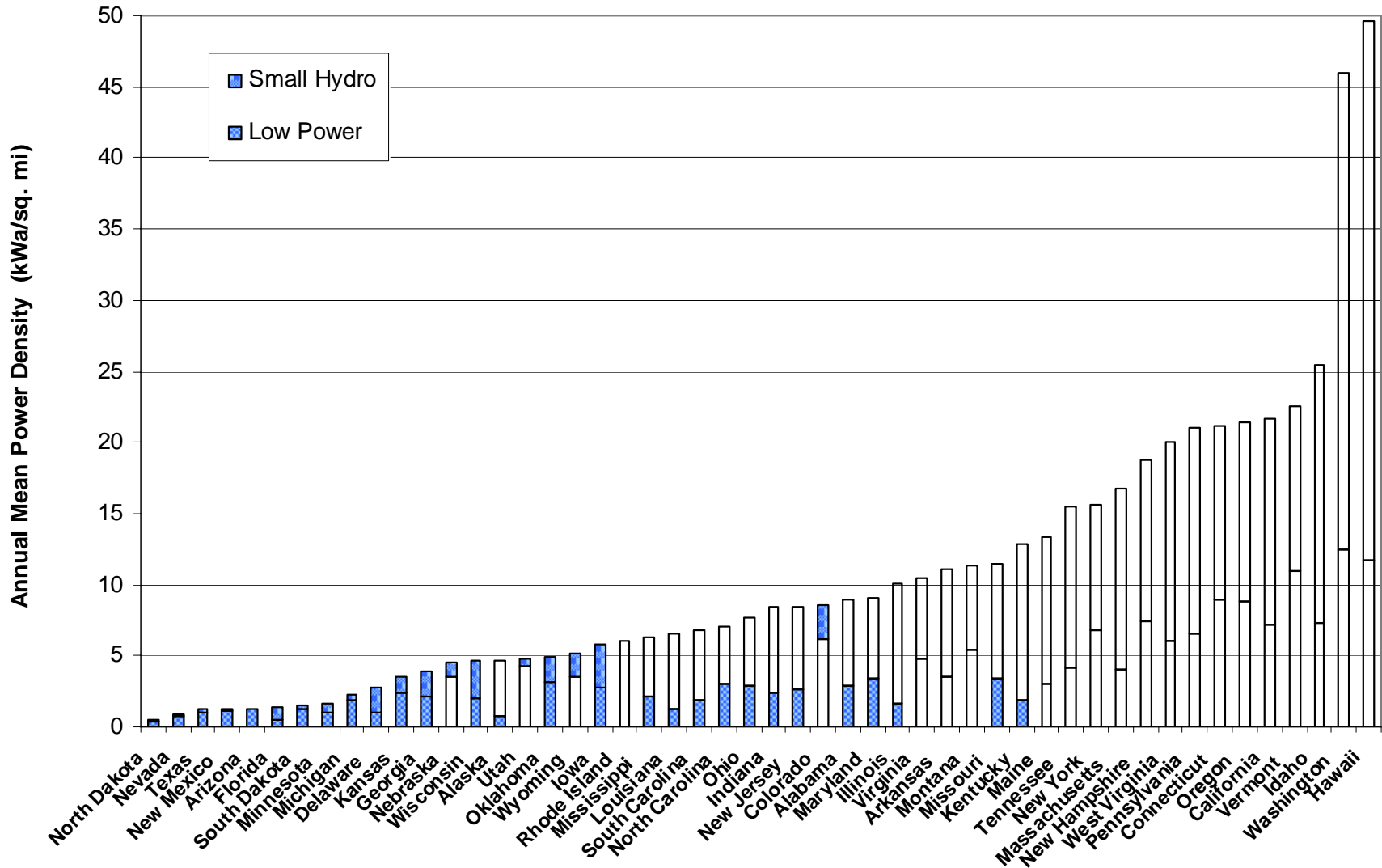
Figure 19. Total hydropower potential density of feasible low power and small hydro projects in the 50 states of the United States.
