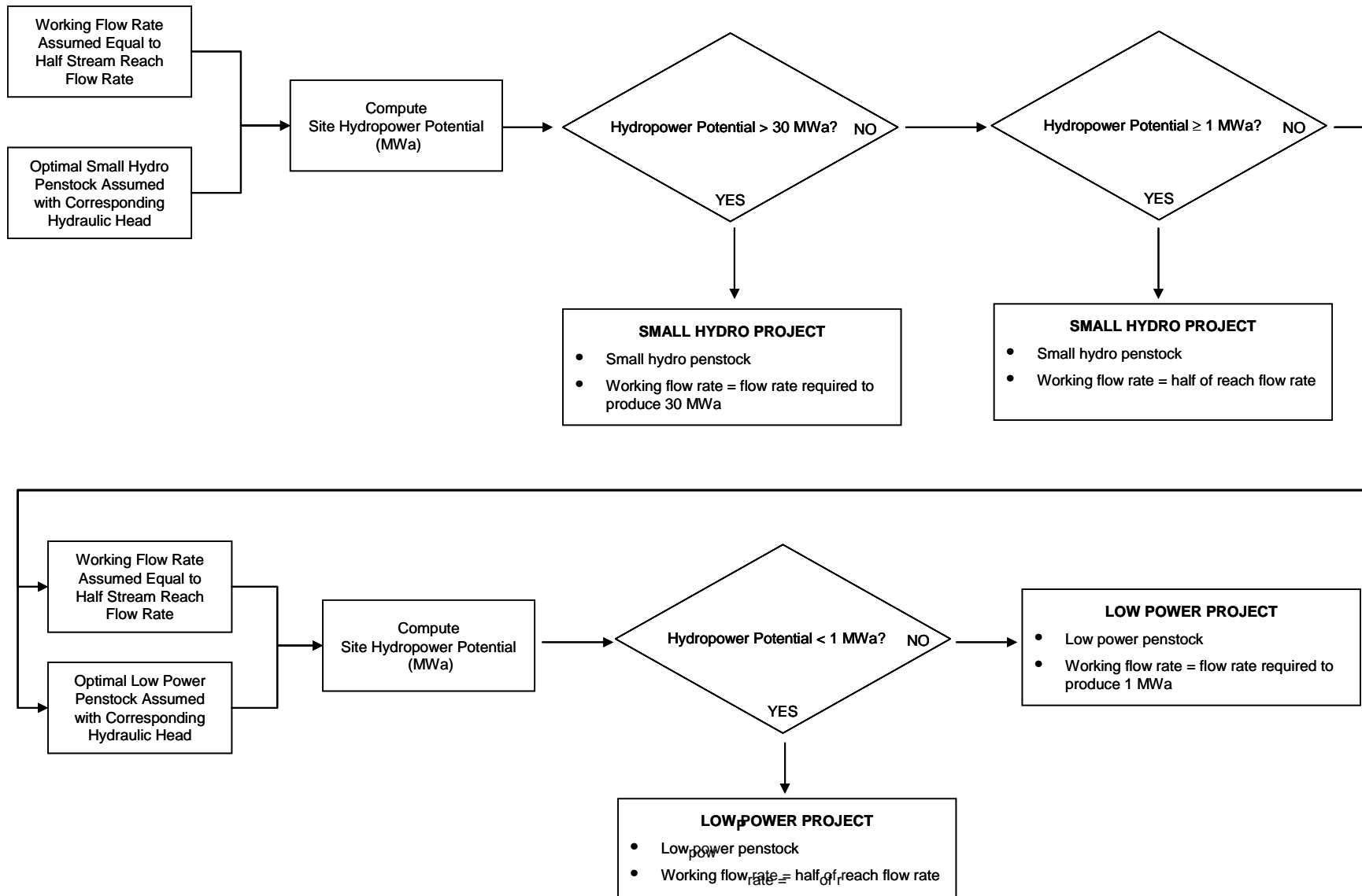
Figure 9. Logic for determining whether a water energy resource site should be developed as a low power or small hydro project using development criteria thereby establishing working flow rate, penstock length, working hydraulic head, and hydropower potential.
