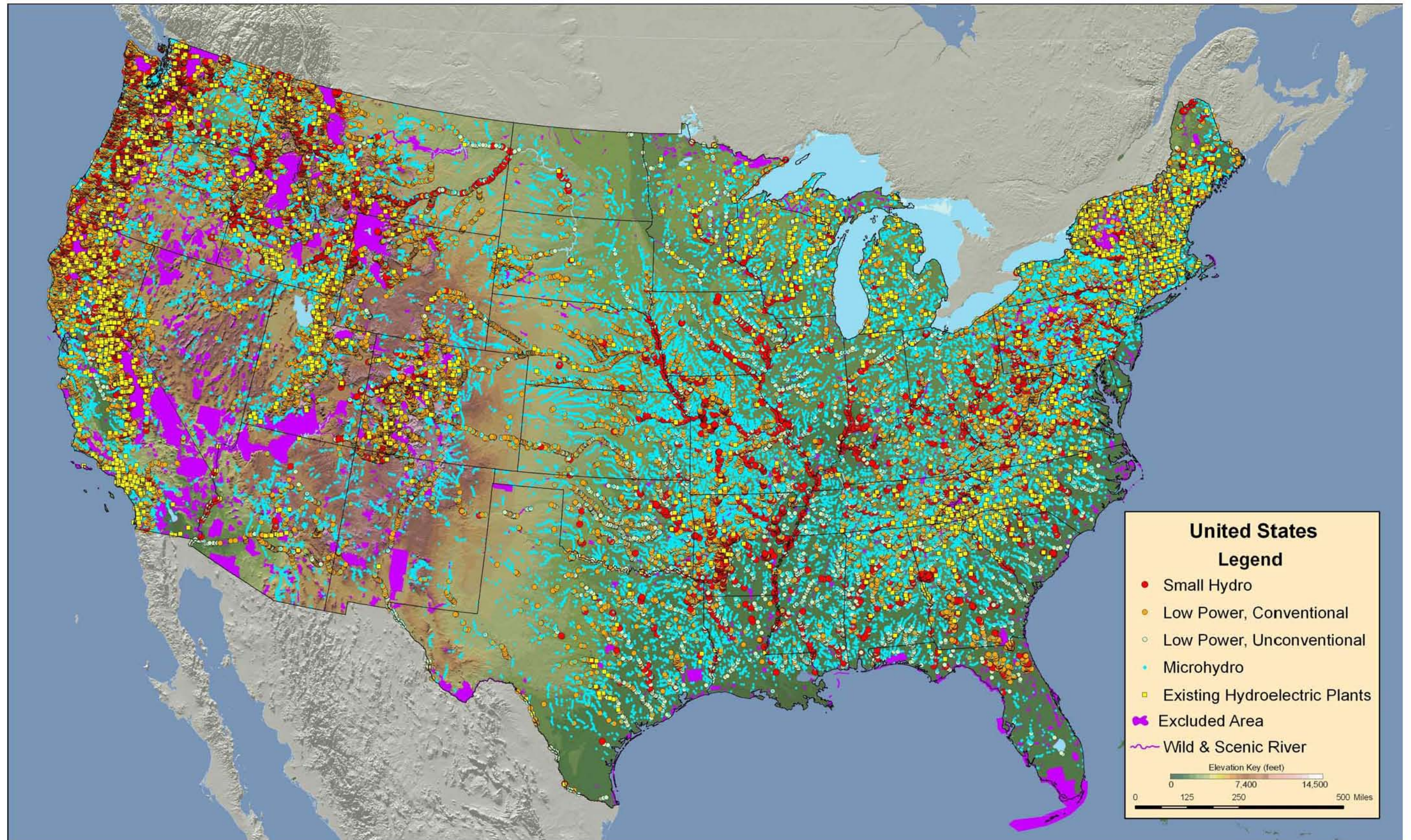
Figure 20. Existing hydroelectric plants and feasible potential hydropower projects in the United States.
