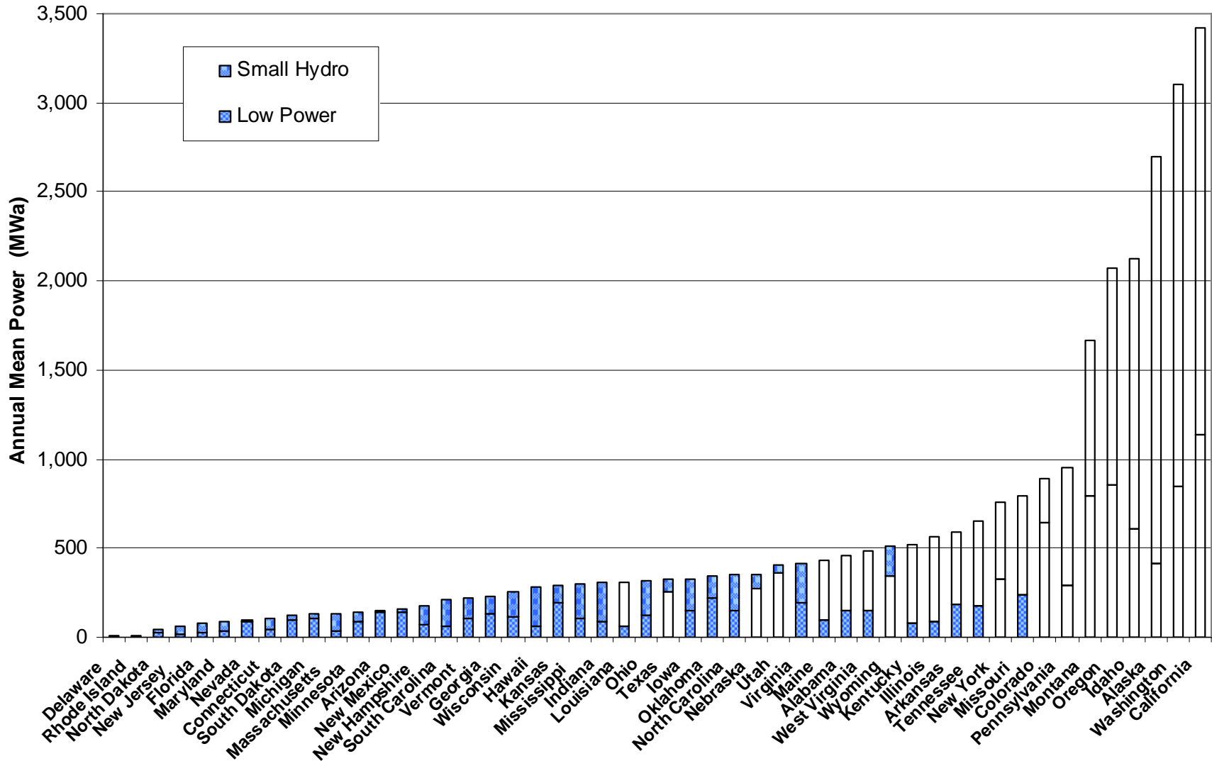
Figure 18. Total hydropower potential of feasible low power and small hydro projects in the 50 states of the United States.
