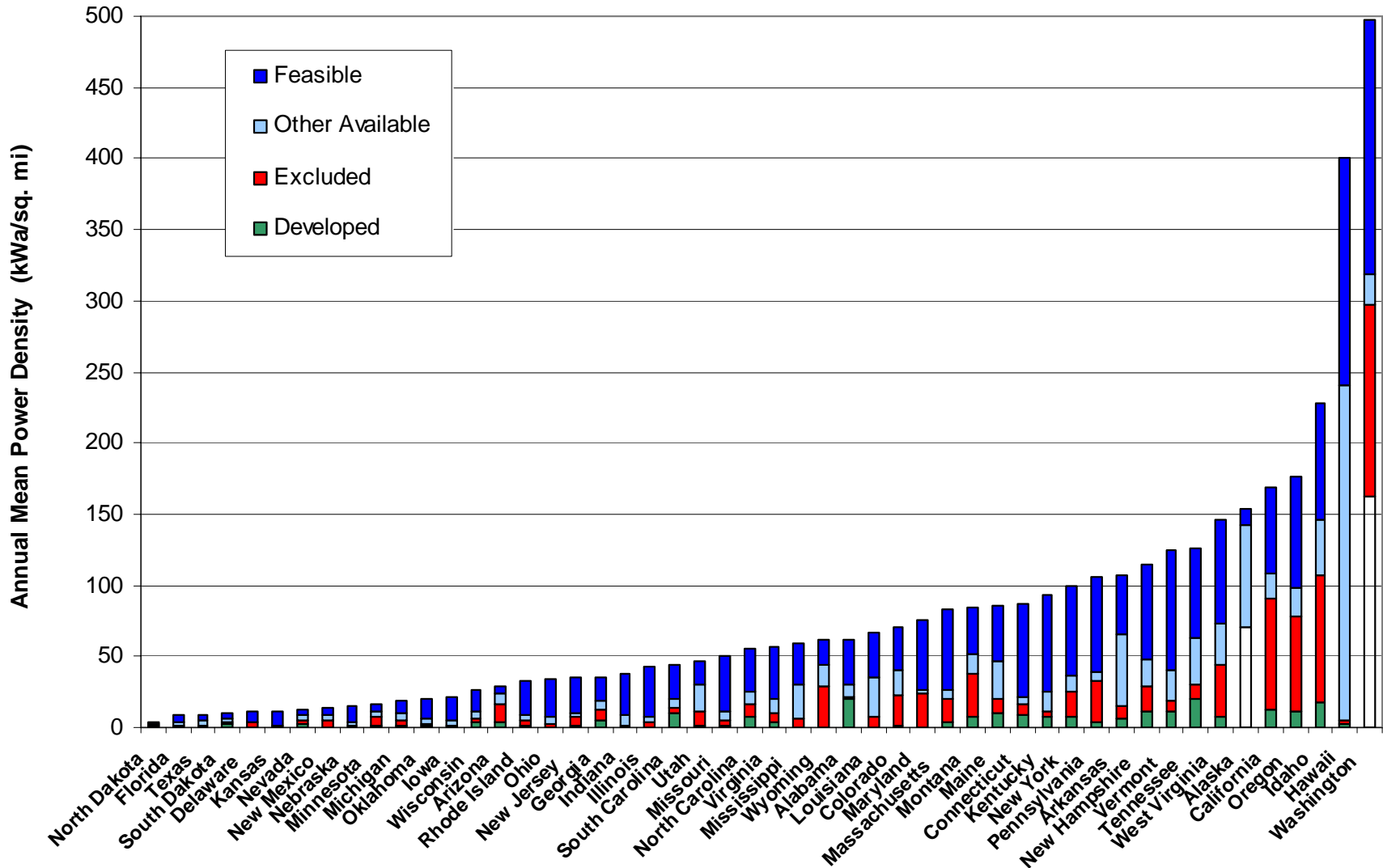
Figure 17. Total gross power potential density of water energy resources in the 50 states of the United States divided into feasible, other available, excluded, and developed power categories.
