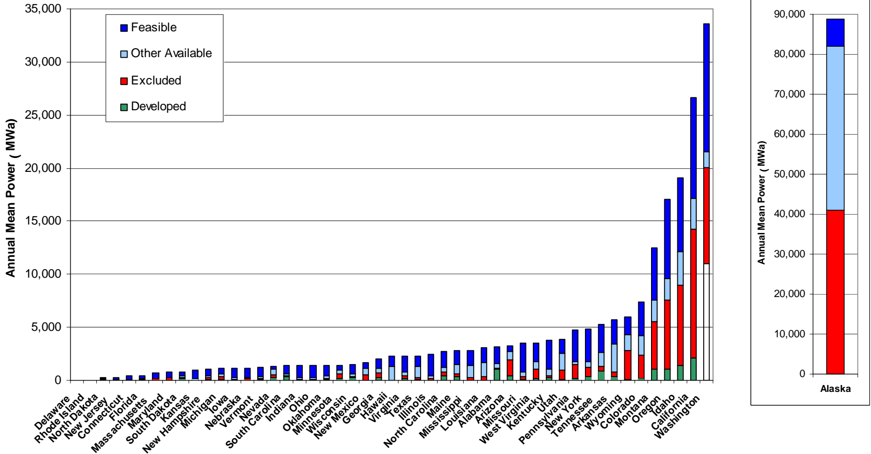
Figure 16. Total gross power potential of water energy resources in the 50 states of the United States divided into feasible, other available, excluded, and developed power categories.
