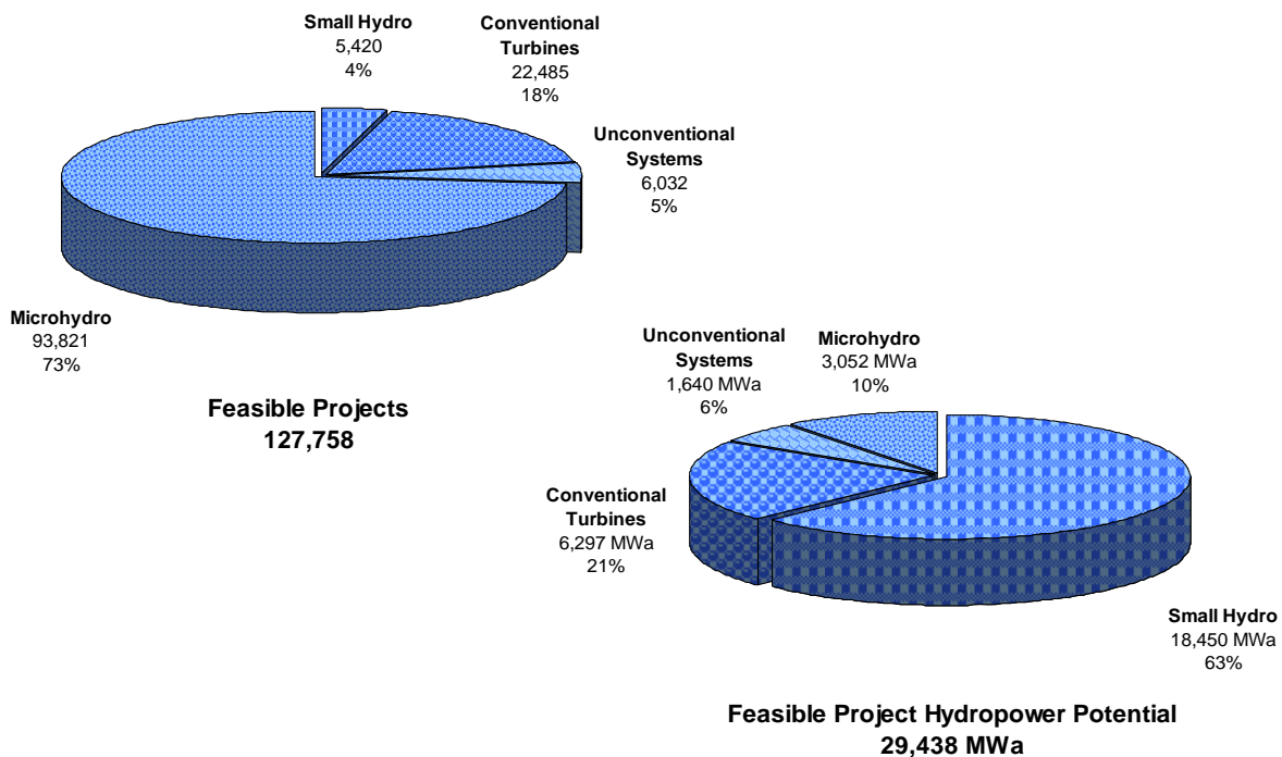
Figure 13. Power category distribution of feasible potential projects and their associated total hydropower potential with low power projects further divided by low power technology classes.
