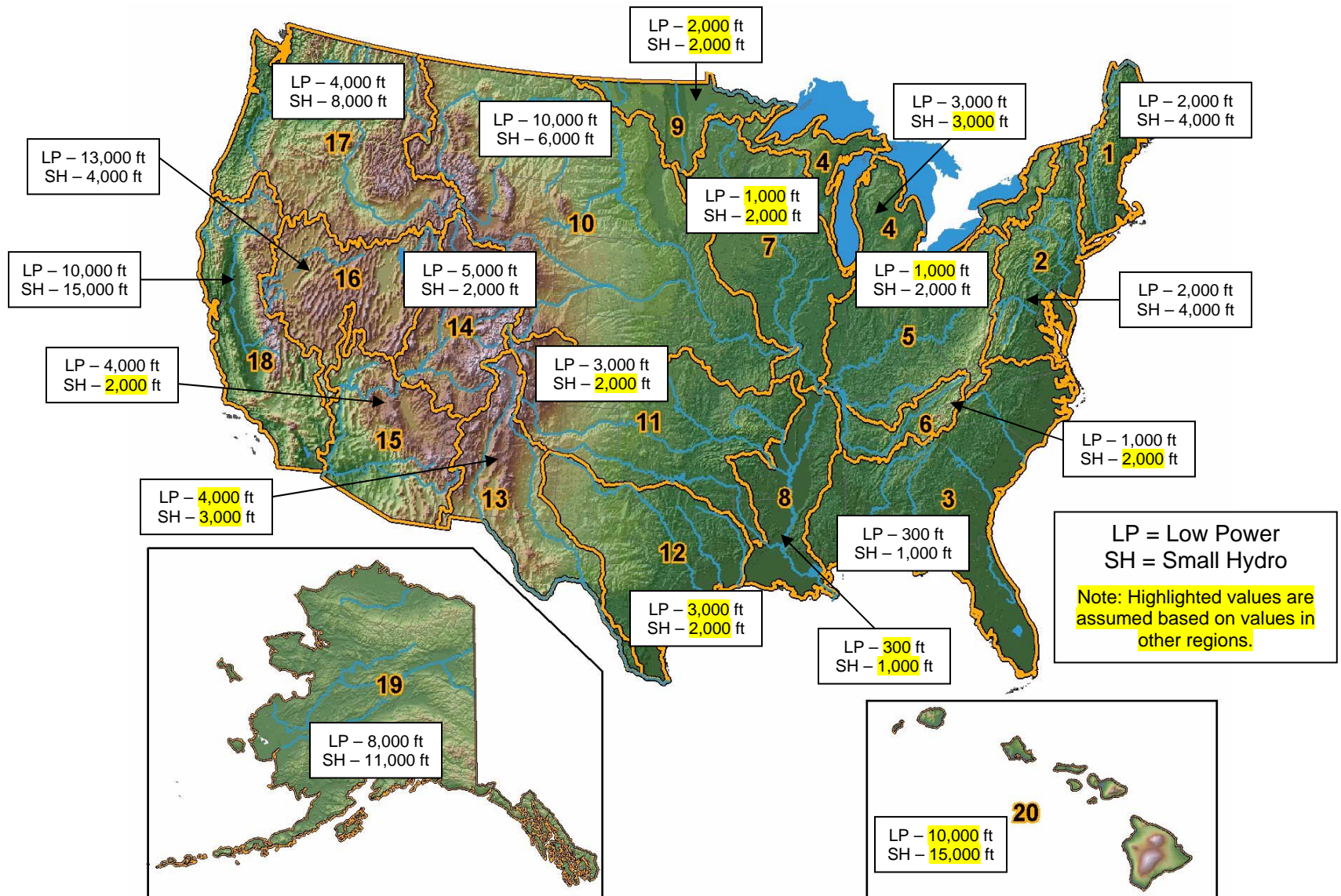
Figure 8. Penstock length upper limits for low power and small hydro plants in 20 U.S. hydrologic regions.
