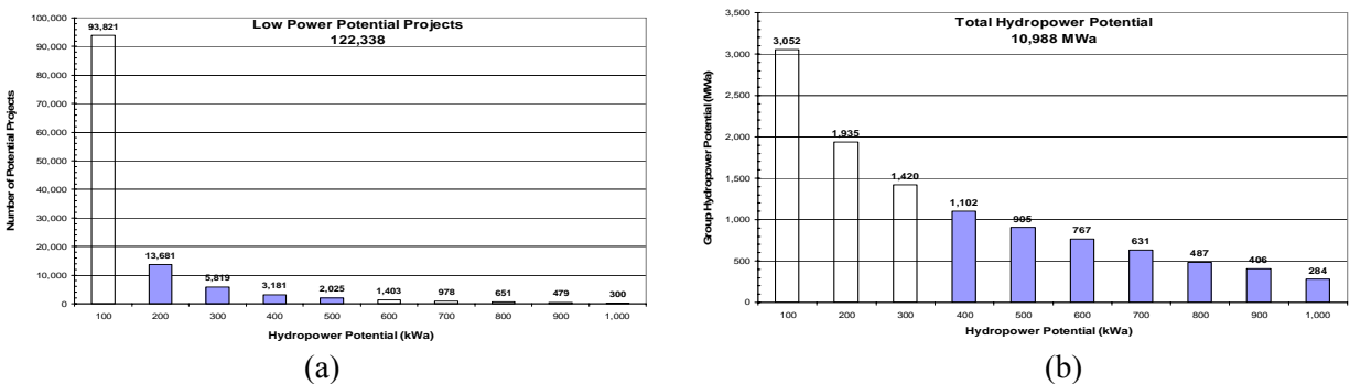
Figure 14. Distribution of (a) number and (b) group hydropower potential of U.S. low power potential projects.
