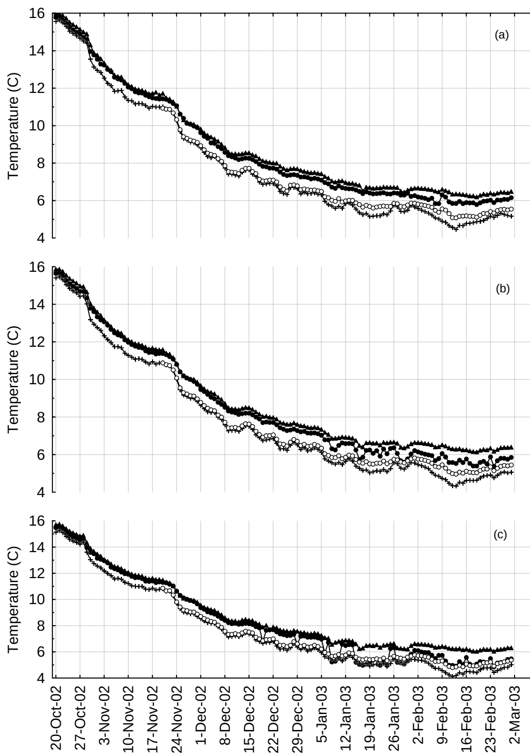
Figure 36. Daily maximum (a), average (b), and minimum (c) temperature of the river (+), egg pocket (○), shallow hyporheic (●) and deep hyporheic (▲) zones at site 218.7.
