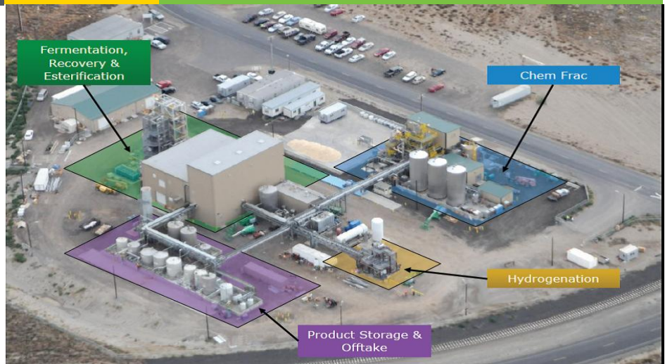
ZeaChem's 250,000 gallon per year integrated biorefinery finalizing construction in 2013.
