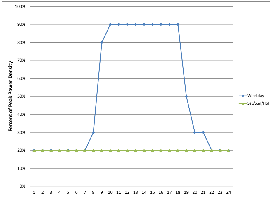
Figure 4.2.5 Small Office Plug Load Schedule
