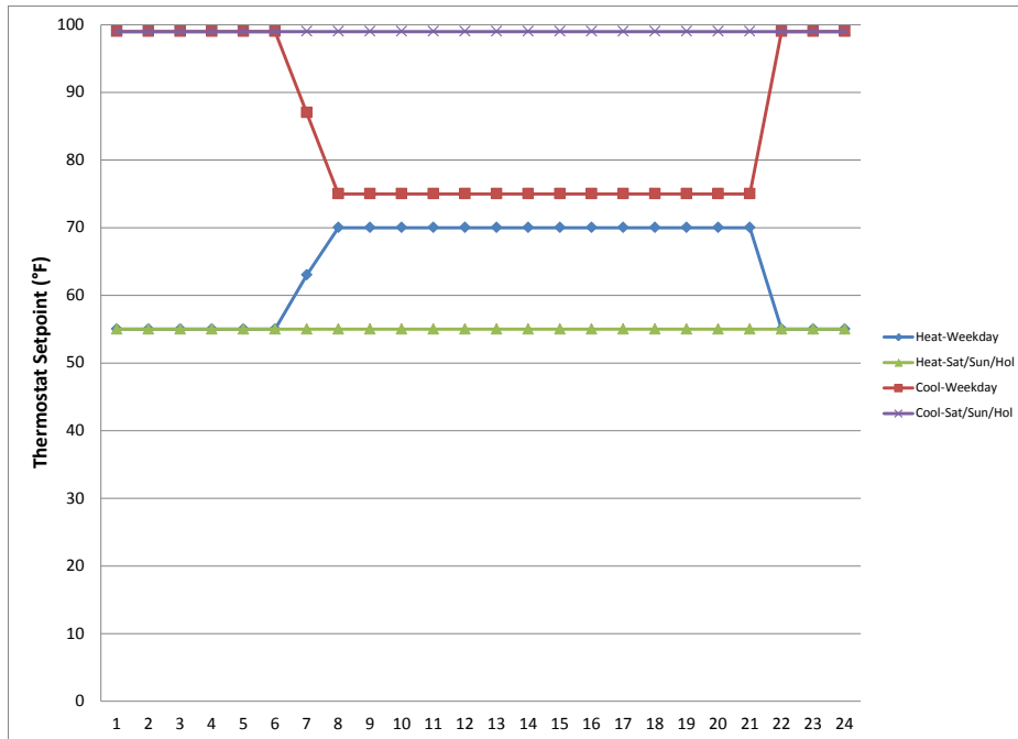
Figure 4.2.7 Small Office Thermostat Set Point Schedule
