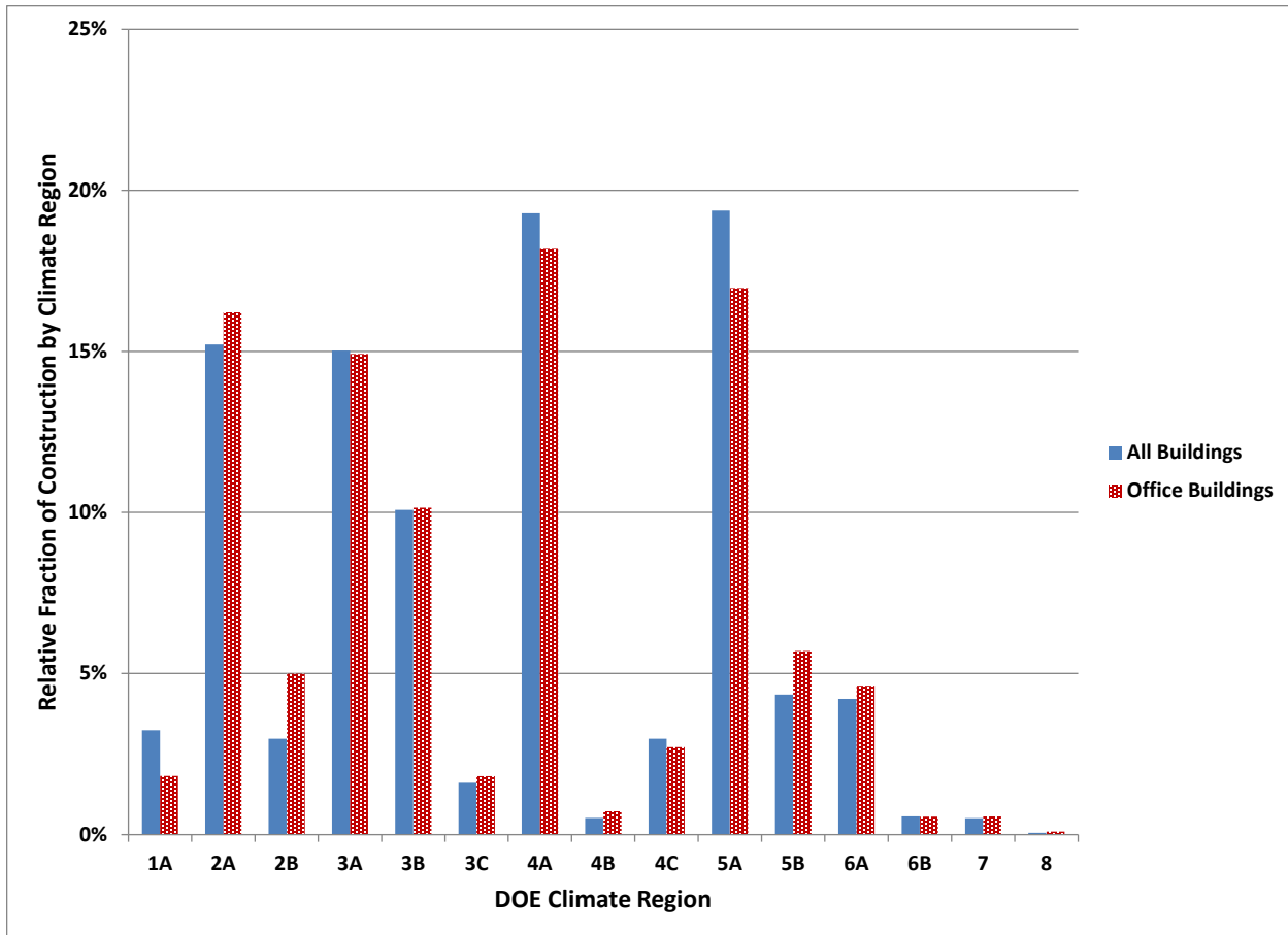
Figure 4.2.1 Comparison of Floor-Space Weighting Factors by Region, Small and Medium Office Buildings versus All Buildings
