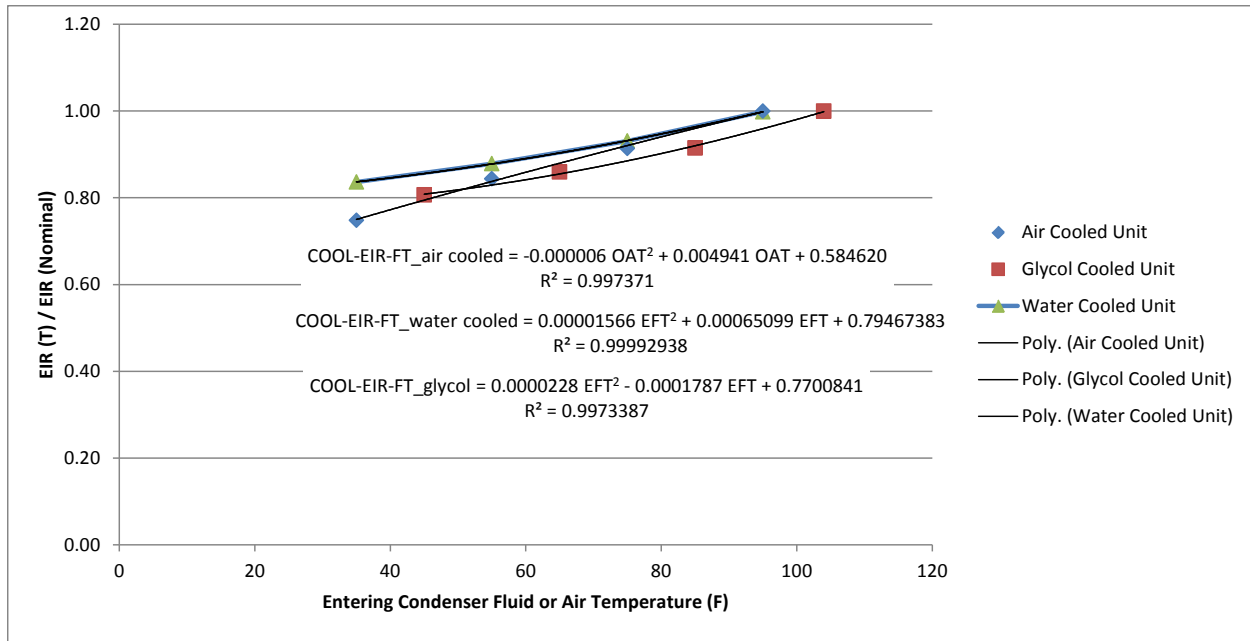
Figure 4.2.2 Cooling EIR as a Function of Entering Condenser Fluid Air Temperature
