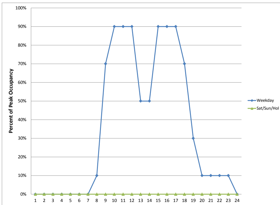
Figure 4.2.6 Small Office Occupancy Schedule
