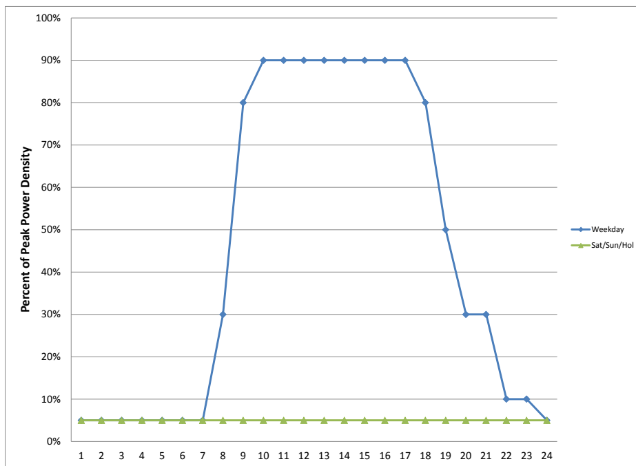
Figure 4.2.4 Small Office Lighting Schedule
