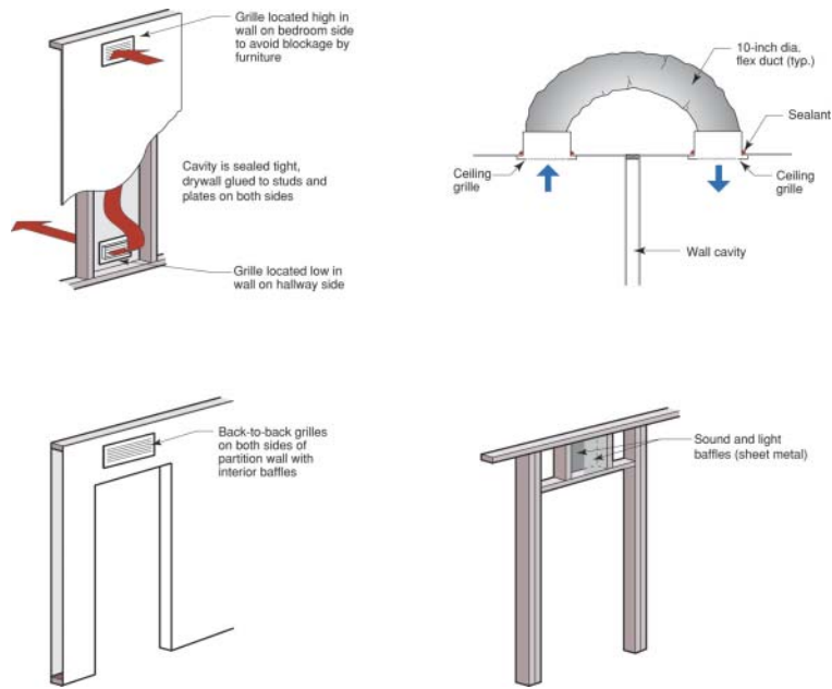
Figure 40. Transfer grille and jump duct approaches
