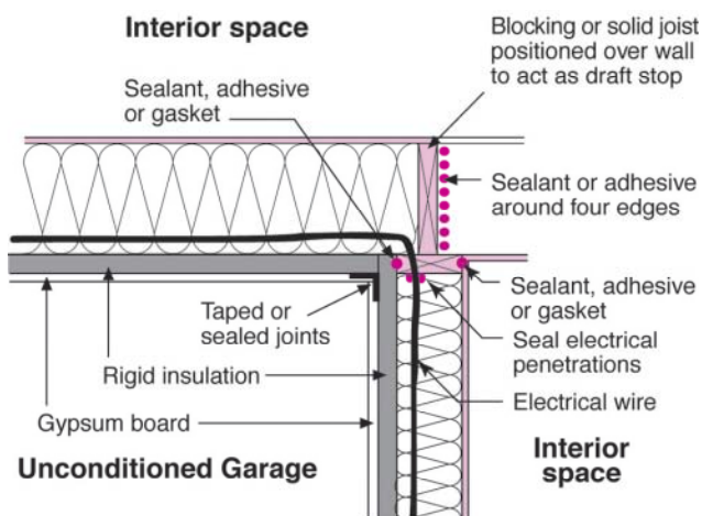
Figure 2. Creating a continuous air barrier
