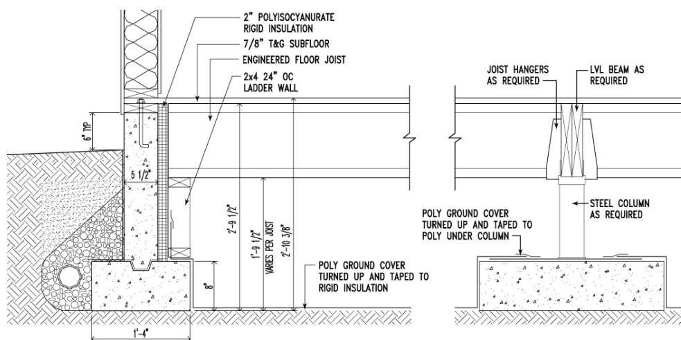
Figure 63. Conditioned crawlspace
