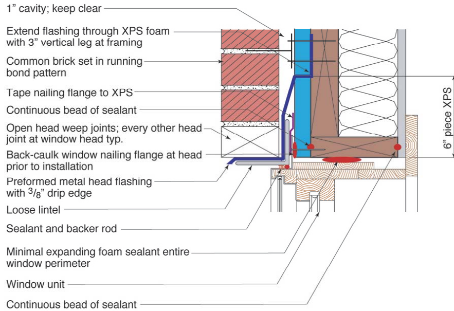
Figure 45. Rough opening flashing
