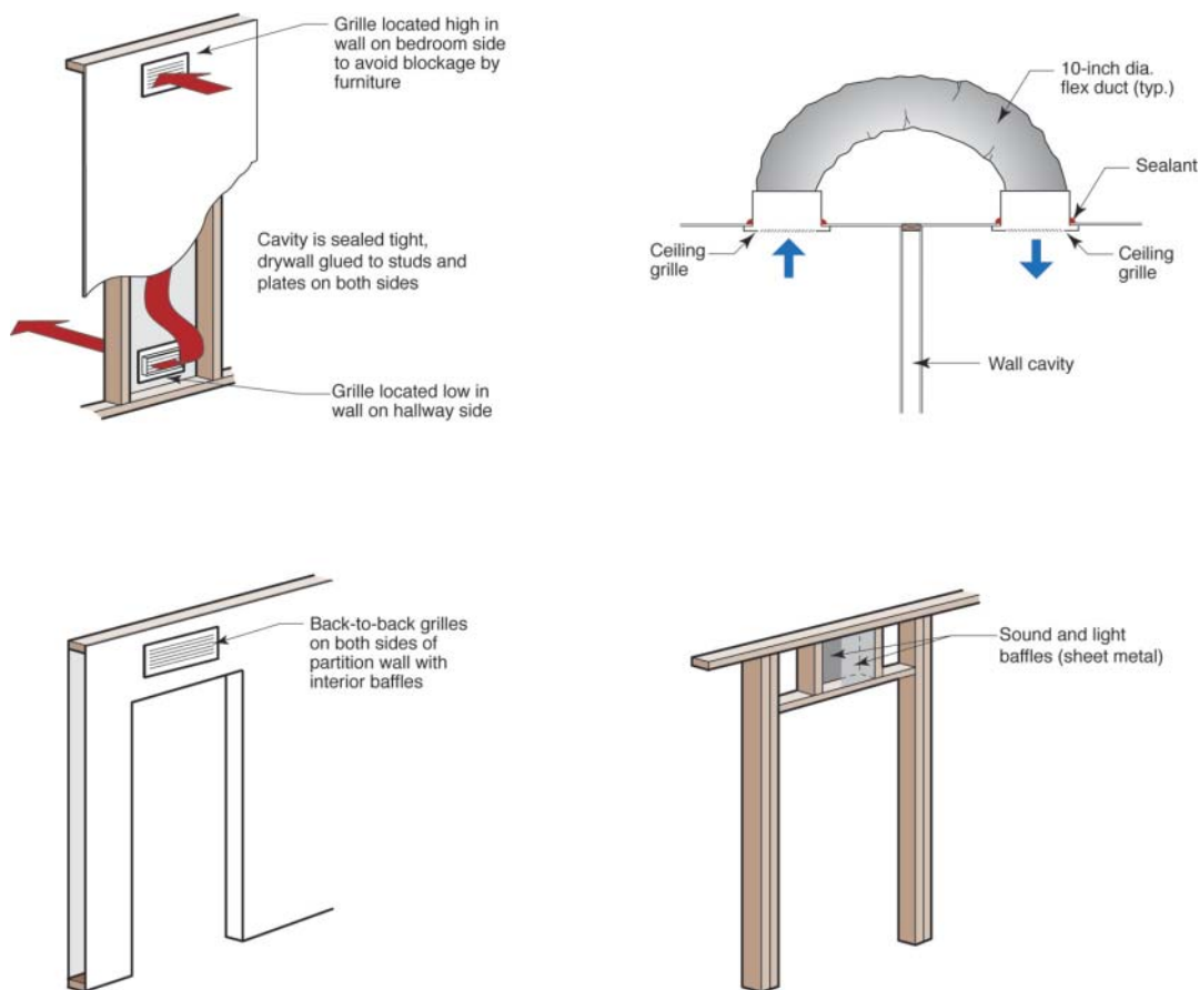
Figure 6. Transfer grilles and jump ducts
