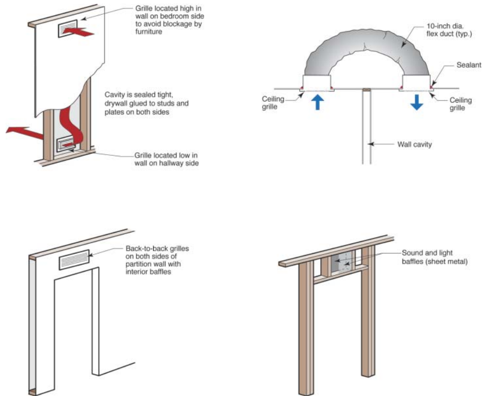
Figure 18. Transfer grilles and jump ducts
