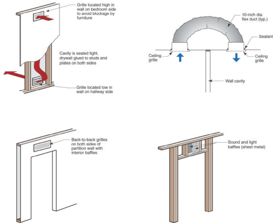
Figure 67. Transfer grilles and jump ducts
