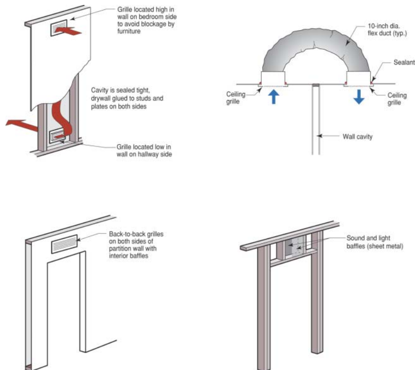
Figure 28. Return grilles
