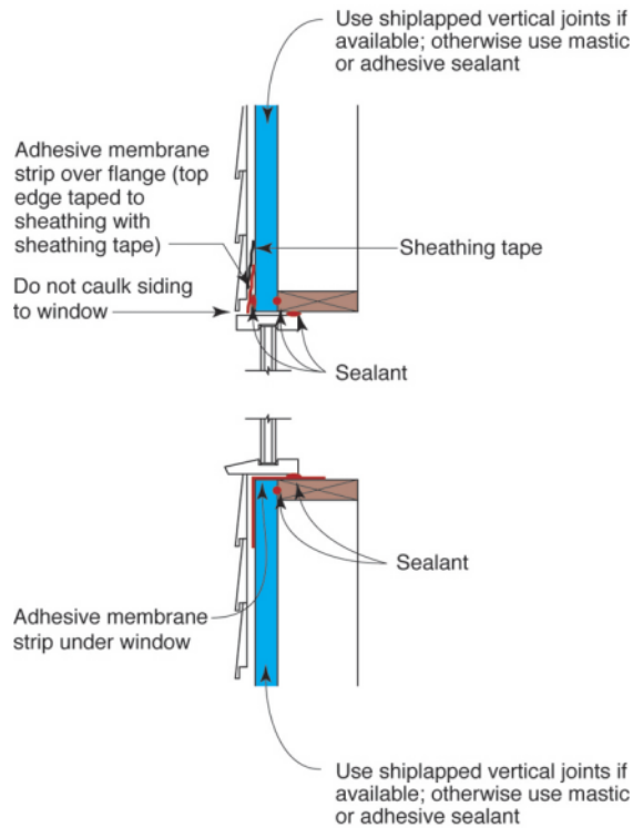
Figure 52. Rough opening flashing
