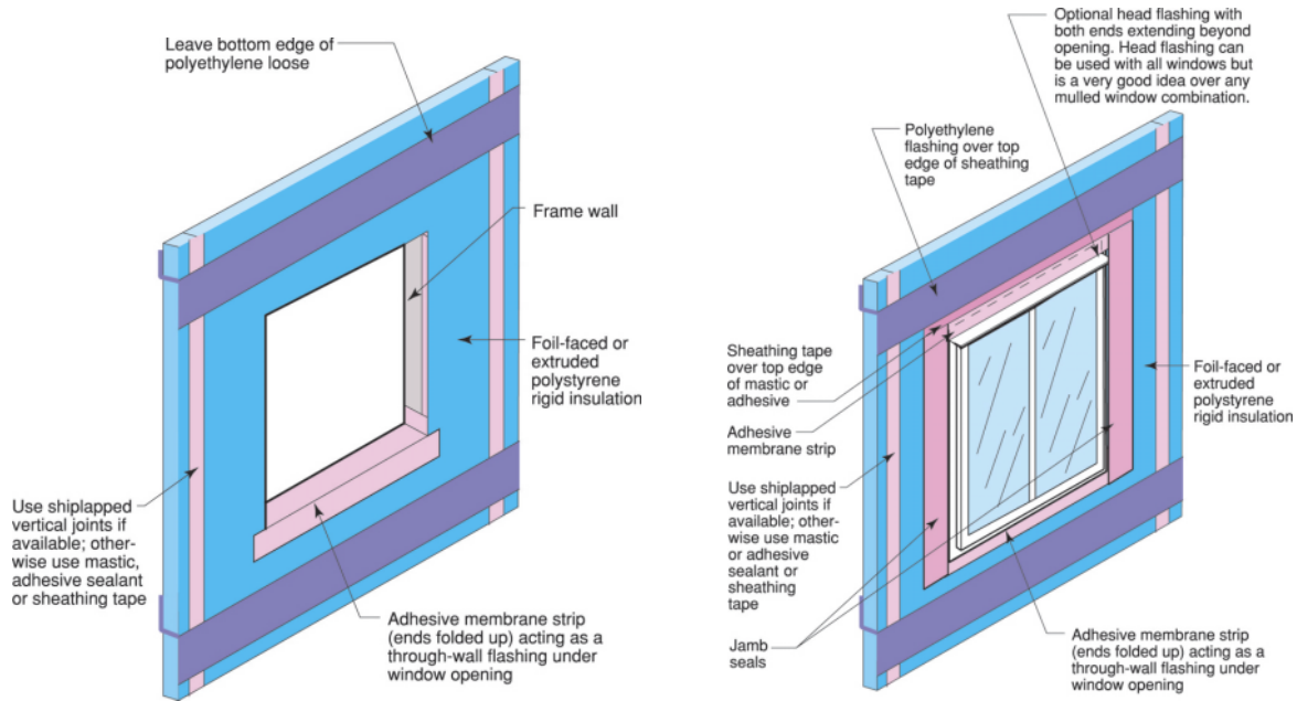
Figure 16. Window flashing
