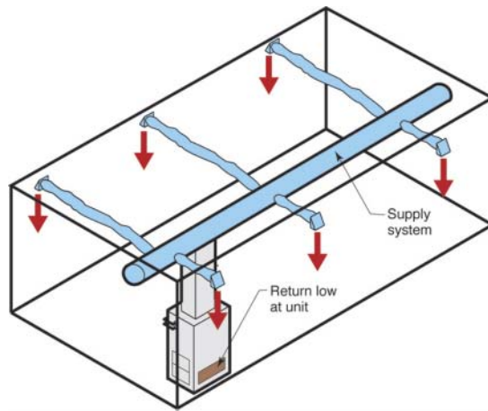
Figure 73. Heating and cooling system layout
