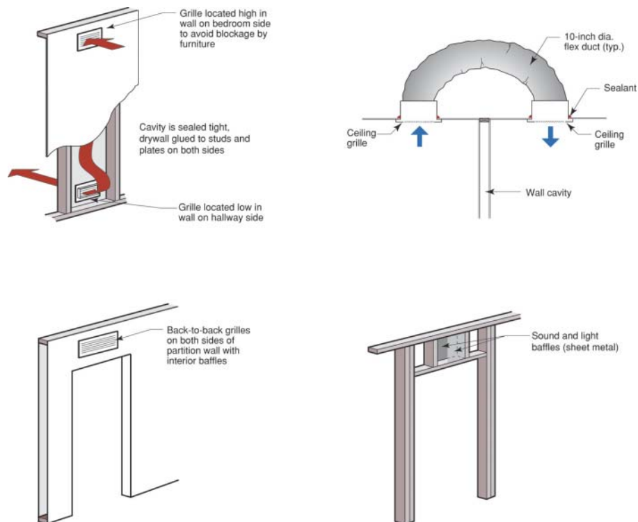
Figure 74. Transfer grilles and jump ducts
