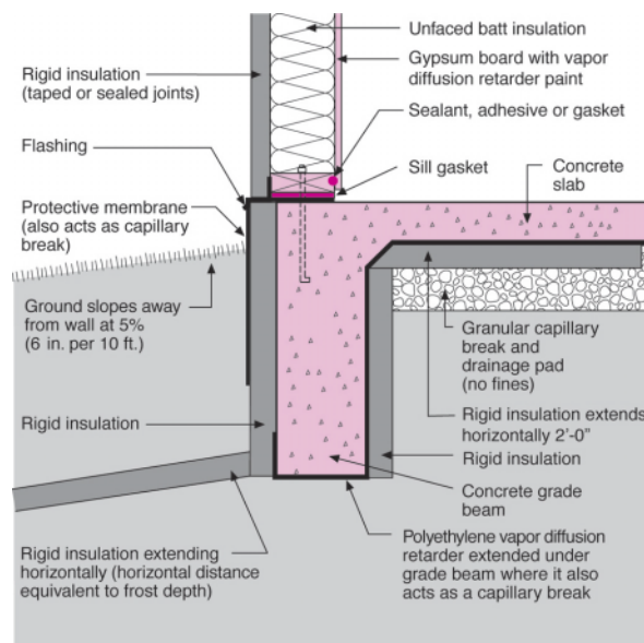
Figure 36. Slab foundation details
