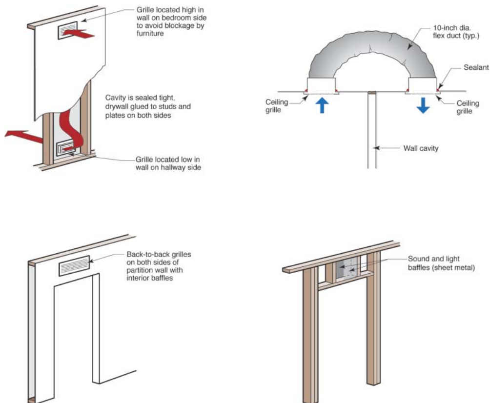
Figure 12. Placement of ducts and transfer grilles
