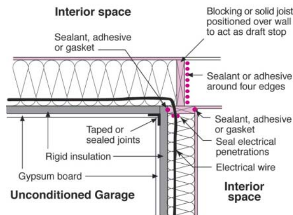
Figure 9. Using sealants and rigid insulation to create a continuous air barrier
