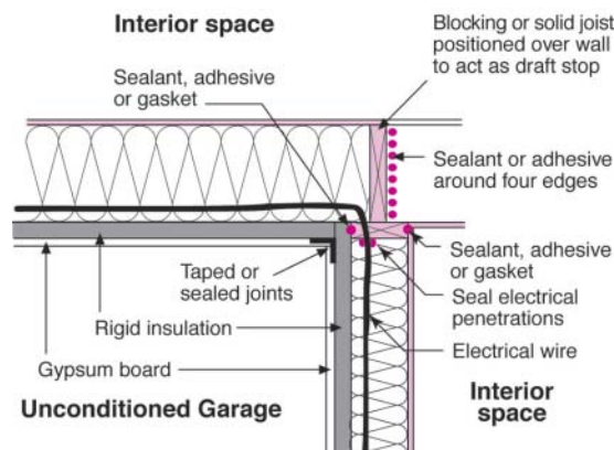
Figure 58. Continuous air barrier
