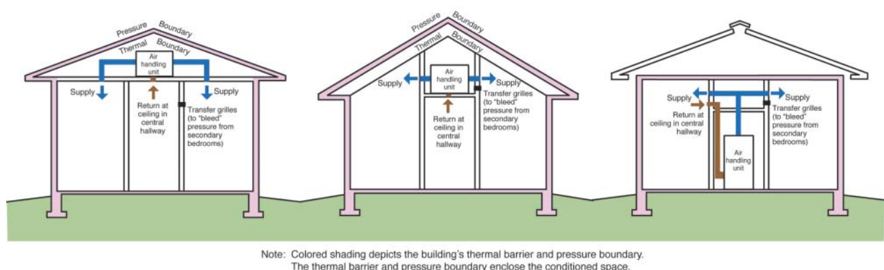
Figure 5. Ducts in conditioned space
