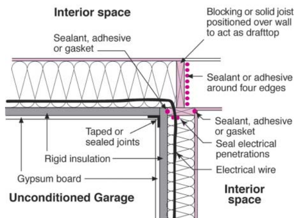
Figure 65. Creating a continuous air barrier
