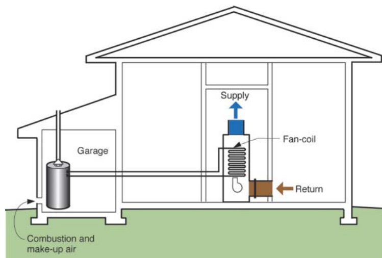
Figure 59. Combo heating system
