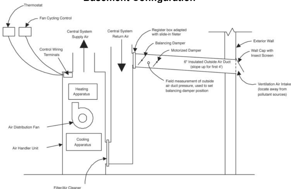
Figure 29. Recommended ventilation system
