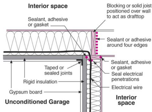
Figure 51. Creating a continuous air barrier
