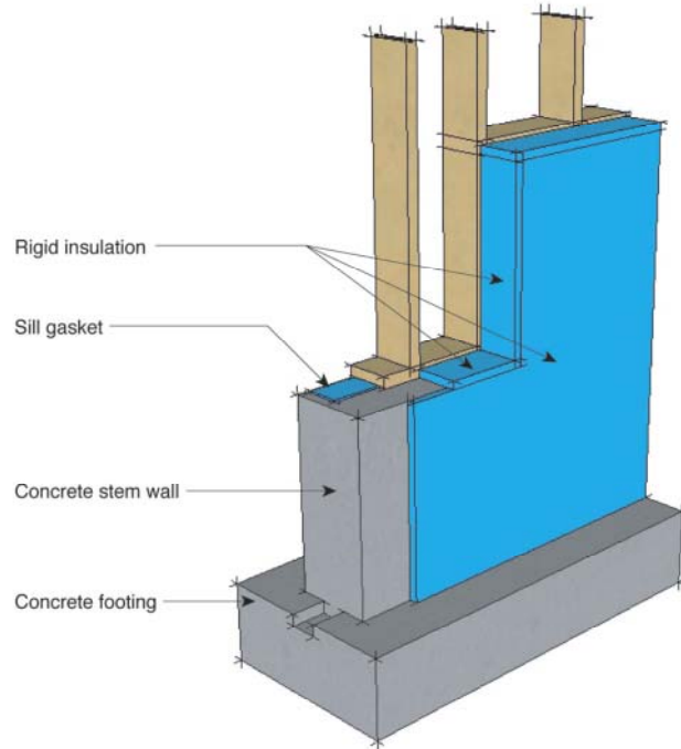
Figure 56. Stepped foundation insulation detail
