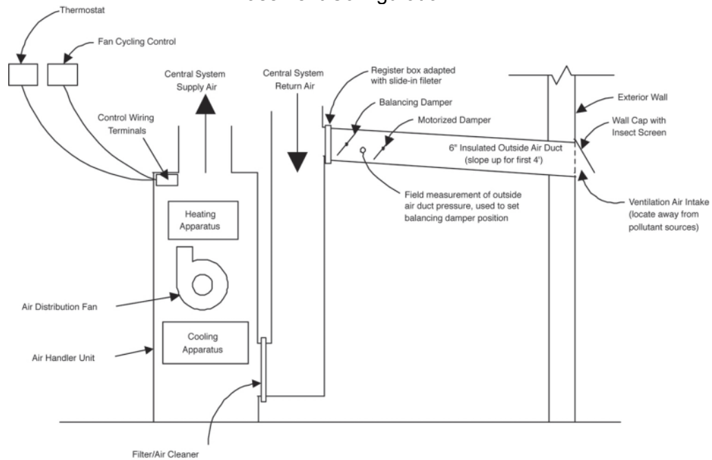
Figure 54. Mechanical ventilation in the “Louisville”
