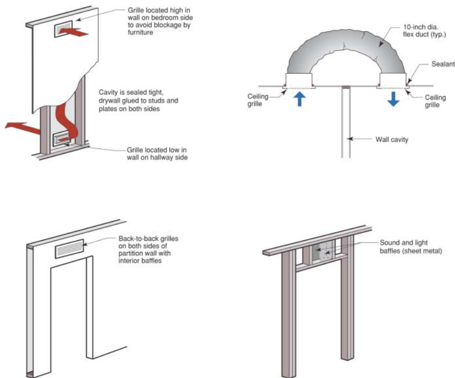
Figure 22. Transfer grille and jump duct approaches
