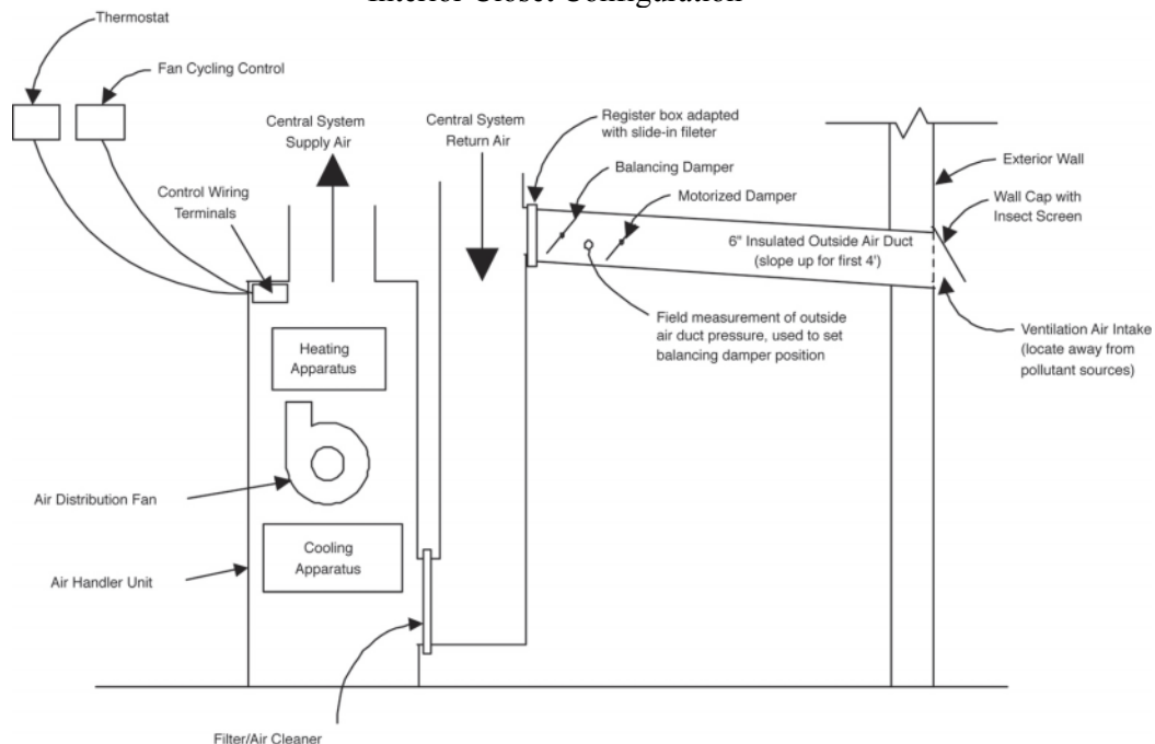
Figure 47. Mechanical ventilation for the “Atlanta”
