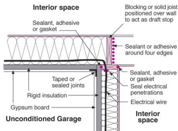
Figure 32. Creating a continuous air barrier
