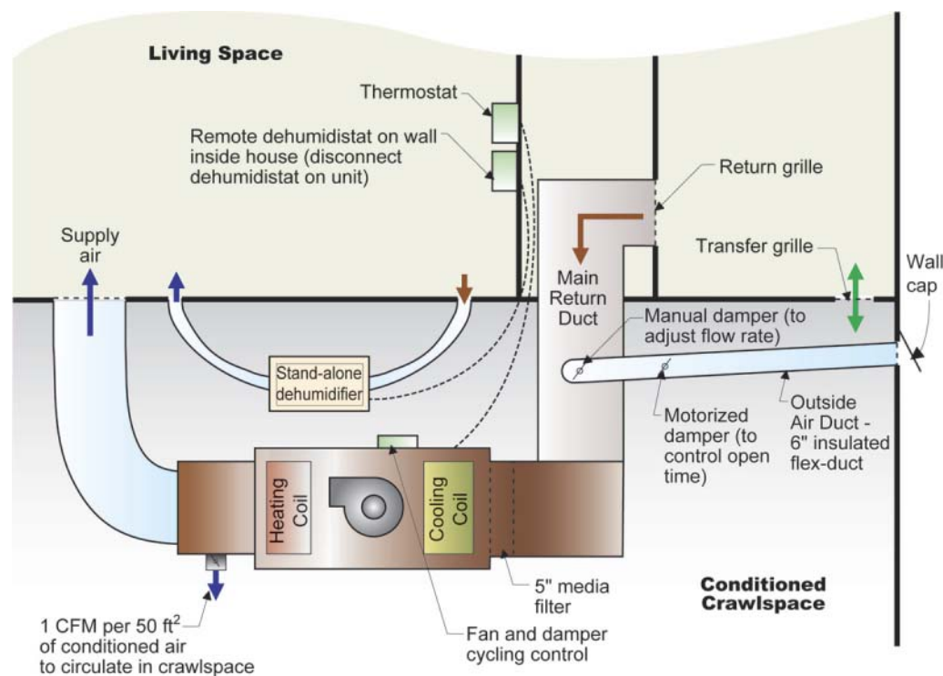
Figure 17. Mechanical system and ventilation in conditioned crawlspace
