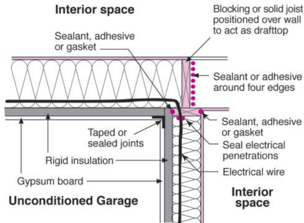
Figure 44. Creating a continuous air barrier
