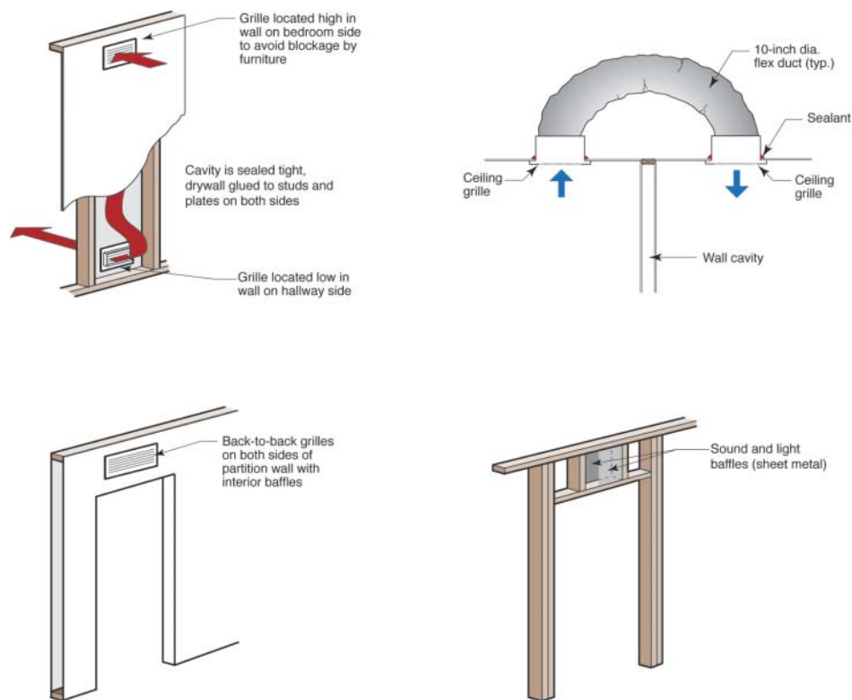
Figure 46. Transfer grille and jump ducts approaches
