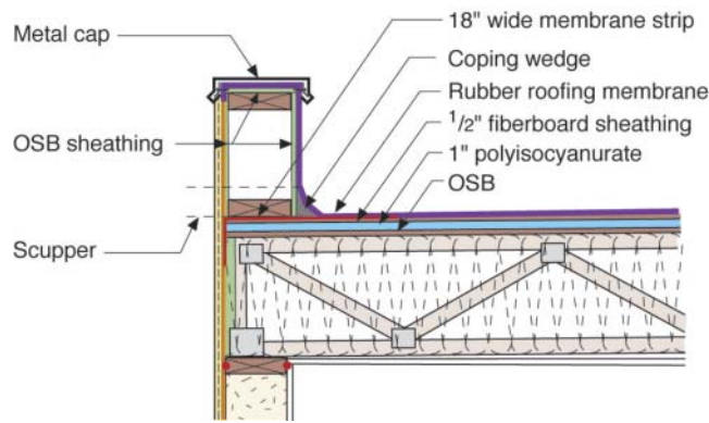
Figure 75. Flat-roof assembly
