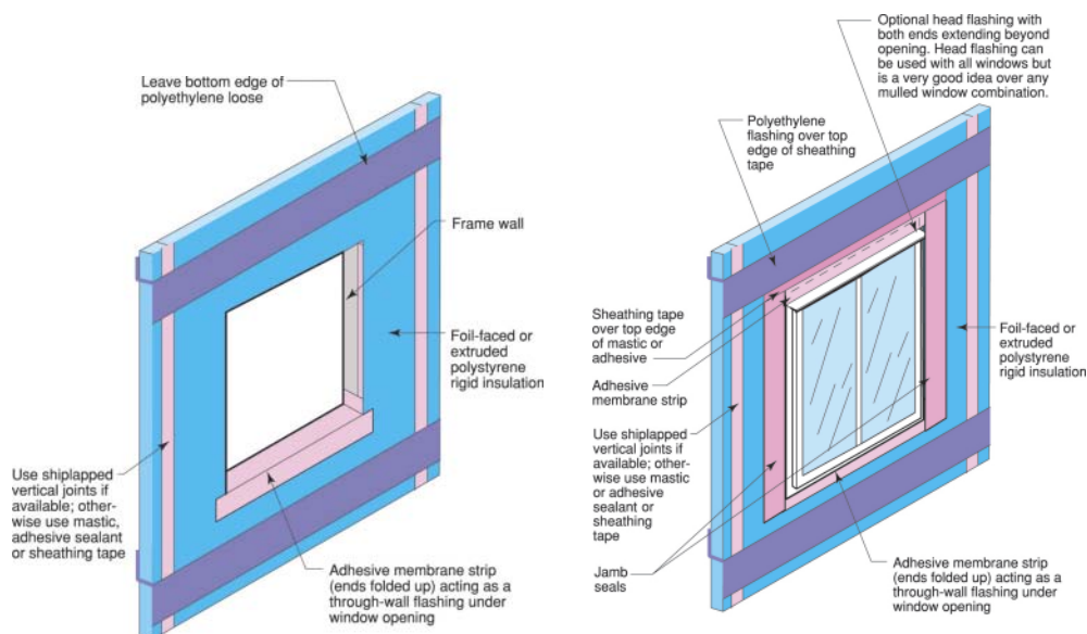
Figure 3. Window flashings
