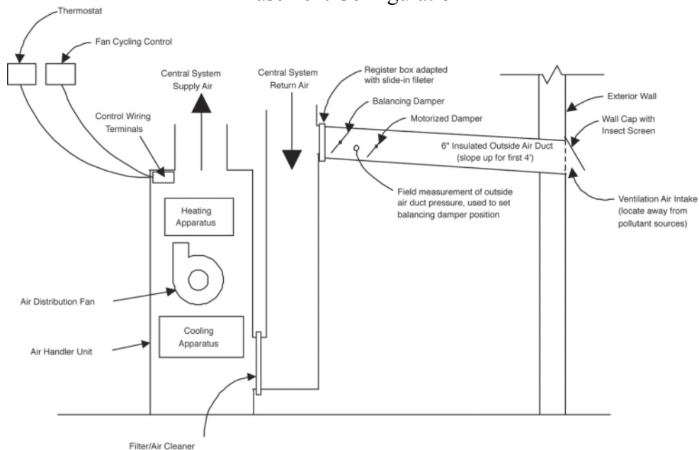
Figure 23. Recommended ventilation system in the “Chicago”
