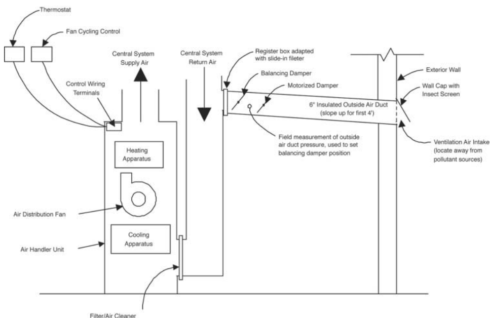
Figure 33. HVAC configuration
