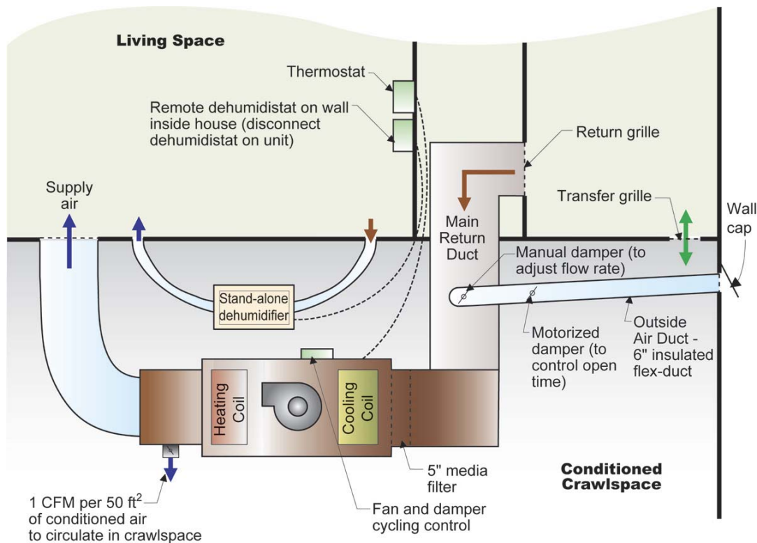
Figure 41. Mechanical system and ventilation in conditioned crawlspace
