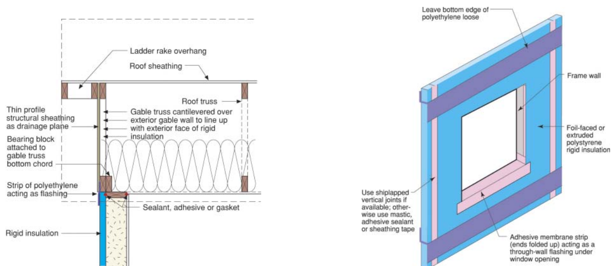
Figure 21. Air sealing and an attached garage.
