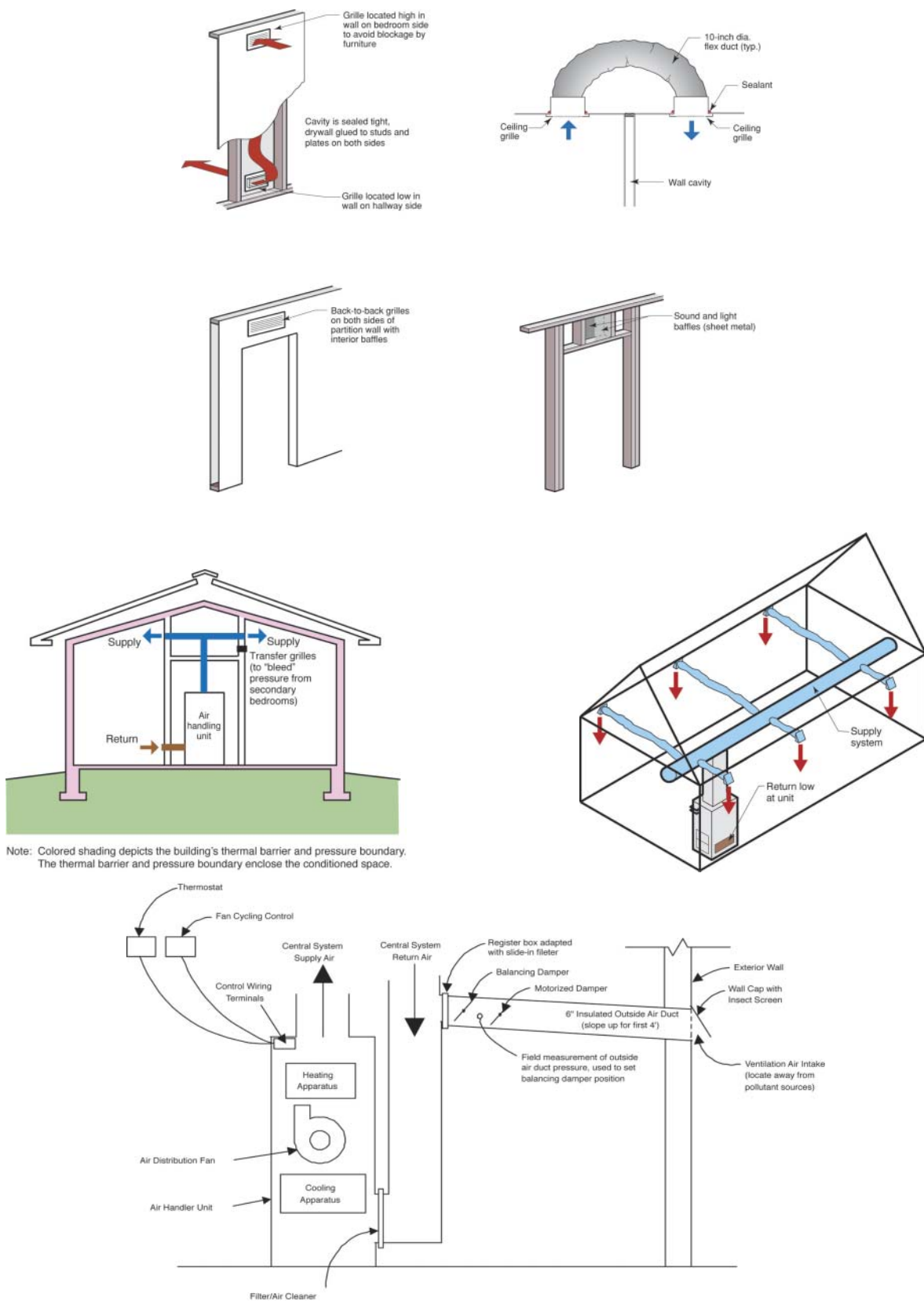
Figure 60. Ducting, transfer grilles, and interior closet configuration
