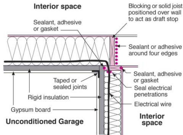
Figure 15. Creating a continuous air barrier
