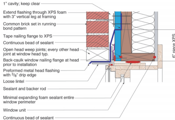
Figure 27. Brick veneer flashing
