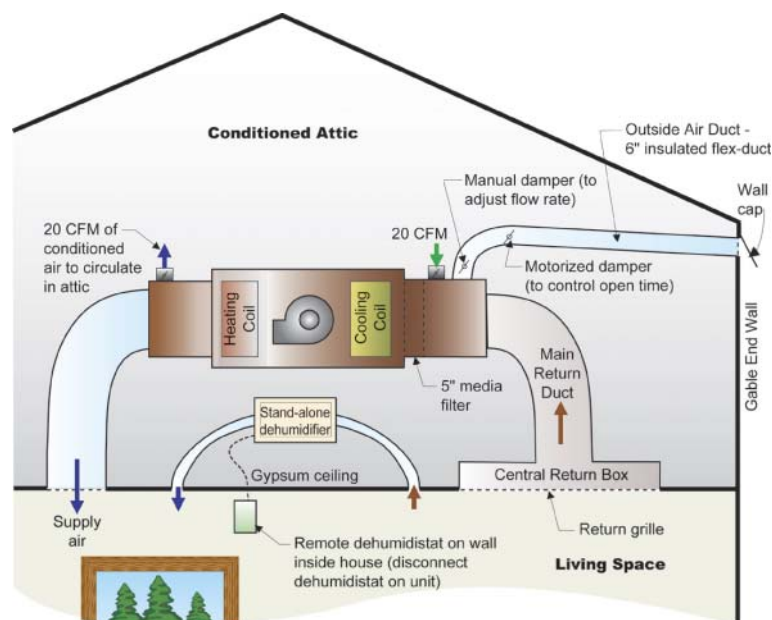
Figure 4. A conditioned attic
