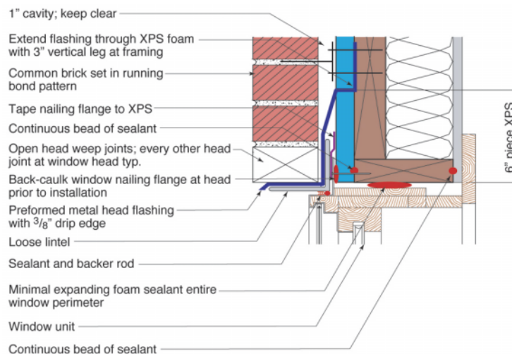
Figure 39. Rough opening flashing
