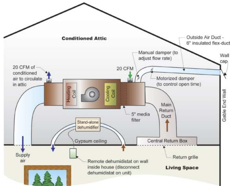
Figure 11. Dehumidification
