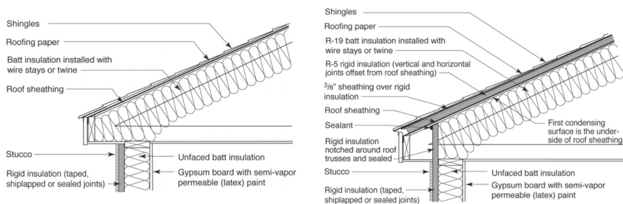
Figure 70. Unvented, conditioned attic design
