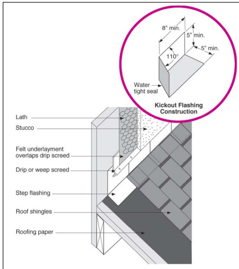
Figure 34. Stucco flashing
