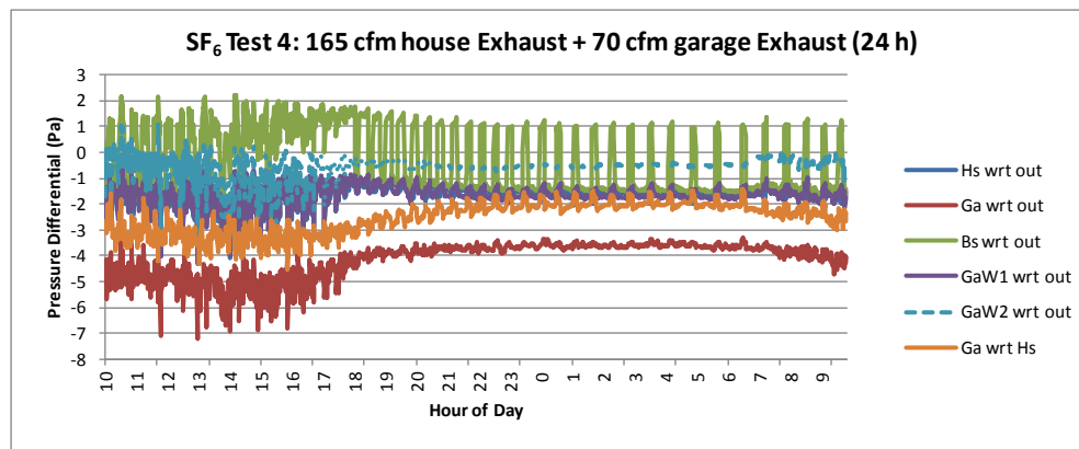
Figure 24. SF 6 test 4, 165 cfm House Exhaust and 70 cfm Garage Exhaust, monitored pressure differentials showing the garage pressure about 2 Pa negative wrt the house
