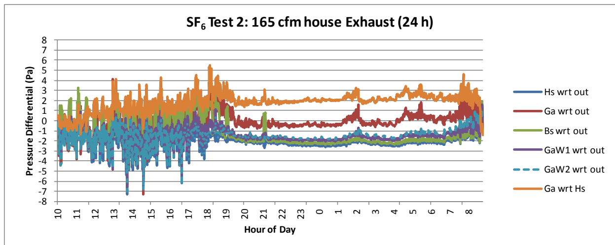
Figure 20. SF 6 test 2, 165 cfm House Exhaust, monitored pressure differentials showing the garage pressure about 2 Pa positive wrt the house
