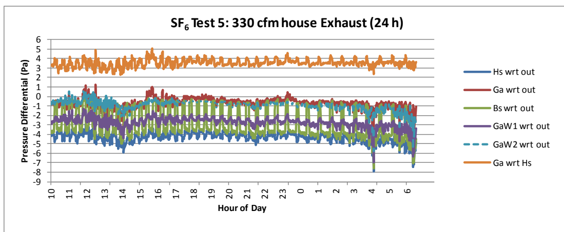
Figure 26. SF 6 test 5, 330 cfm House Exhaust, monitored pressure differentials showing the garage pressure about 3.5 Pa positive wrt the house
