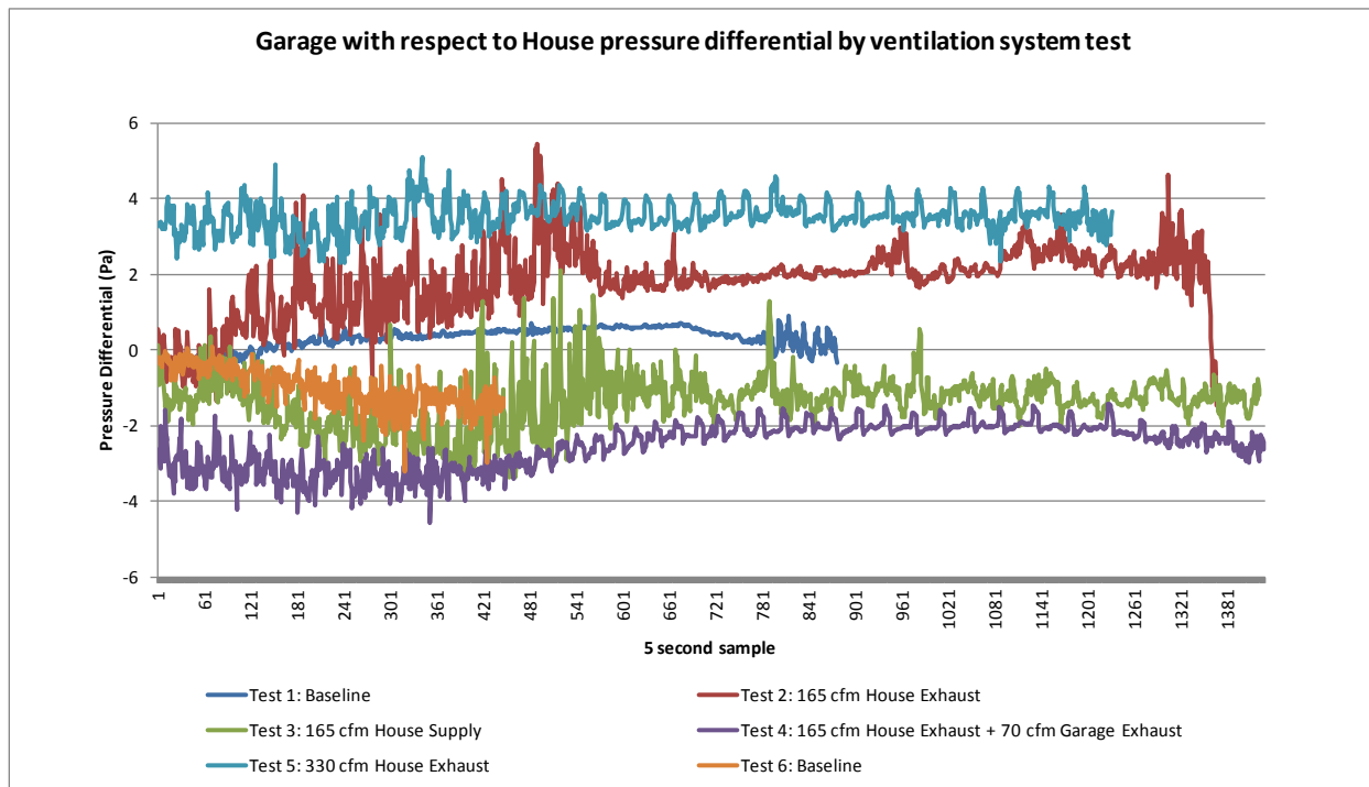
Figure 29. Pressure differential of the garage wrt house for each tracer gas test
