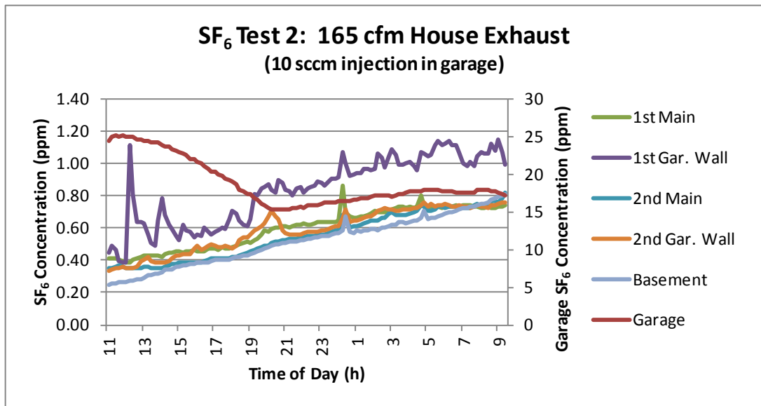
Figure 19. SF 6 test 2, 165 cfm House Exhaust ventilation tracer gas test showing that, by the end of the 24-hour test, 4.6% \pm 1.4% of the air in the house came from the garage (0.78/17 = 0.046)
