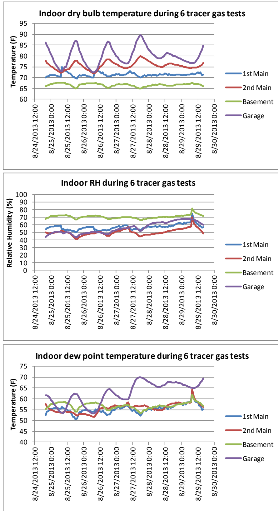
Figure 16. Indoor temperature and humidity conditions during the six tracer gas tests
