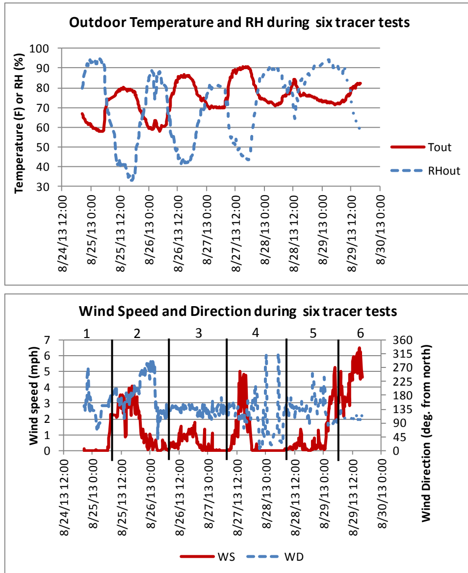
Figure 15. Weather conditions during the six tracer gas testing periods
