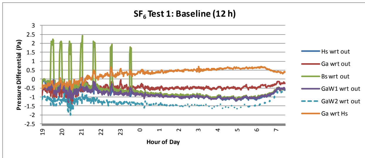
Figure 18. SF 6 Test 1, Baseline, monitored pressure differentials showing the garage pressure about 0.5 Pa positive with respect to the house
