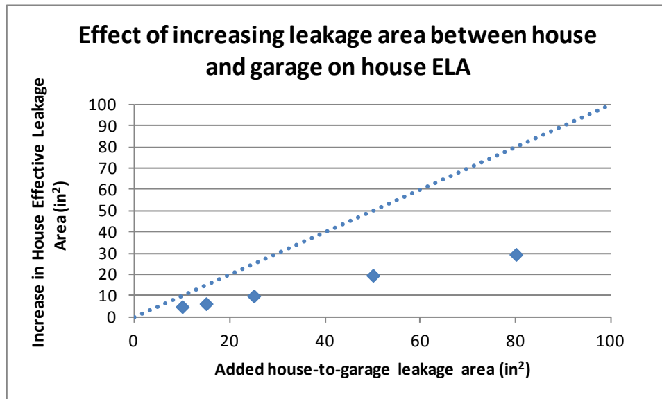
Figure 14. House leakage area increased by less than half the physical house-to-garage opening area added
