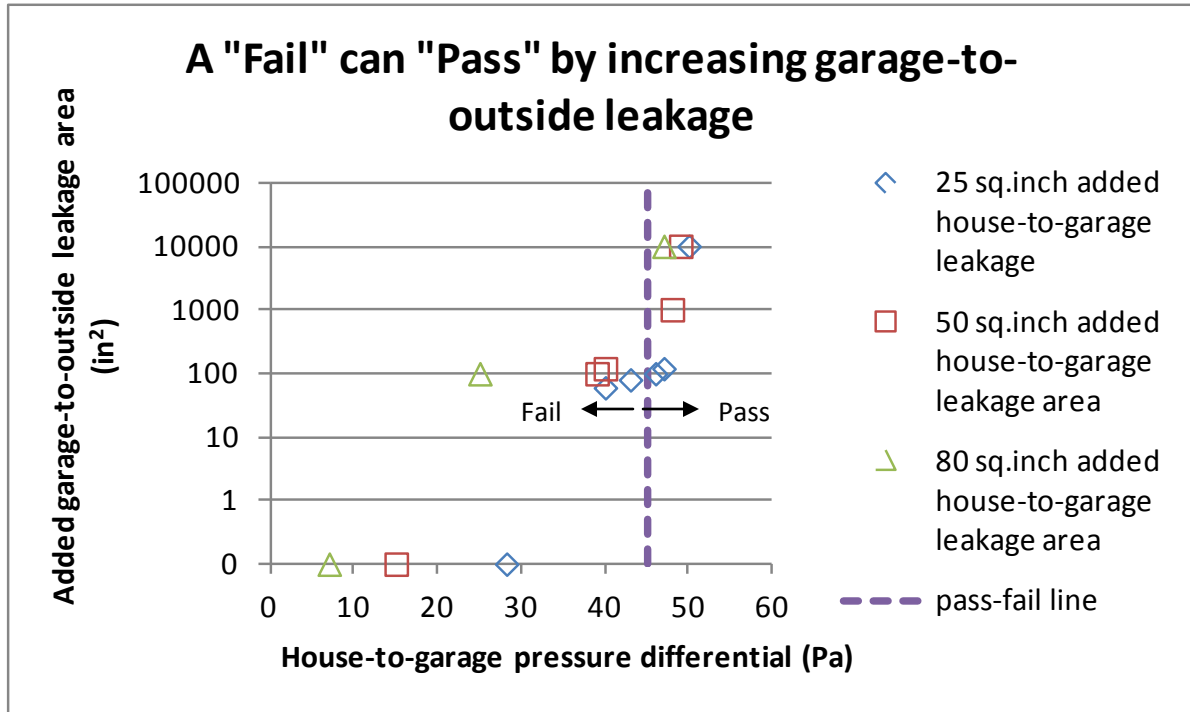
Figure 12. Test results showing inadequacy of house-to-garage pressure differential as a single criterion for house-to-garage airtightness
