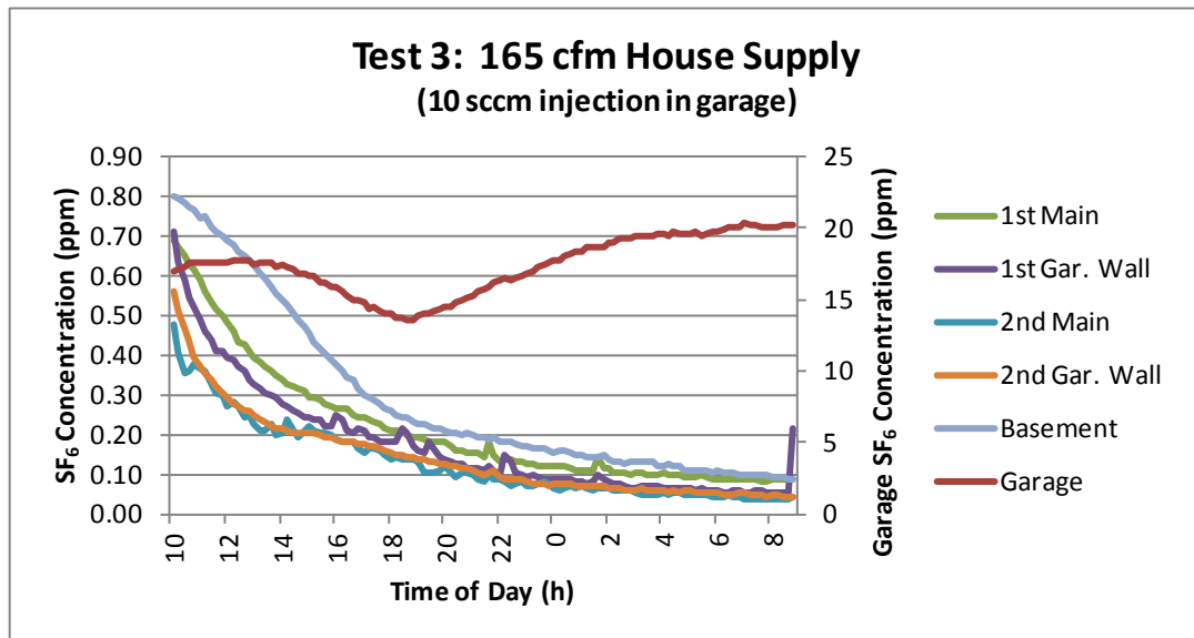
Figure 21. SF 6 Test 3, 165 cfm House Supply ventilation tracer gas test showing that, by the end of the 24-hour test, supply ventilation had suppressed essentially all air transfer from the garage to the house ( 0.1/20 = 0.005 )
