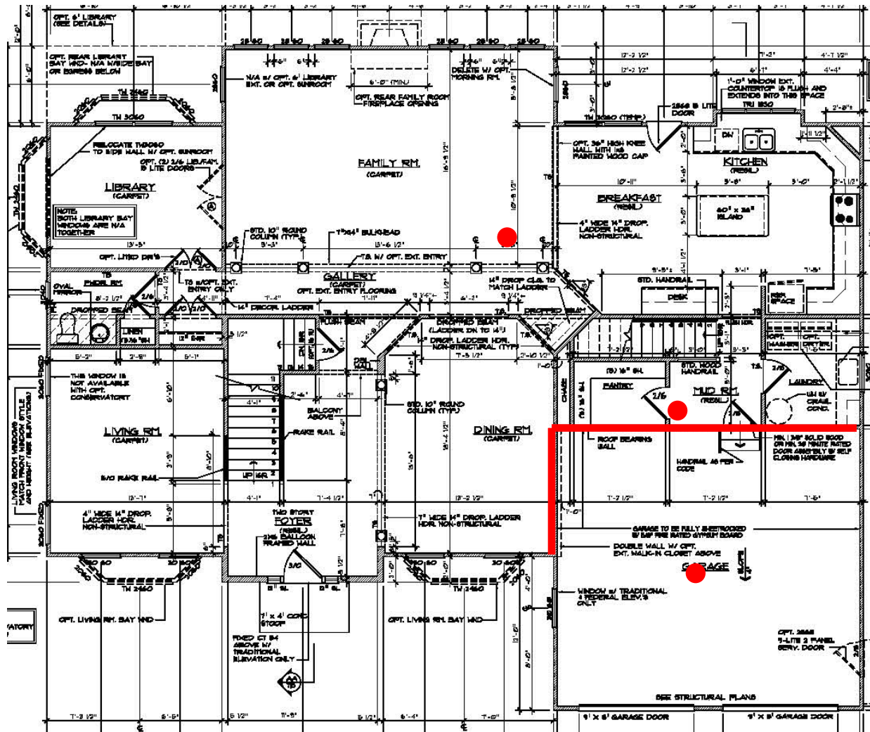
Figure 2. First-floor plan, with garage-to-house interface walls marked with thick red lines, and with red dots marking measurement station locations
