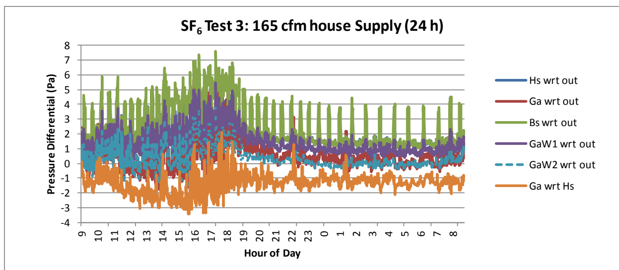
Figure 22. SF 6 test 3, 165 cfm House Supply, monitored pressure differentials showing the garage pressure about 1.5 Pa negative wrt the house
