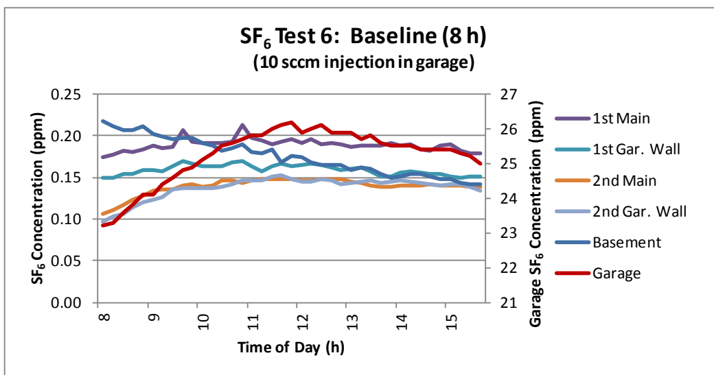
Figure 27. SF 6 Test 6, the final Baseline tracer gas test showed again that there was little garage-to-house air transfer across the well-sealed garage to house interface ( 0.16/25 = 0.006 )
