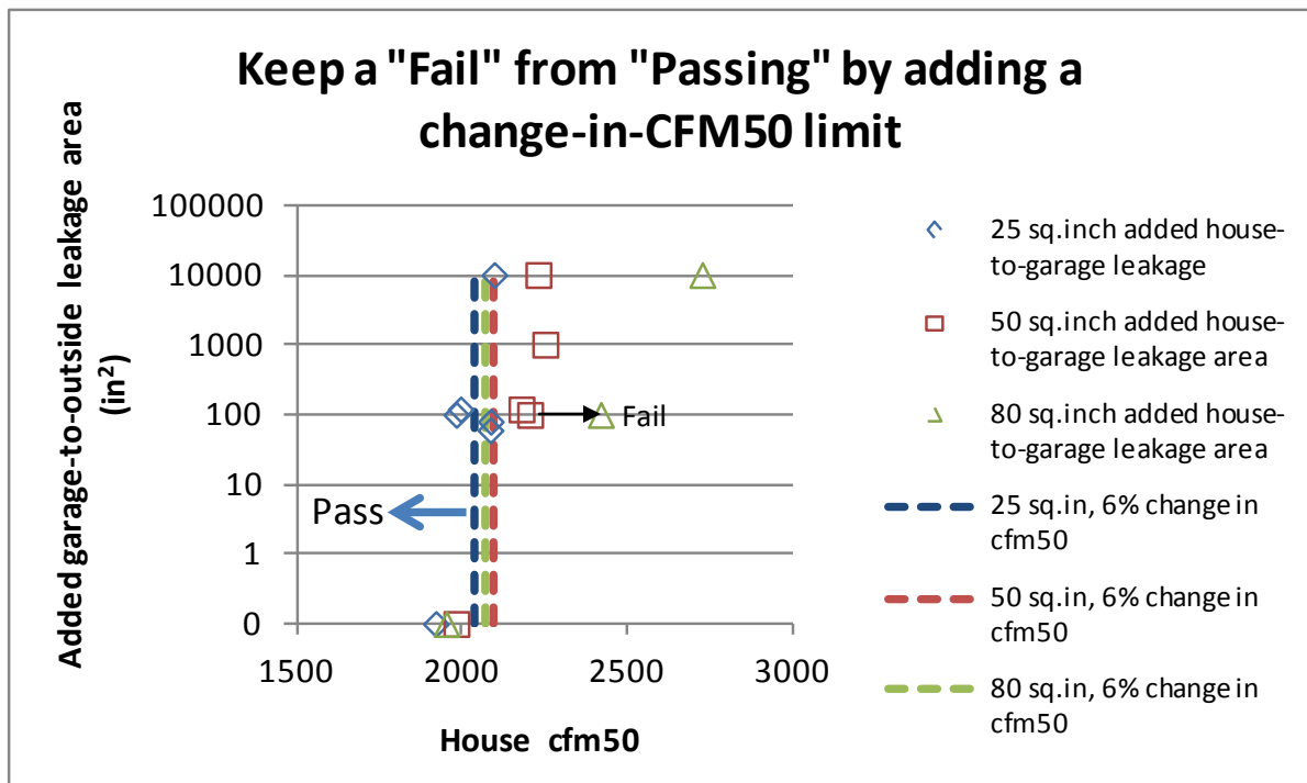
Figure 13. Elimination of false positives was found by adding a second criterion limiting the increase in house CFM50 to 6% with the overhead garage door open compared to closed
