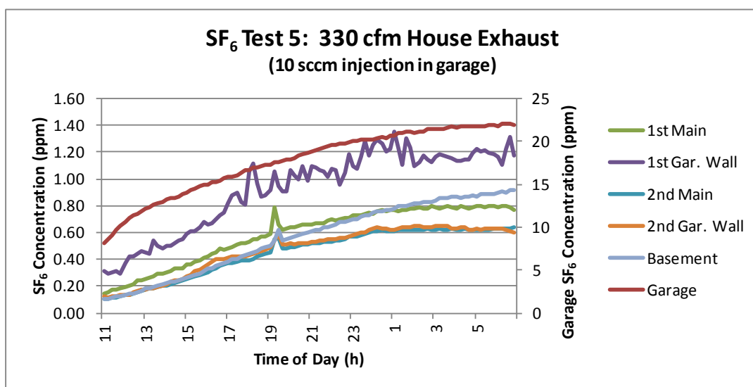
Figure 25. SF 6 test 5, 330 cfm House Exhaust tracer gas test showed that, by the end of the 24-hour test, 3.2\% \pm 1.4\% of the air in the house had come from the garage ( 0.7/22 = 0.032 )
