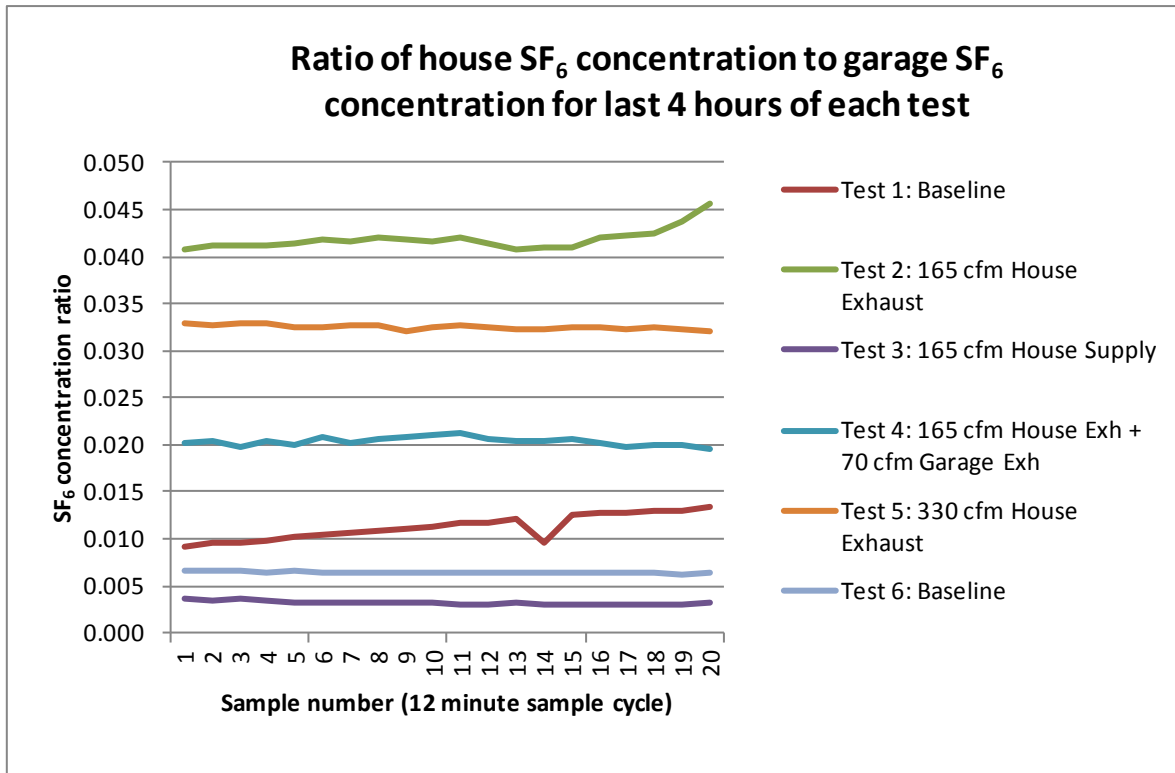
Figure 30. Ratio of average house SF 6 concentration to garage SF 6 concentration for the last 4 hours of each test, representing the fraction of house air that came from the garage
