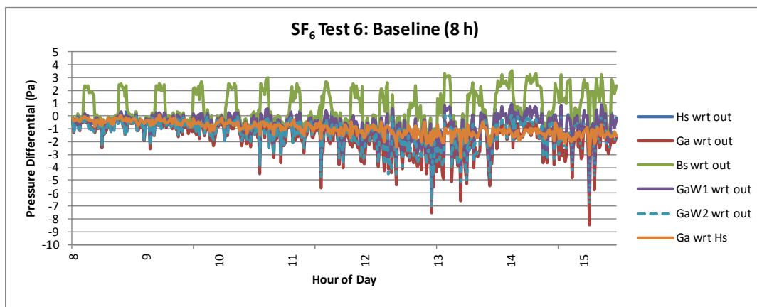
Figure 28. SF 6 Test 6, Baseline (8 h), monitored pressure differentials showing the garage pressure about 1.5 Pa negative wrt the house
