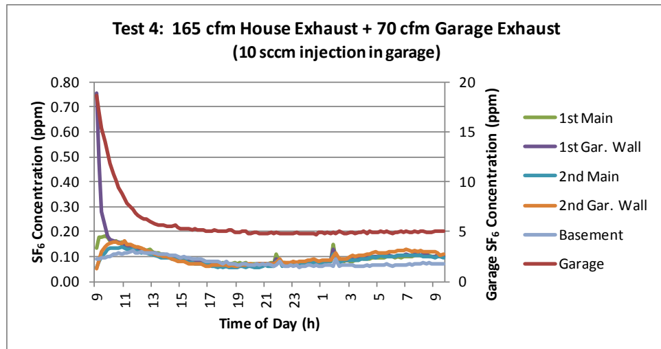
Figure 23. SF 6 test 4, 165 cfm House Exhaust and 70 cfm Garage Exhaust tracer gas test showed performance that was about the same as for the initial Baseline test ( 0.1/5.0 = 0.02 )
