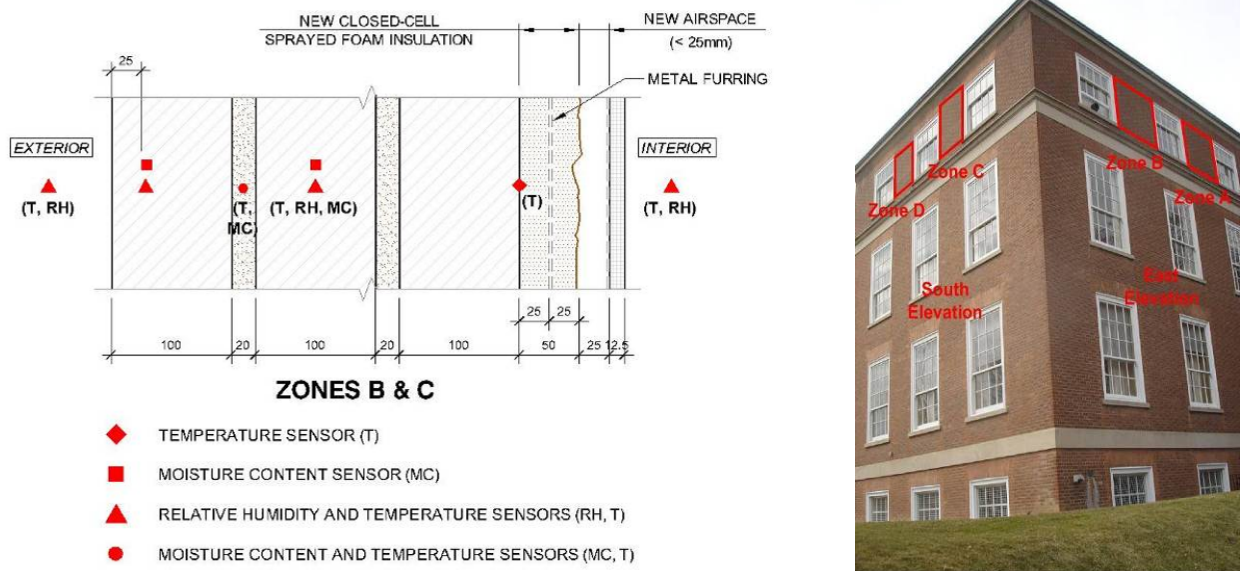
Figure 92. Instrumentation plan and monitoring locations, prototype installation in Toronto, Ontario
