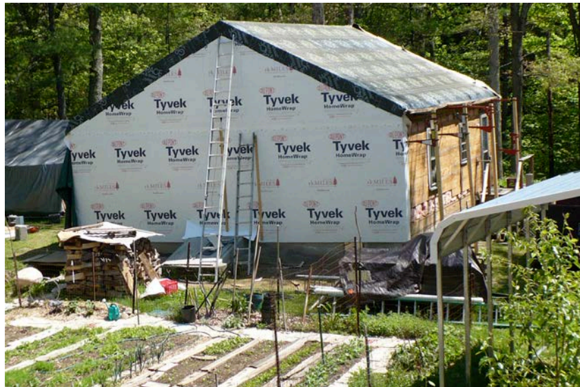
Figure 8. “Chainsaw” transition of air and water control membrane at rake
