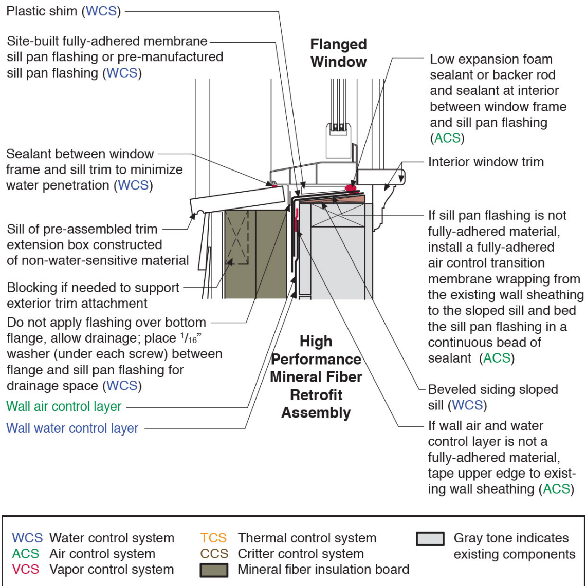
Figure 34. Schematic detail for window sill of new window or reinstalled window in a high performance mineral fiber retrofit wall assembly
