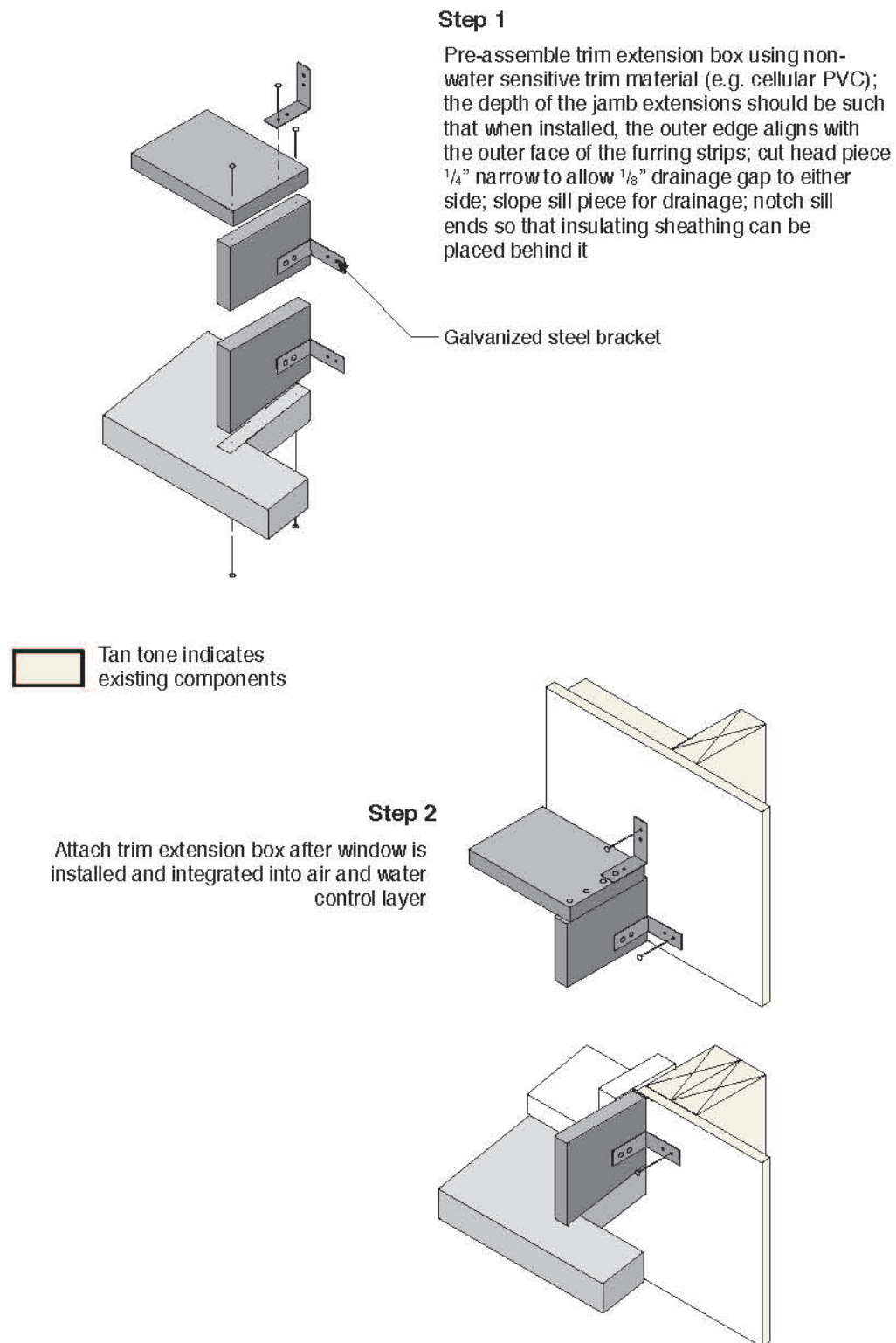
Figure 40. Steps 1 and 2 of exterior trim installation sequence for window in a high performance mineral fiber retrofit wall assembly
