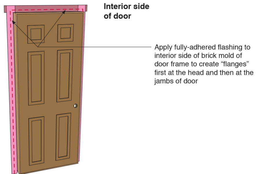
Figure 53. Steps 7 and 8 of installation sequence for new door or reinstalled door in a high performance mineral fiber retrofit wall assembly
