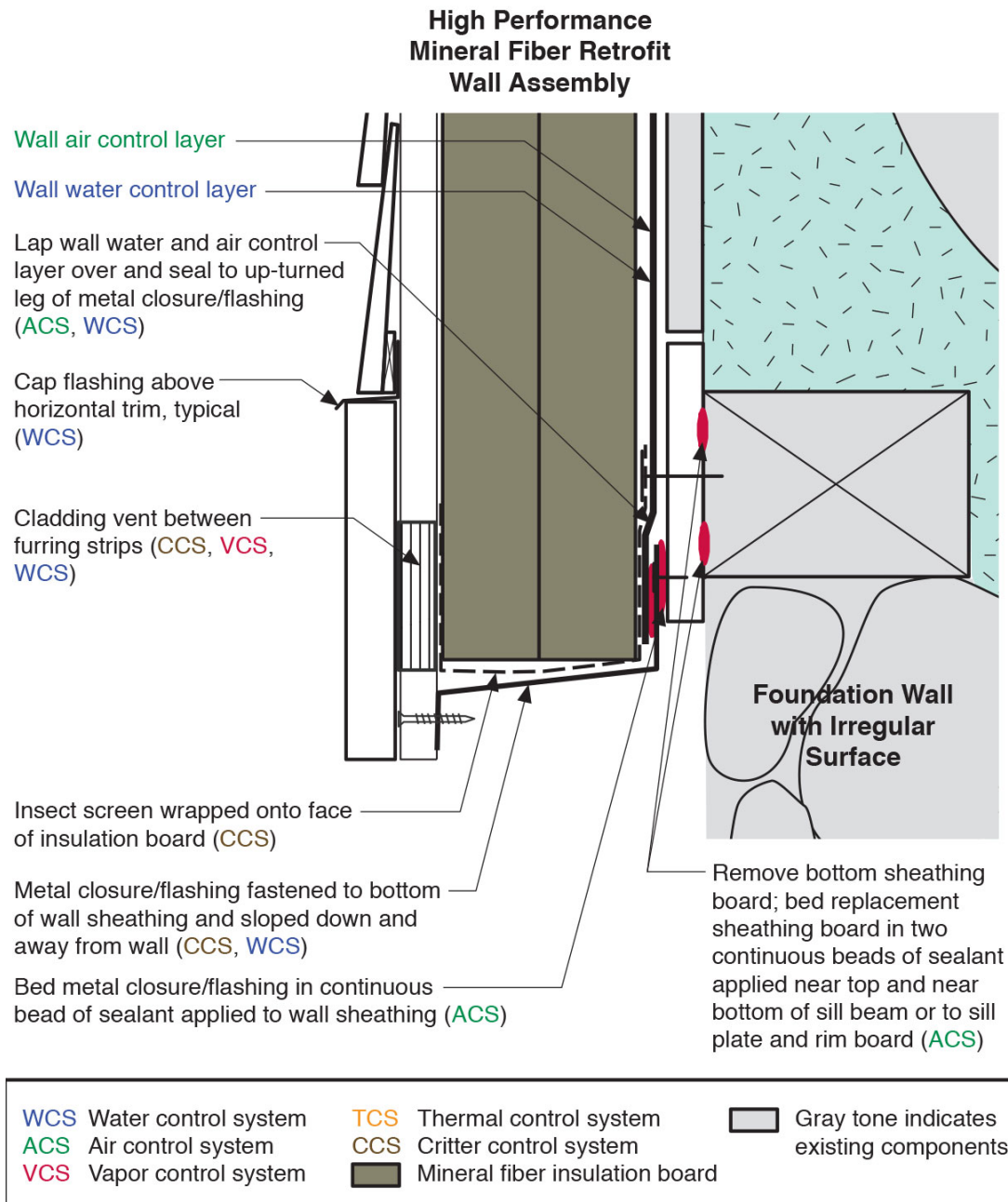
Figure 31. Schematic detail for transition from a high performance mineral fiber retrofit wall assembly to a bumpy-surface foundation wall
