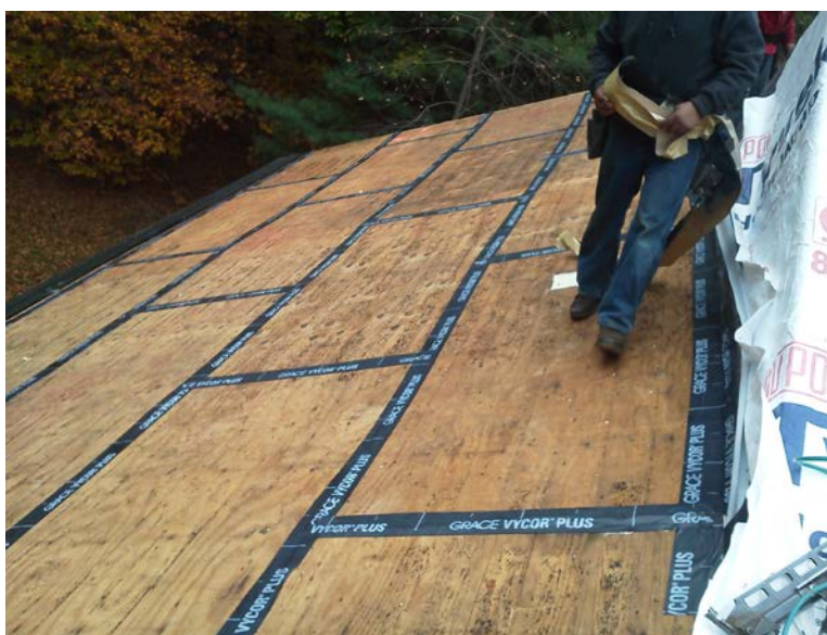
Figure 6. Taped wood panel roof sheathing as air control membrane
