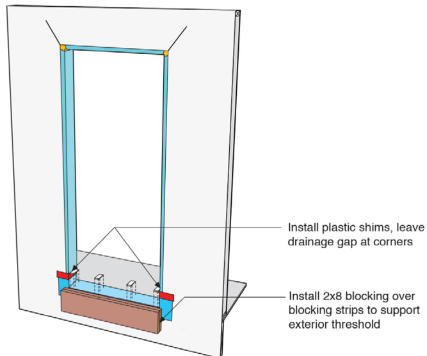
Figure 52. Steps 5 and 6 of installation sequence for new door or reinstalled door in a high performance mineral fiber retrofit wall assembly
