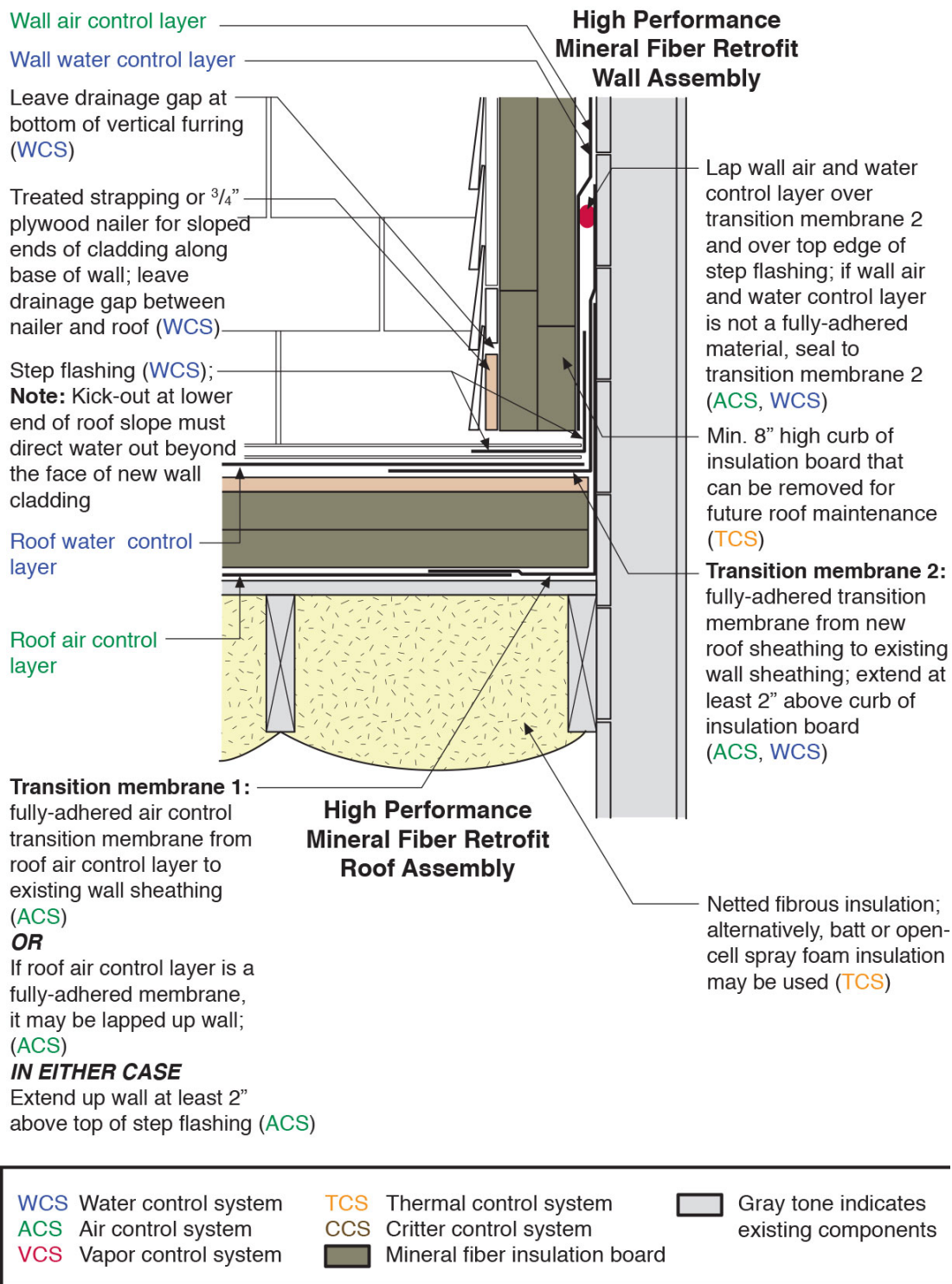
Figure 16. Schematic detail for transition from a lower high performance mineral fiber retrofit roof assembly to a high performance mineral fiber retrofit wall assembly
