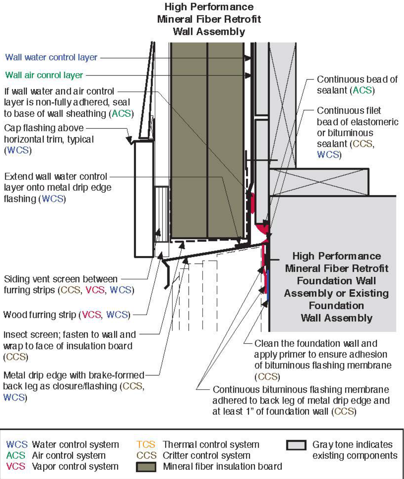
Figure 69. Schematic detail for transition from a high performance mineral fiber retrofit wall assembly to a top of high performance mineral fiber retrofit foundation wall assembly showing how the metal closure/transition flashing is secured and sealed to the foundation wall.
