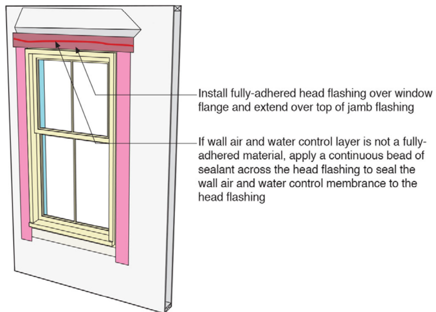
Figure 38. Steps 7 and 8 of installation sequence for new window or reinstalled window in a high performance mineral fiber retrofit wall assembly
