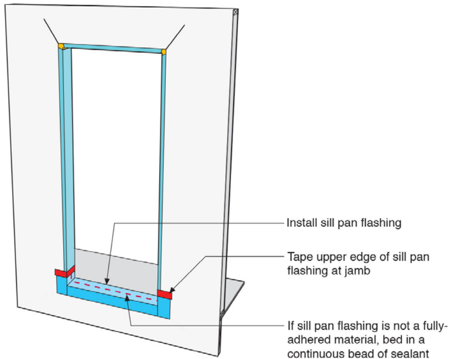
Figure 51. Steps 3 and 4 of installation sequence for new door or reinstalled door in a high performance mineral fiber retrofit wall assembly
