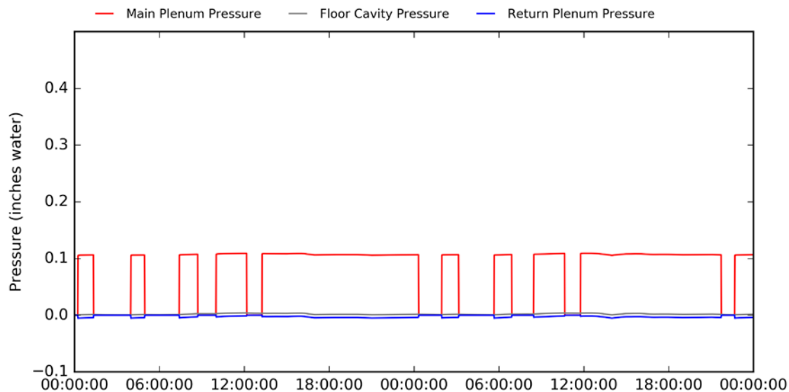
Figure 38. Static pressure in the trunk-and-branch system
