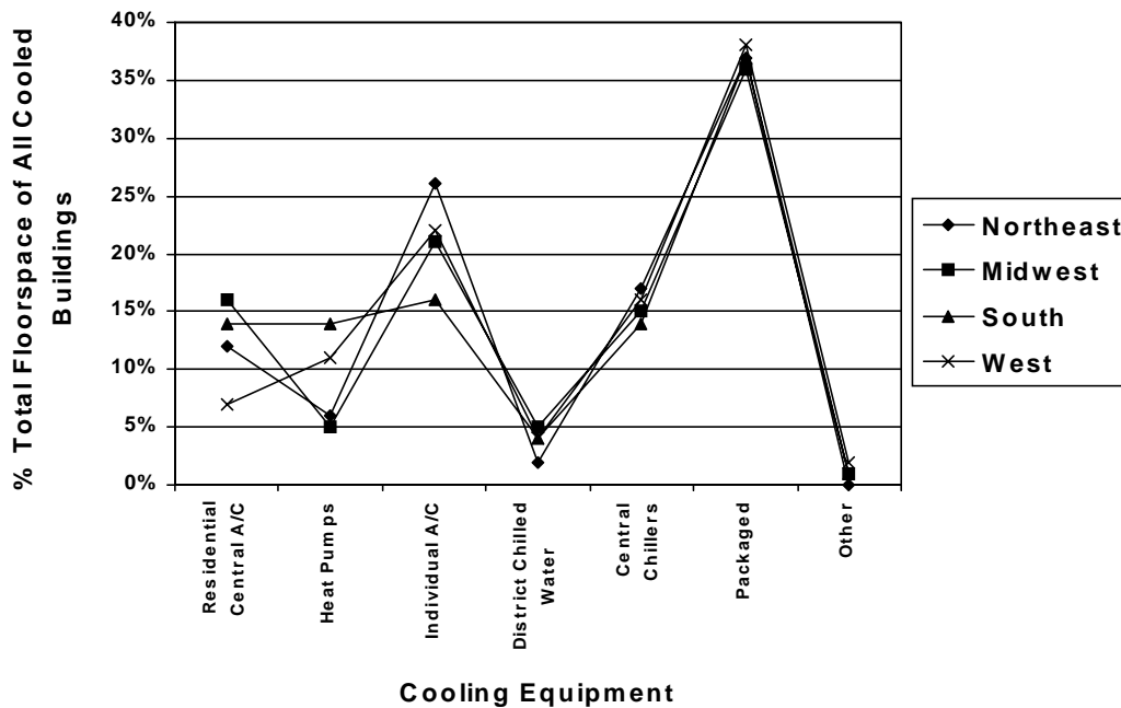
Figure 5-3: Equipment Type Distribution for Cooling
