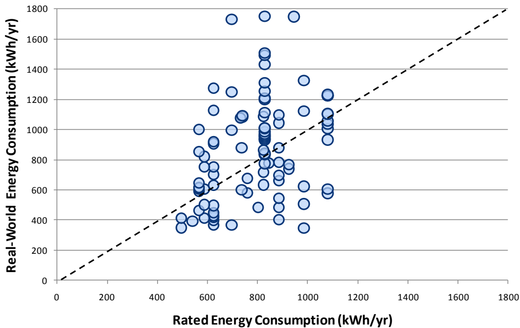
Figure 6. Comparison between real-world energy consumption and rated energy consumption (Source: PNNL 1998)
