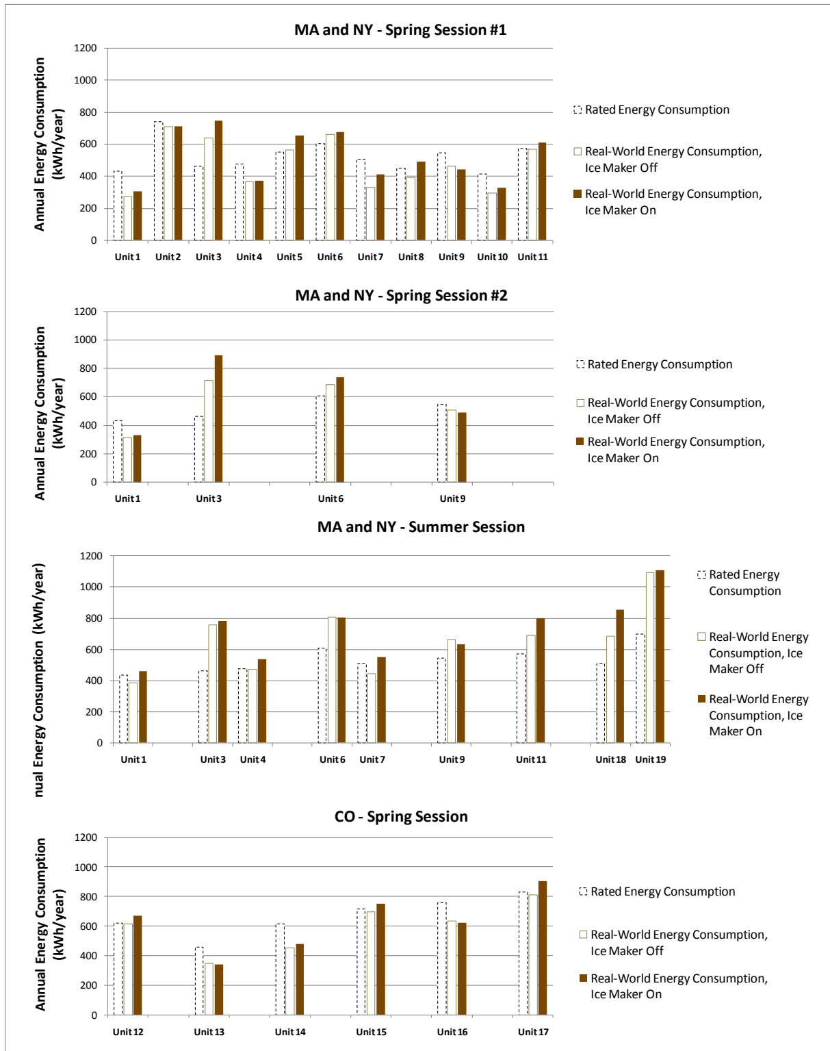
Figure 10. Comparison of rated energy consumption, energy consumption with ice maker off, and energy consumption with ice maker on
