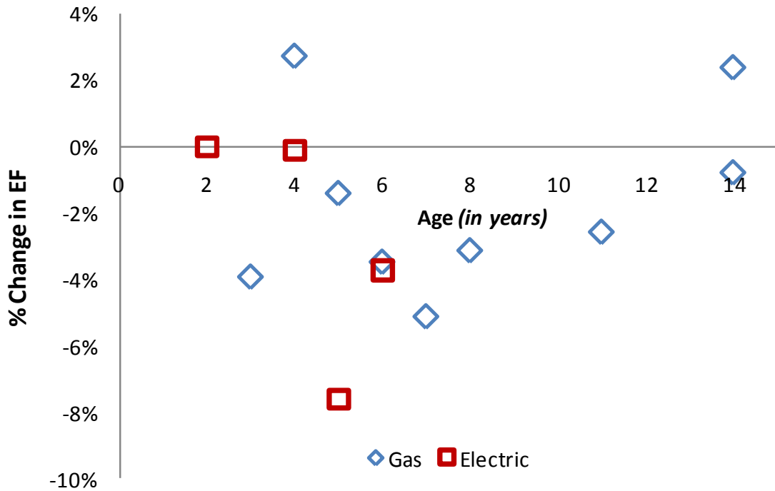
Figure 4: Plot of percent change in Energy Factor with age show no clear correlation between performance decline and age.
