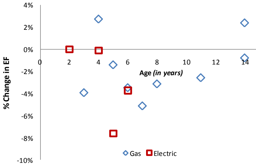
Figure 1: Plot of percent change in Energy Factor with age show no clear correlation between performance decline and age.
