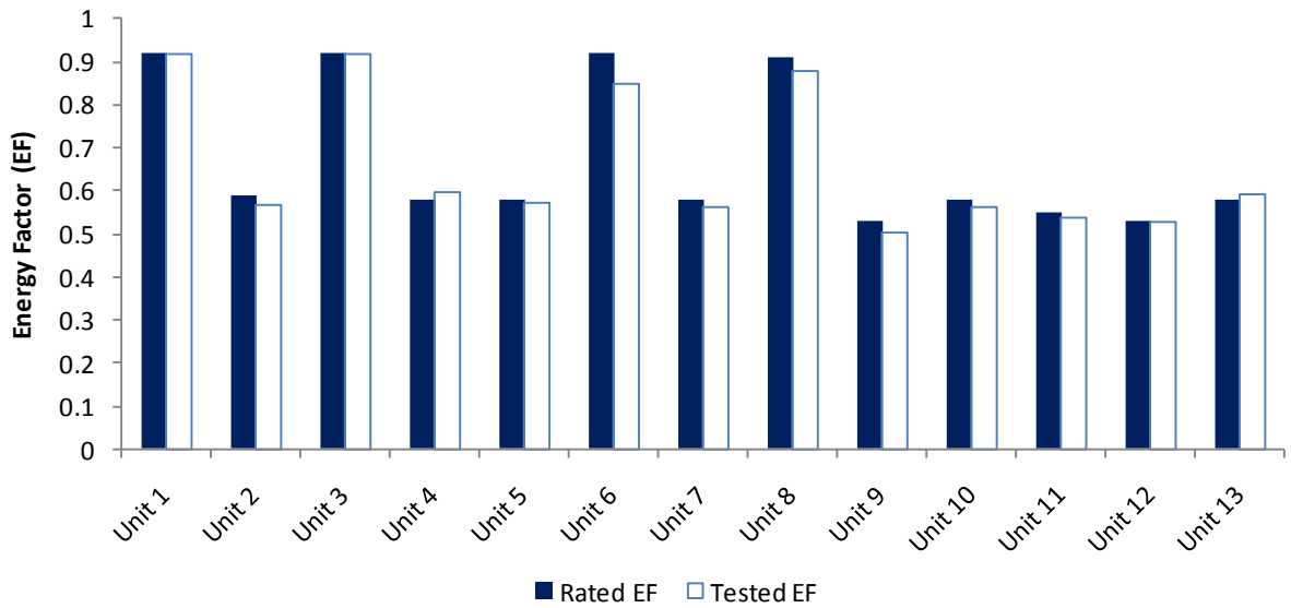
Figure 3: Comparison of Rated and Tested Performance of Water Heater Samples
