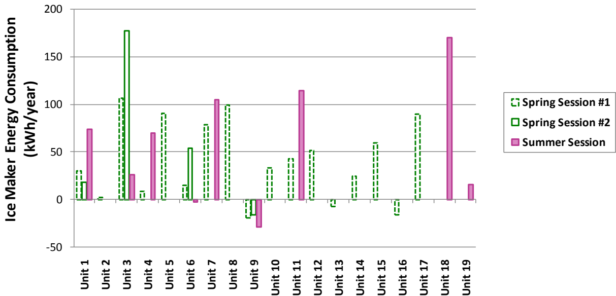
Figure 16. Ice maker energy consumption of each unit in the field study
