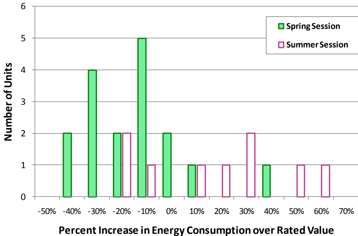
Figure 12. Distribution of percent increase in energy consumption over rated value
