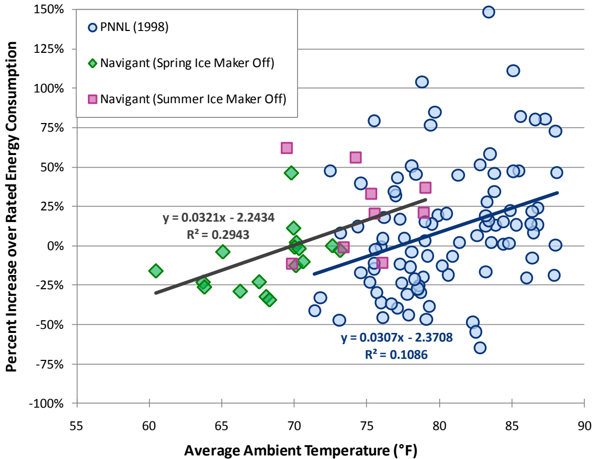
Figure 14. Comparison between rated energy consumption and actual energy consumption vs. average temperature – PNNL vs. Navigant (Source: PNNL 1998)
