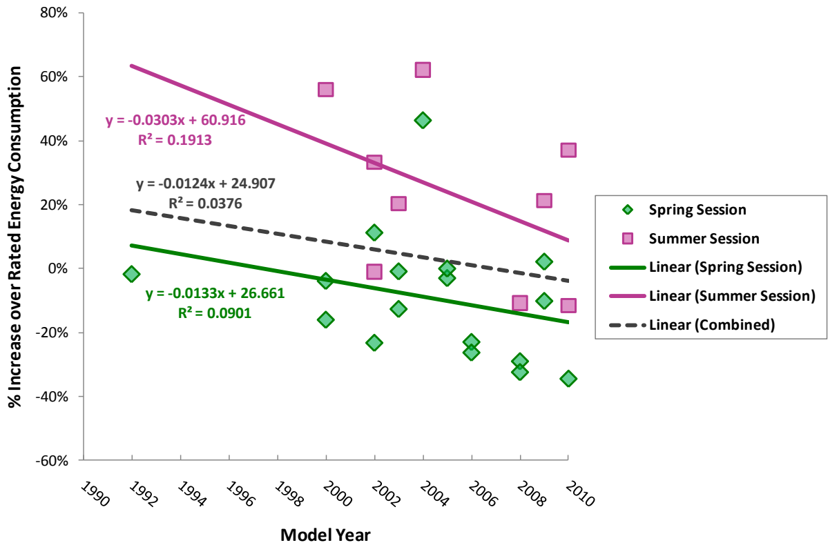
Figure 15. Percent increase over rated energy consumption as a function of model year
