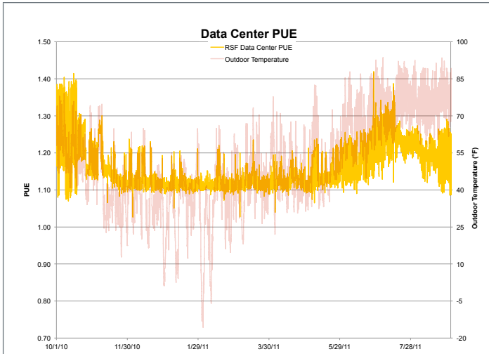
Figure 5.3. Hourly PUE performance over the first 11 months Illustration by Chad Lobato, NREL
