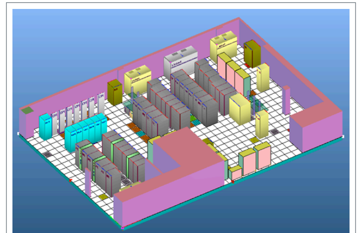
Figure 4 5. Model of the hot aisle/cold aisle layout in the NREL legacy data center
