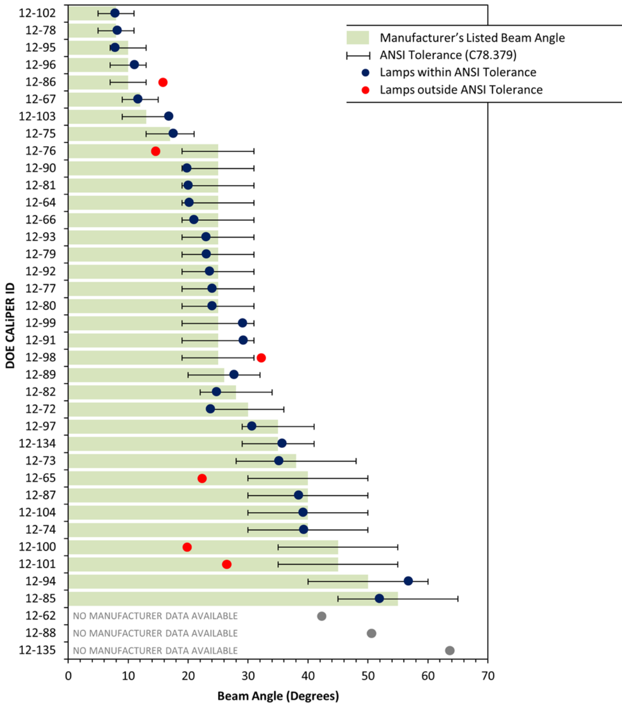
Figure 9. Accuracy of manufacturers' claimed beam angle. Six products fell outside ANSI tolerances.
