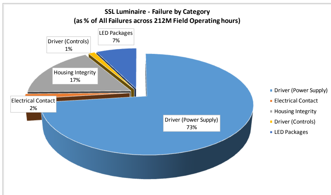
Figure 5. SSL luminaire failure modes, across 212 million field hours. Source: Appalachian Lighting Systems, Inc.
