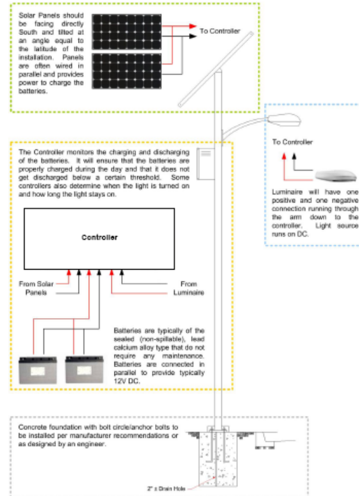
Figure 1 Typical Solar Lighting System Components
