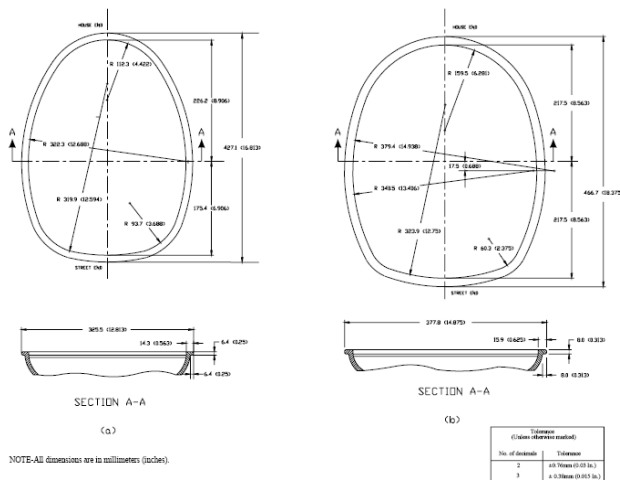
Figure 2A – Flange dimensions for refractors for medium horizontal-burning HID luminaires
