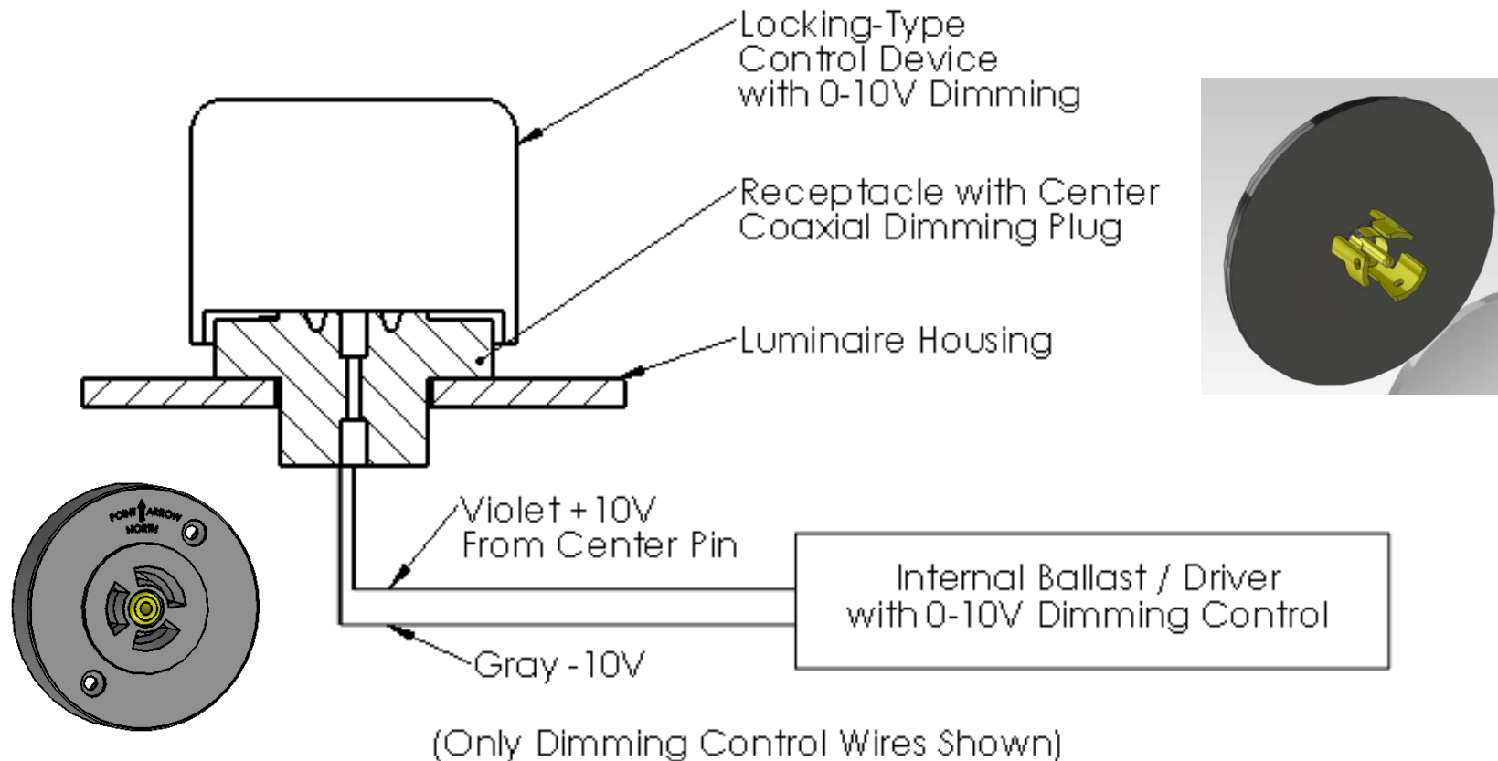
Locking-Type Controller with Modified 5 Conductor Receptacle
