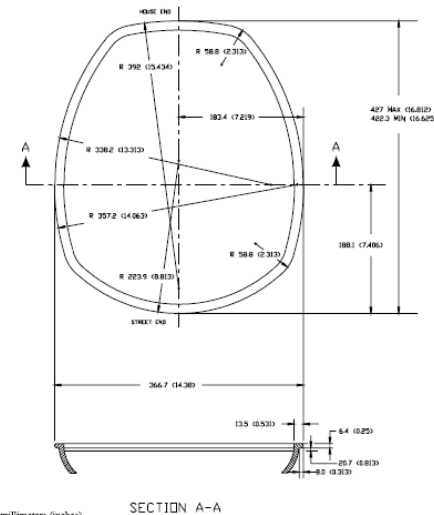
Figure 2B – Flange dimensions for refractors for medium horizontal-burning HID luminaires (continued)
