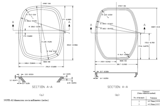
Figure 1 – Flange dimensions for refractors for small horizontal-burning HID luminaires
