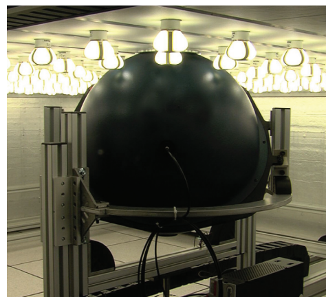
Long-term lumen maintenance is one of the pivotal tests for L Prize competition entrants. Photo courtesy of DOE.
