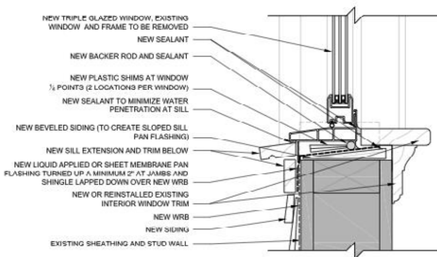
This diagram shows the sill detail for a replacement window in conjunction with siding replacement.
