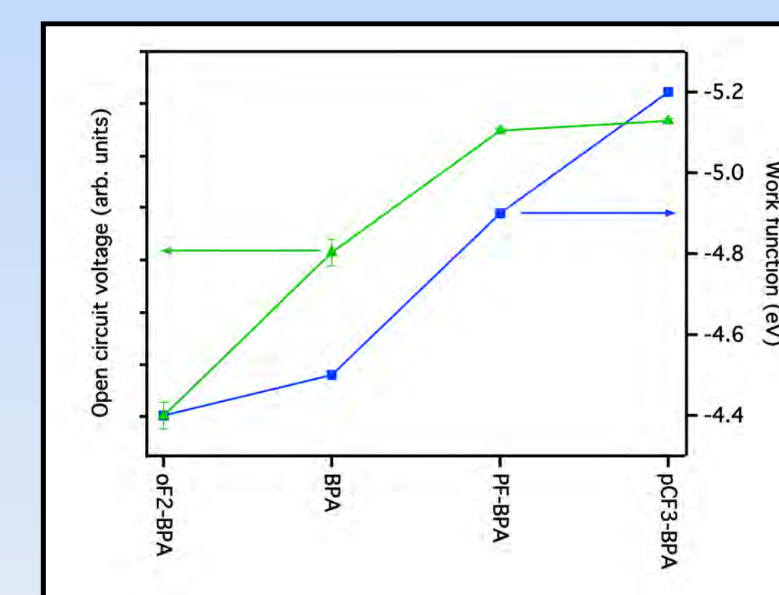
Figure 3: Demonstration of phosphonic acid SAMs tuning the open circuit voltage in BHJ solar cells roughly linearly with increasing work function of the modified substrate, glass/ITO/SAM.
