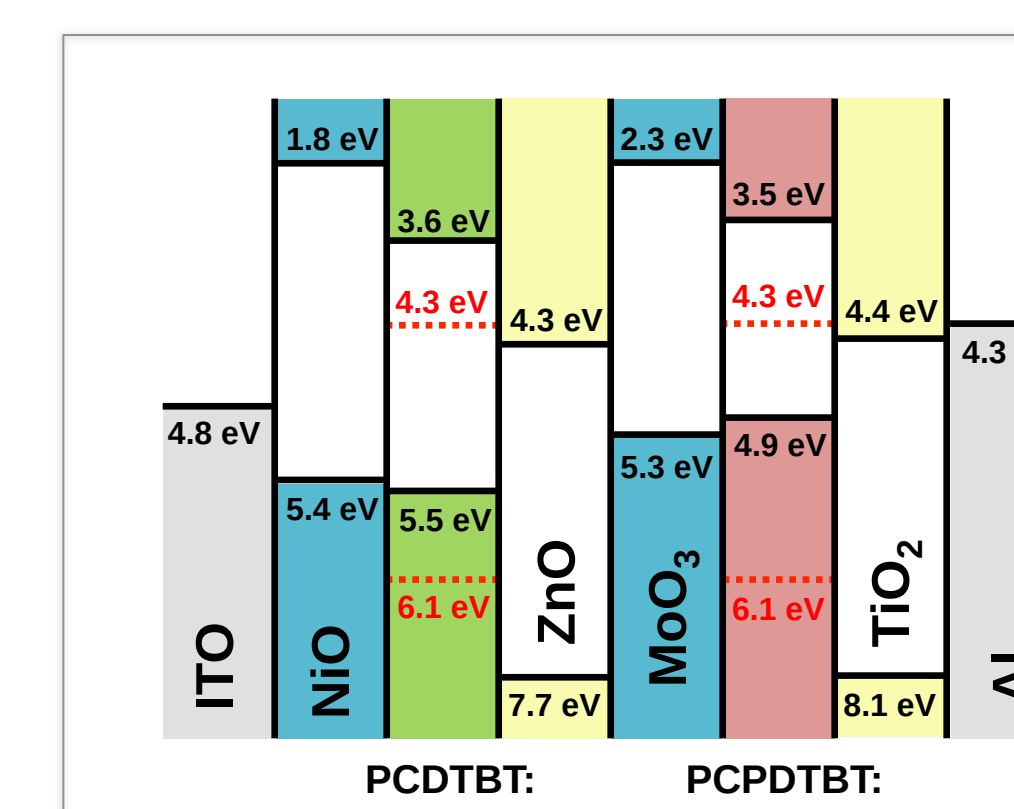
Figure 2: Energy levels for a PCPDTBT/PCDTBT multijunction solar cell using metal oxide electrode materials. Thin metals and self-assembled monolayers including thiols and phosphonic acids, may assist energy level alignment for efficient charge recombination.
