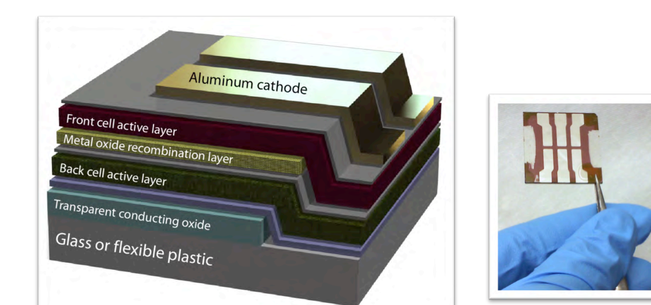
Figure 1: Standard multijunction device architecture using organic semiconducting and metal oxide materials.
