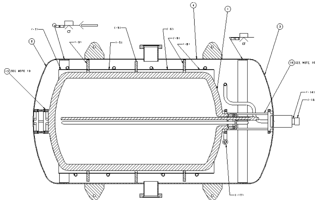
Figure 5. Insulation design for first-generation pressure vessel. The figure shows a vacuum space, for obtaining high thermal performance from the multilayer insulation, and instrumentation for pressure, temperature and level. Dimensions are given in cm.
