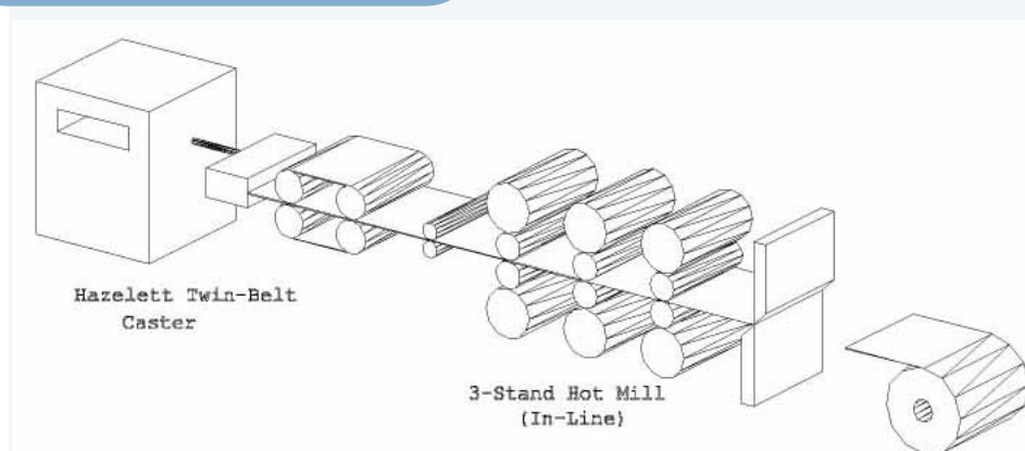
In-Line annealed continuous cast aluminum sheet.
