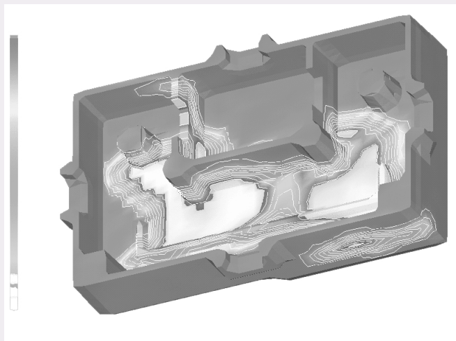
EPS volume fraction during filling of GM test box. Red is close pack and blue is empty.
