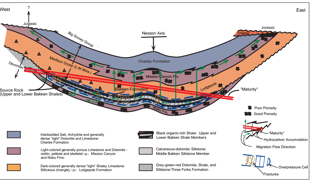
Figure BK-11.2. Schematic east-west section across the Williston Basin showing source-rock maturity, fluid overpressure, fracture, migration and hydrocarbon accumulation patterns in the Bakken formation and adjacent units (from Messiner, 1984).
