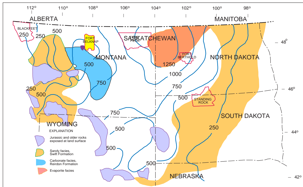
Figure BK-10.1. Thickness of Jurassic rocks in feet, showing approximate distribution of carbonate facies and evaporite facies (modified after Peterson, 1972).
