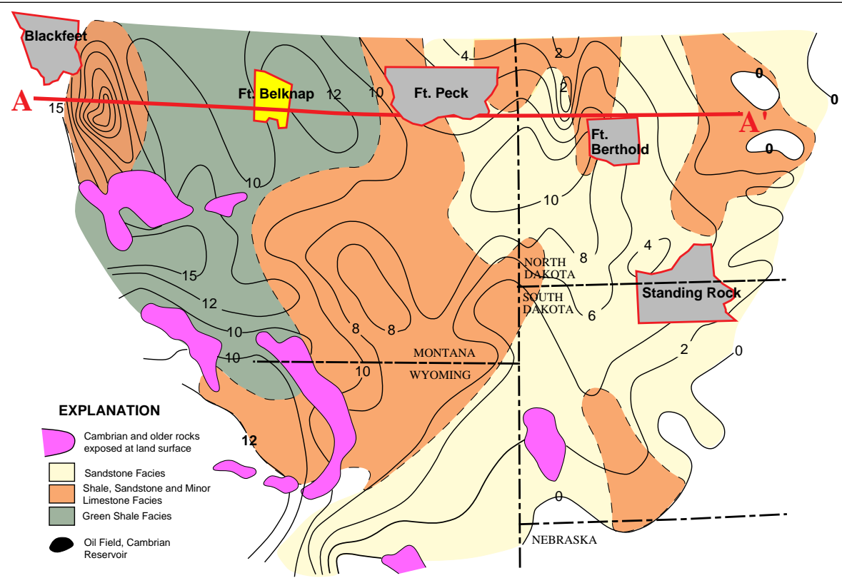
Figure BK-3.1. Thickness in hundreds of feet and rock facies map of Deadwood Formation or equivalent rocks. (Cambrian and Lower Ordovician)
