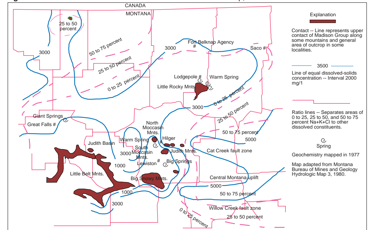
Figure BK-10.4. Dissolved solids concentration and ratio of sodium, potassium, and chloride to dissolved solids concentration in water of the Madison Group, Montana.
