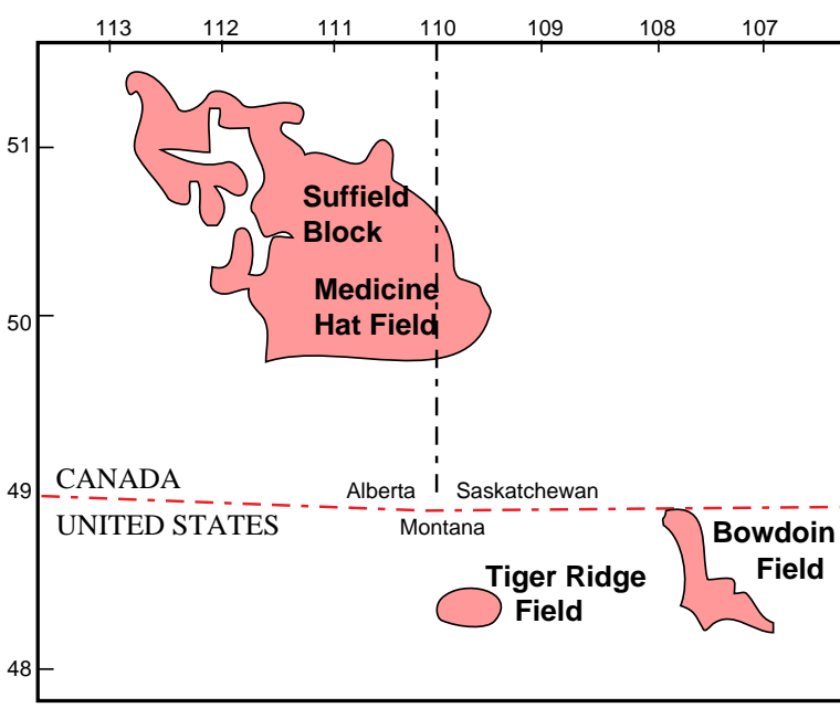
Figure BK-9.3. Distribution of shallow gas fields in north-central Montana, southeastern Alberta, and southwestern Saskatchewan. Bowdoin field and large area in Canada produce from low-permeability reservoirs. Tiger Ridge field produces from structural traps of conventional reservoirs.
