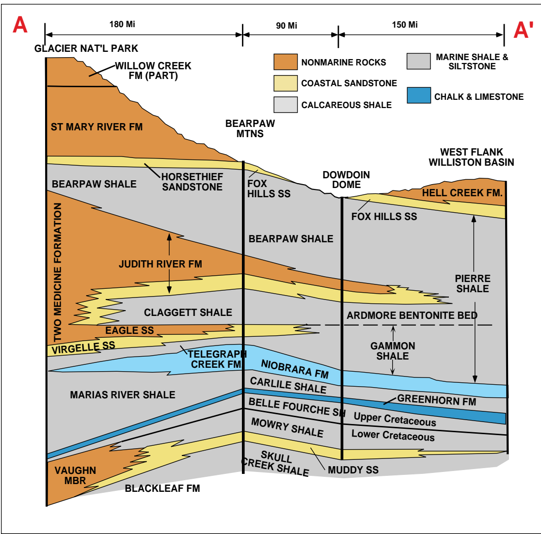
Figure BK 9.2. Diagrammatic sequence of selected Cretaceous Rocks from Glacier National Park to the west flank of the Williston Basin, Montana (after Rice and Shurr, 1980).
