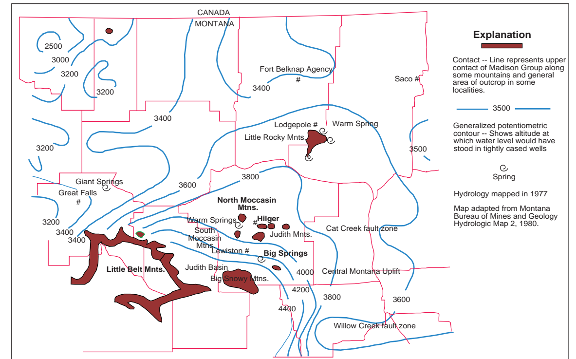
Figure BK-10.3. Potentiometric surface of water in the Madison Group, central Montana.
