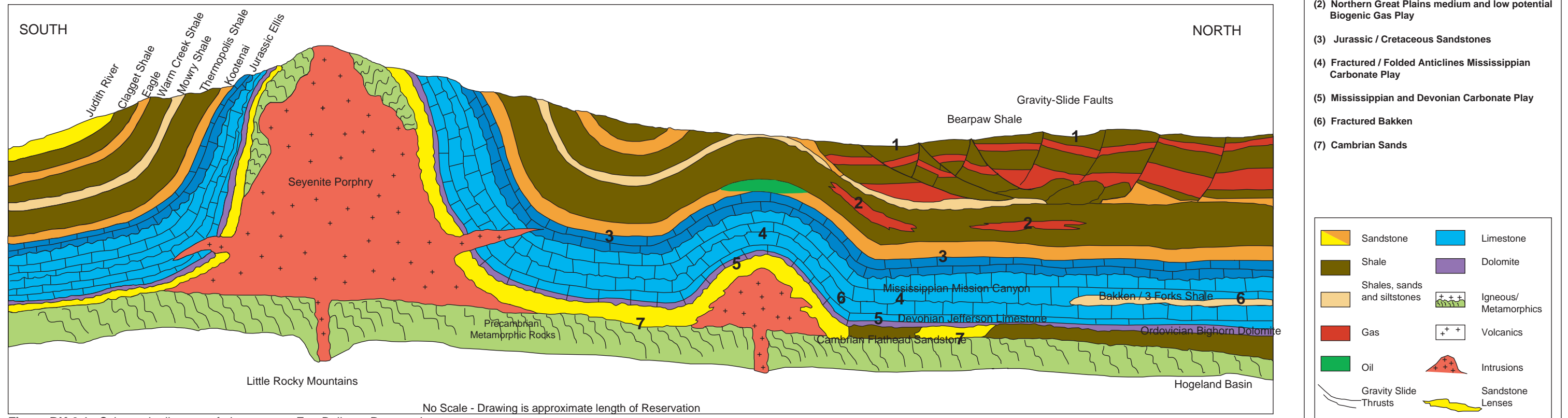
Figure BK-6.1. Schematic diagram of play types at Fort Belknap Reservation.
