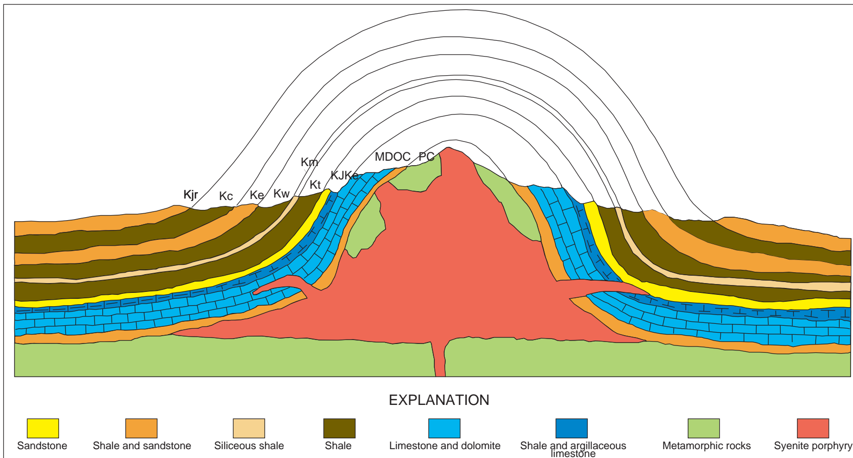
Figure BK-5.1. Schematic section through the Little Rocky Mountains, showing the laccolithic intrusion of syenite porphyry and the doming of the sedimentary rocks. Tsp, syenite porphyry; Kjr, Judith River Formation; Kc, Clagget Shale; Ke, Eagle Sandstone; Kw, Warm Creek Shale; Km, Mowry Shale; Kt, Thermopolis Shale; KJKe, Kootenai Formation and Ellis Group; MDOC, limestone and sandstone of Mississippian to Cambrian age; and PC, Precambrian rocks.
