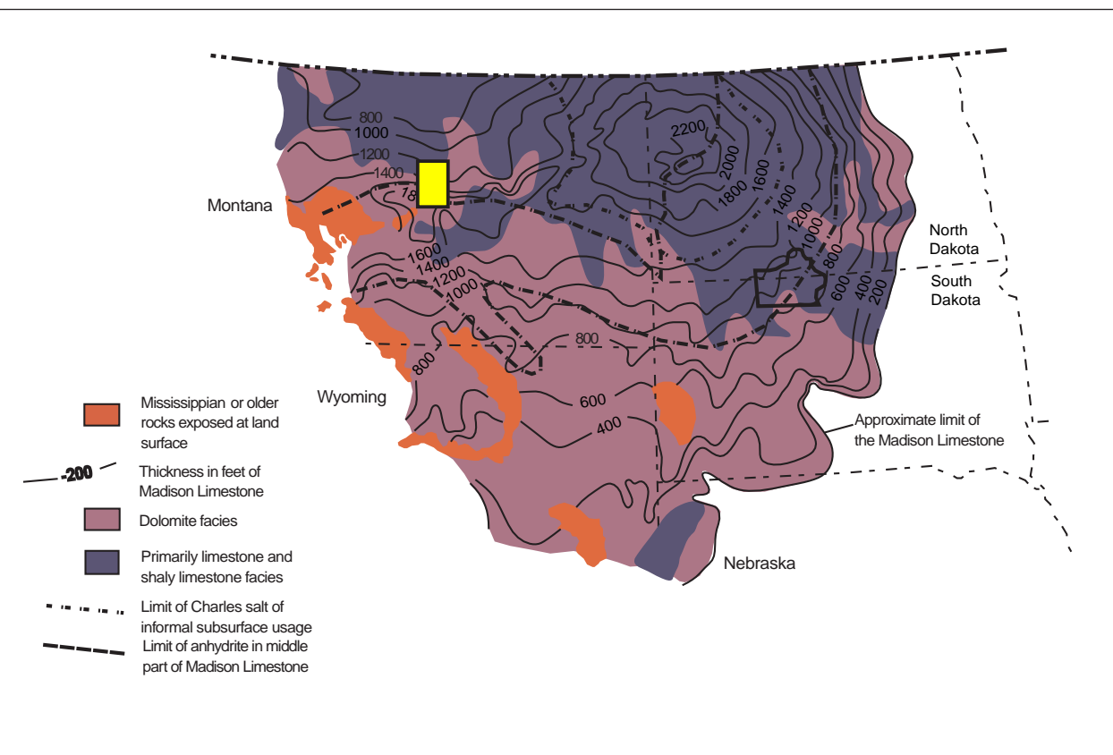
Figure BK-10.2. Thickness in feet and generalized rock facies of the Madison Group (Mississippian) and equivalent rocks (modified after Peterson, 1981, 1984b).
