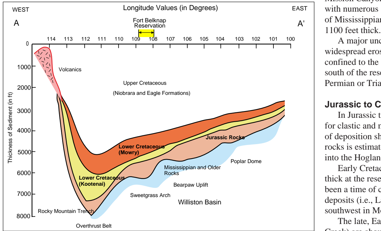
Figure BK-4.4. Generalized time-interval cross-section of Cretaceous and older rocks along A-A' line of section.
