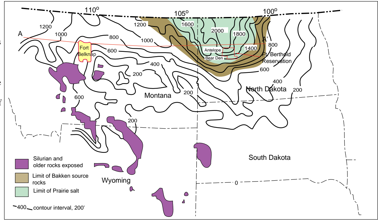
Figure BK-11.3. Map showing thickness of Devonian rocks, limit of Prairie salt, limit of Bakken source rock, location of analog fields and reservation, and location of regional cross-section A-A' (modified after Peterson, 1987).
