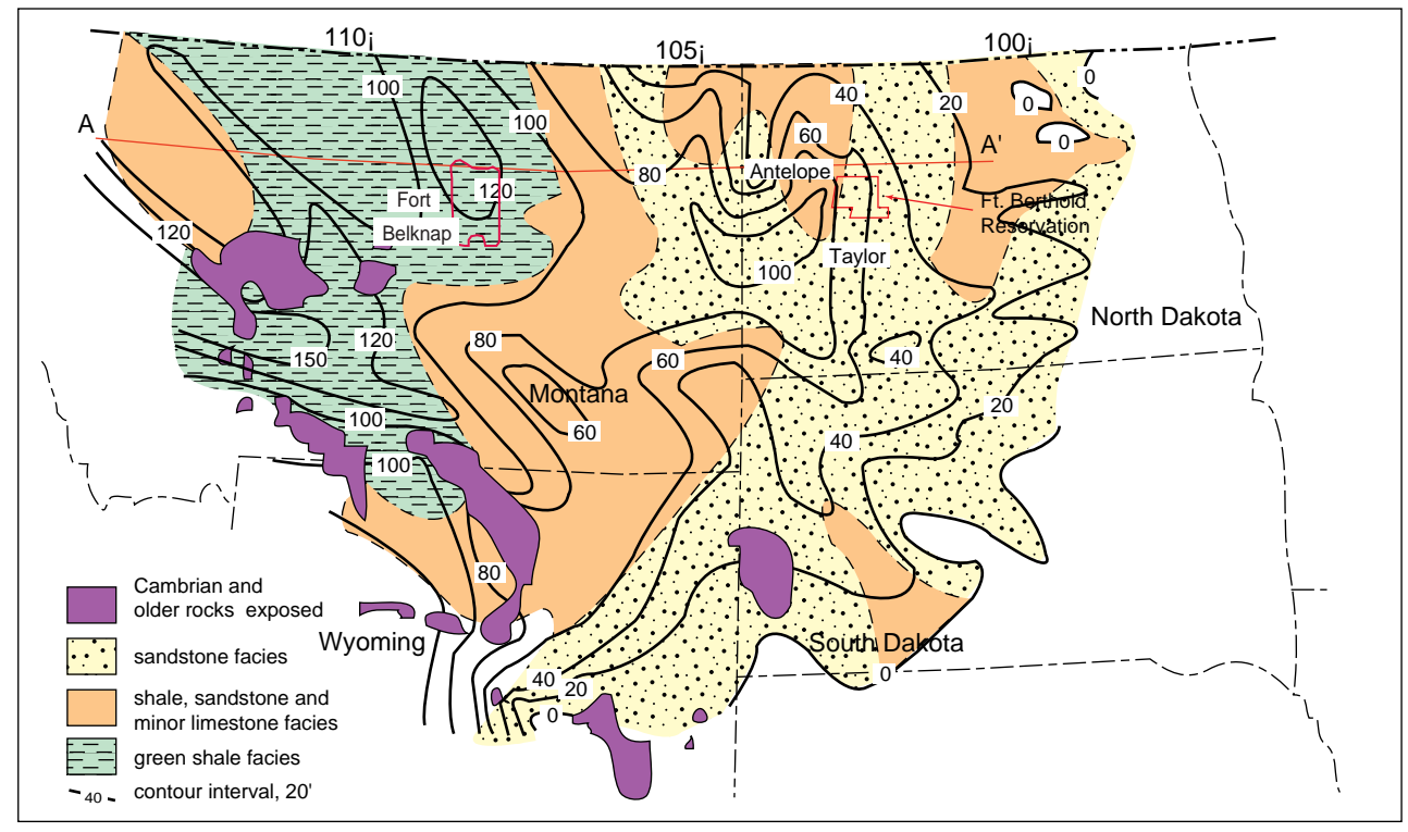
Figure BK-11.4. Thickness of Deadwood and equivalent rocks, location of analog fields, location of reservation, and location of regional cross-section A-A' (modified after Peterson, 1987).
