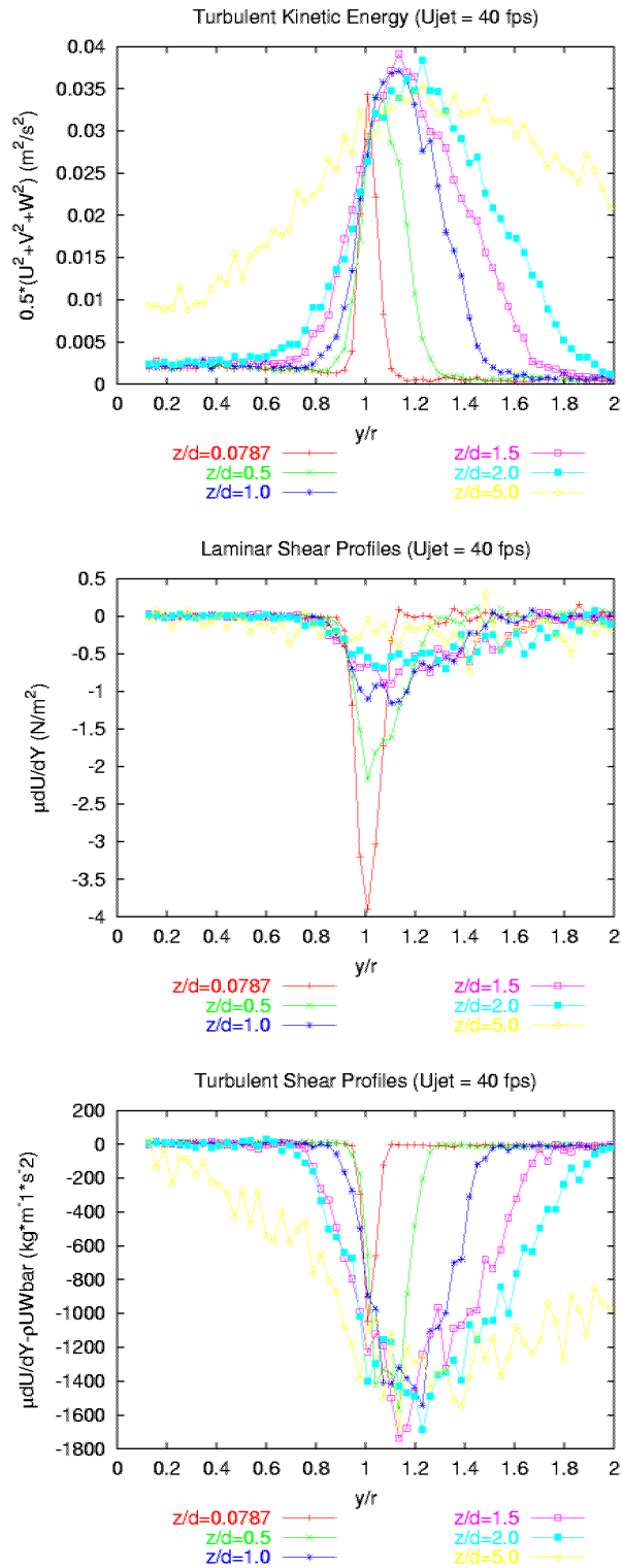
Figure 4.6. Profiles of TKE, LAMSHEAR, and TURBSHEAR at jet speed U = 40 fps.
