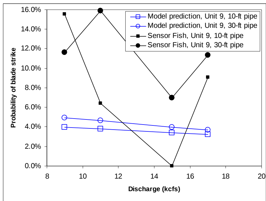
Figure 3.6. Prediction of Blade Strike by the Deterministic Model as a Function of Discharge and Comparison with Sensor Fish Results, Existing Unit (Unit 9)
