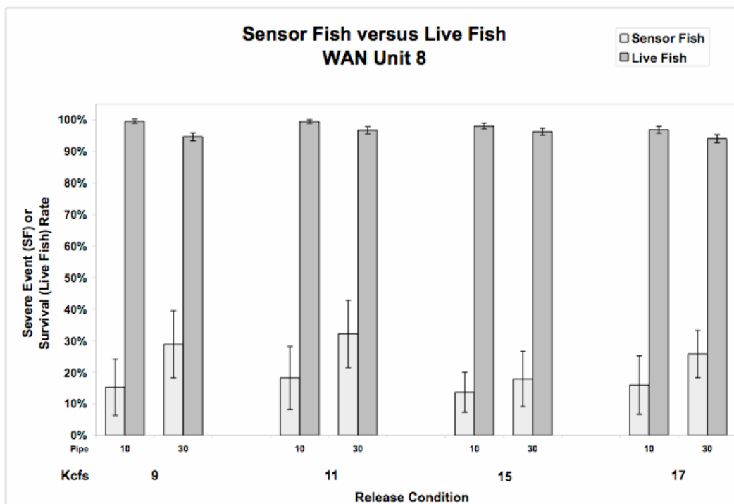
Figure 4.21. Comparison of Sensor Fish Severe Event (collision and shear) and Live Fish Survival Rates (and standard error) for Unit 8 (AHT) across Discharge (kcfs) and Release Pipe (10 and 30 ft)
