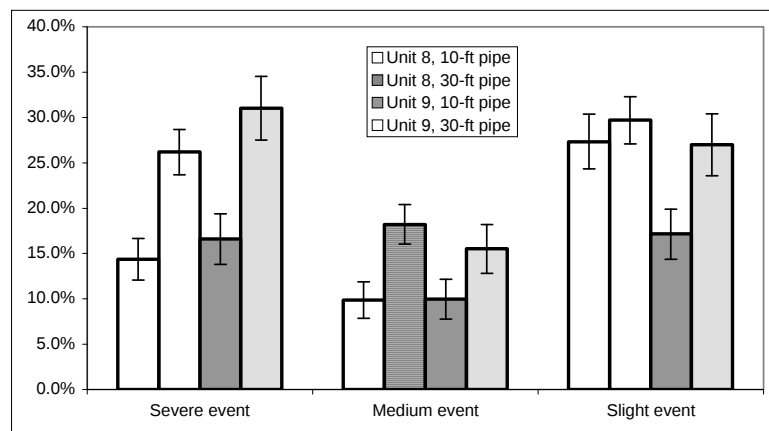
Figure 4.13. Comparison of Probabilities of Significant Events by Different Release Pipe Elevations. All regions and discharges were combined.
