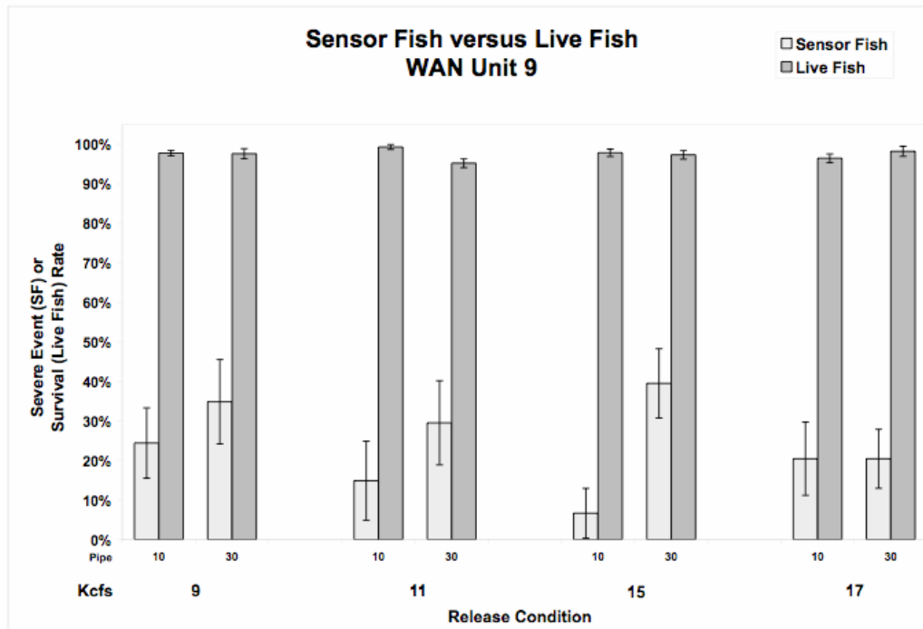
Figure 4.20. Comparison of Sensor Fish Severe Event (collision and shear) and Live Fish Survival Rates (and standard error) for Unit 9 (existing) across Discharge (kcfs) and Release Pipe (10 and 30 ft)
